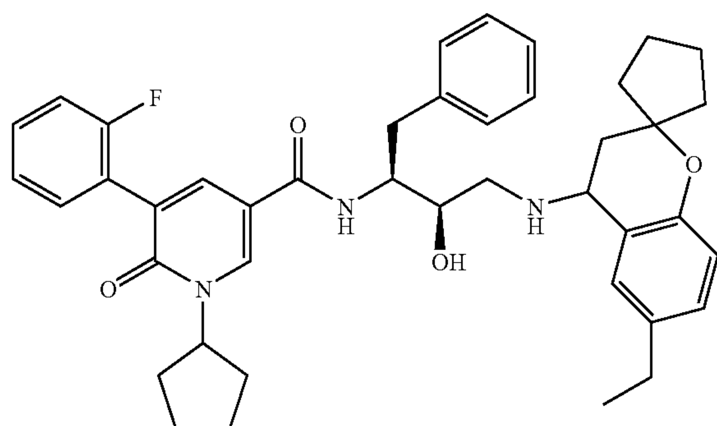
1-cyclopentyl-N-((2S,3R)-4-(6-ethyl-2,2-spirocyclopentylchroman-4-ylamino)-3-hydroxy-1-phenylbutan-2-yl)-5-(2-fluorophenyl)-6-oxo-1,6-dihydropyridine-3-carboxamide
