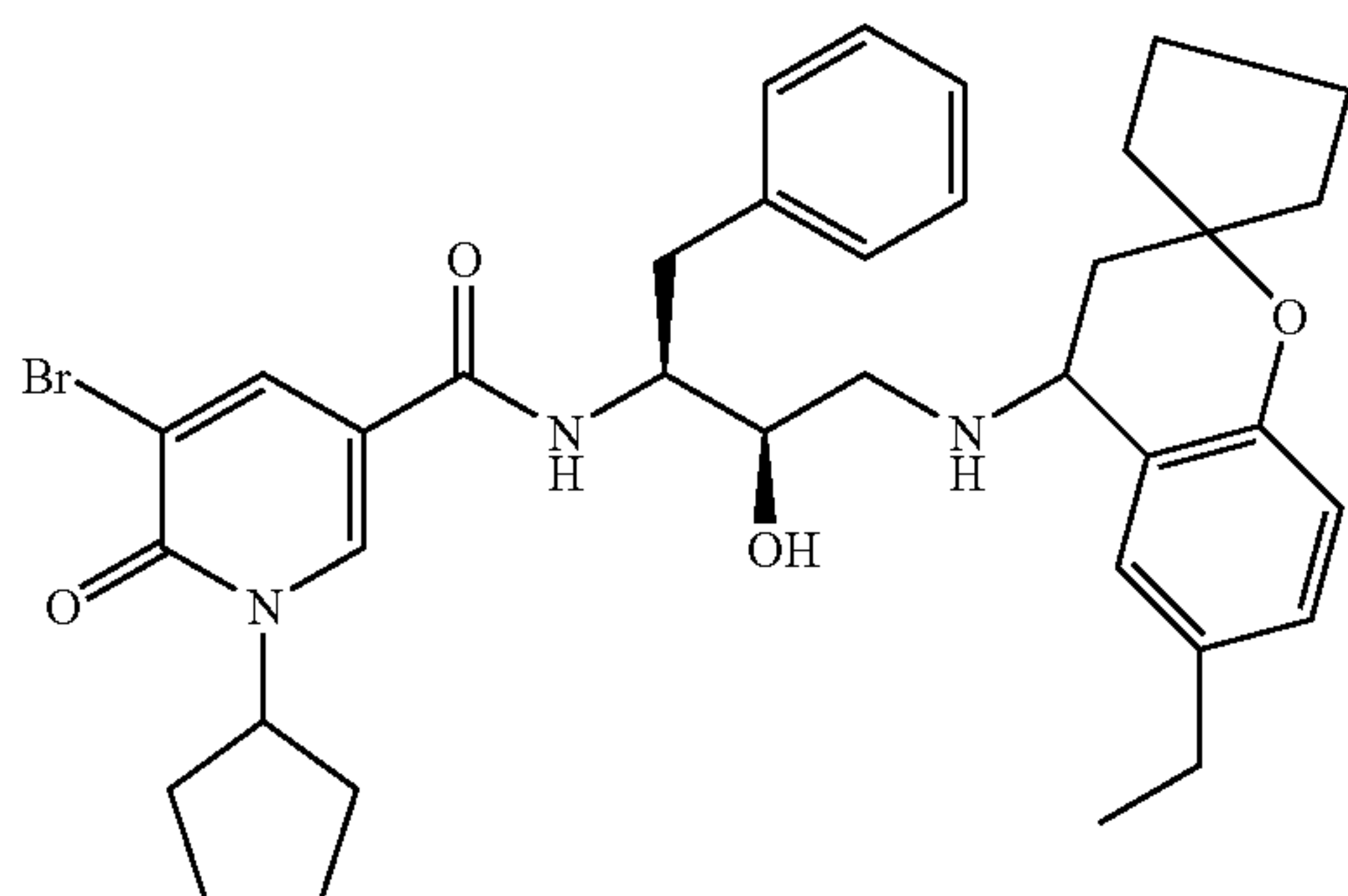
5-Bromo-1-cyclopentyl-N-((2S,3R)-4-(6-ethyl-2,2-spirocyclopentylchroman-4-ylamino)-3-hydroxy-1-phenylbutan-2-yl)-6-oxo-1,6-dihydropyridine-3-carboxamide
