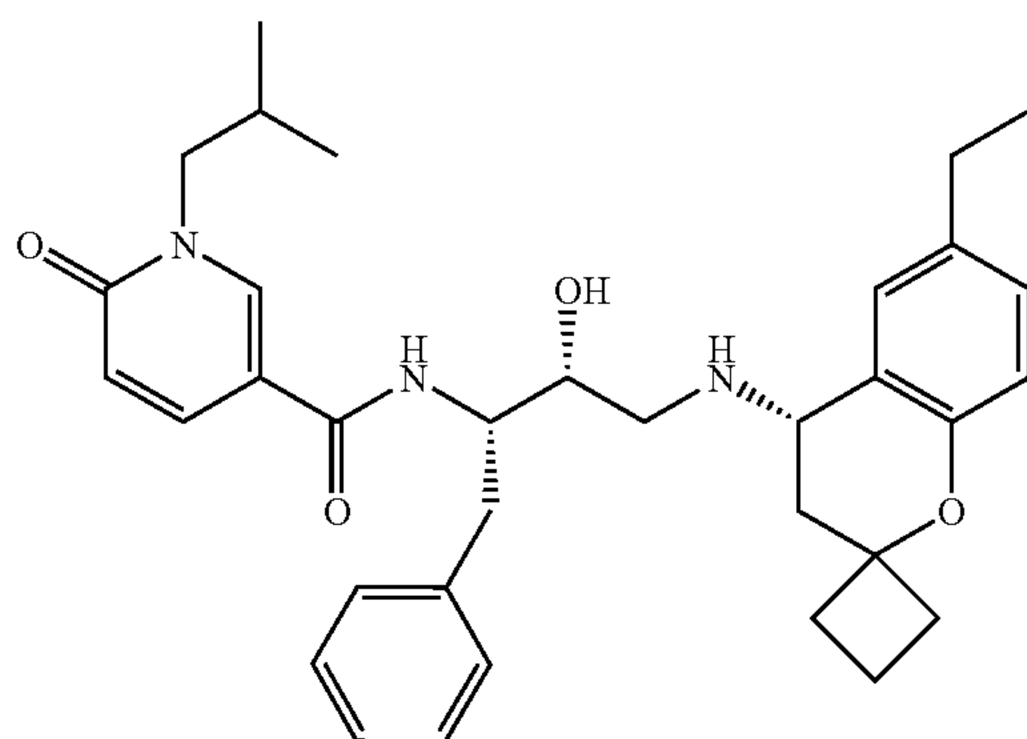
1-Isobutyl-N((2S,3R)-4-((S)-6-ethyl-2,2-spirocyclobutylchroman-4-ylamino))-3-hydroxy-1-phenylbutan-2-yl)-6-oxo-1,6-dihydropyridine-3-carboxamide.TFA salt
