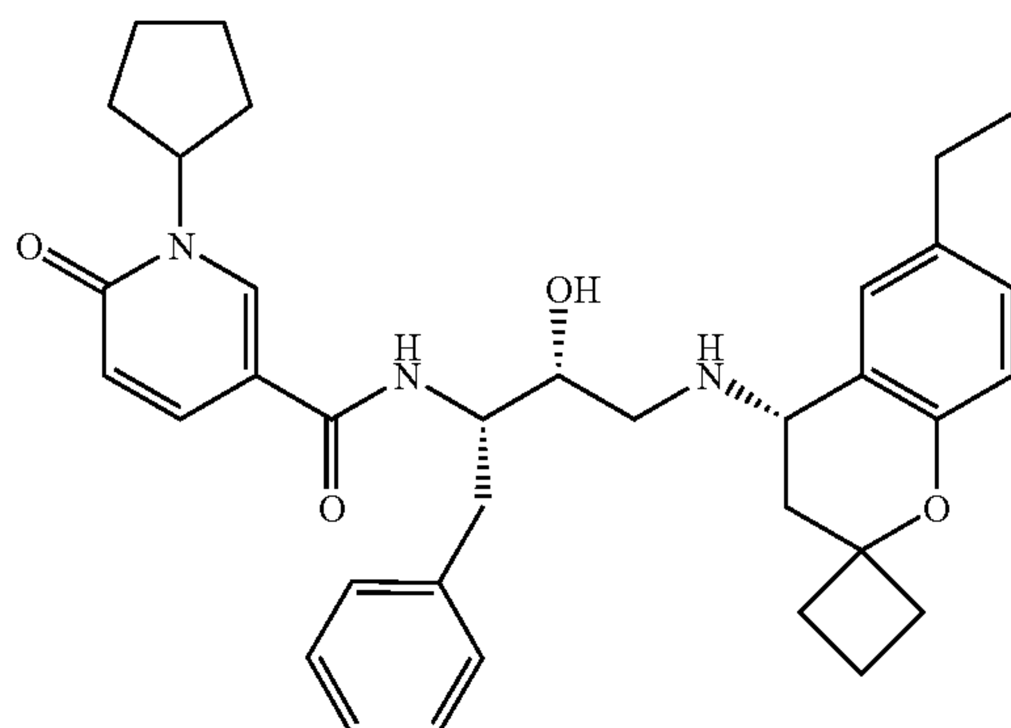
1-Cyclopentyl-N((2S,3R)-4-((S)-6-ethyl-2,2-spirocyclobutylchroman-4-ylamino))-3-hydroxy-1-phenylbutan-2-yl)-6-oxo-1,6-dihydropyridine-3-carboxamide.TFA salt
