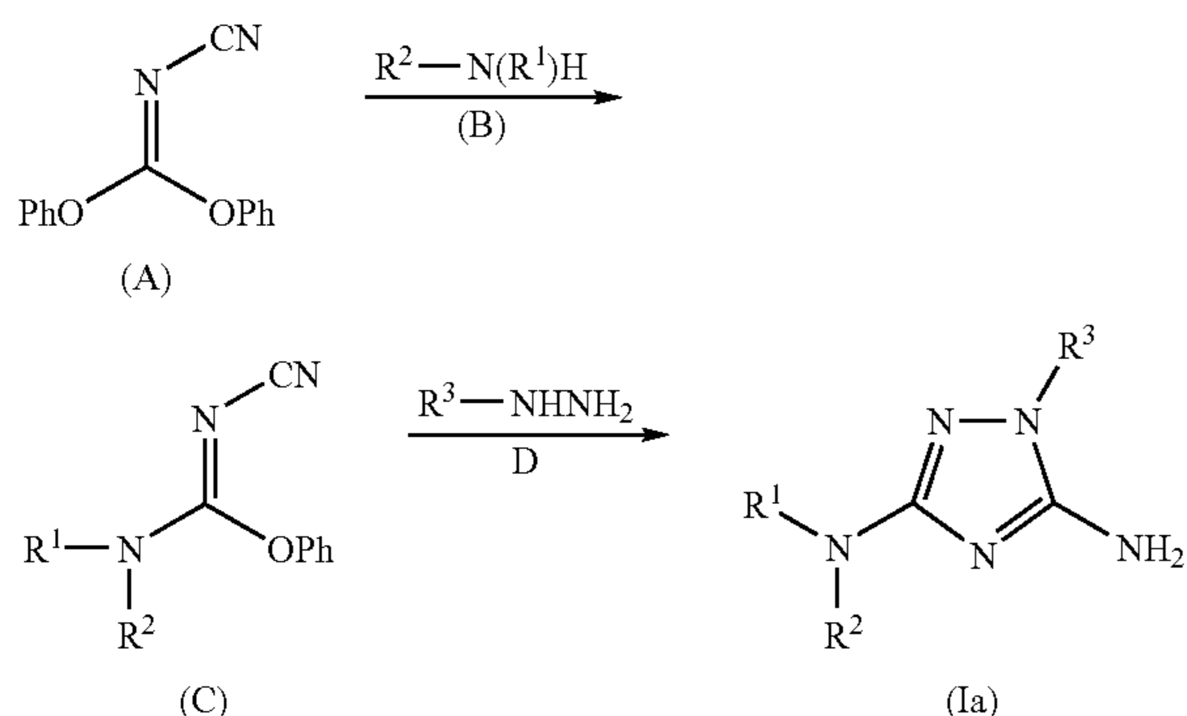
REACTION SCHEME 1
