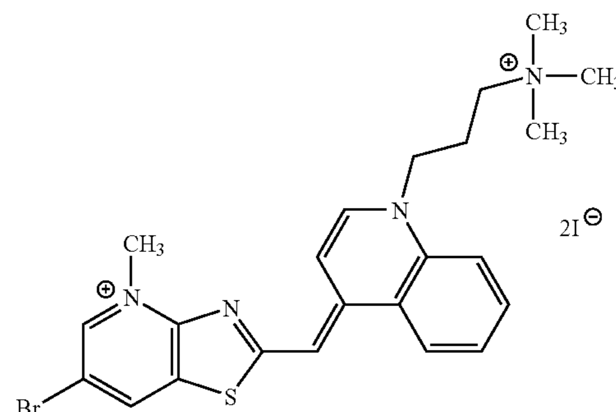
Compound 47
