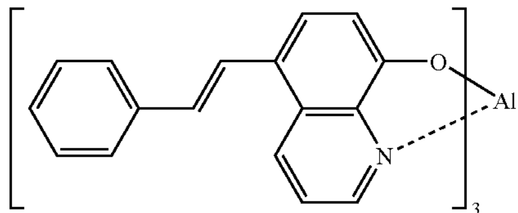
Compound described in JP-A 9-255686
