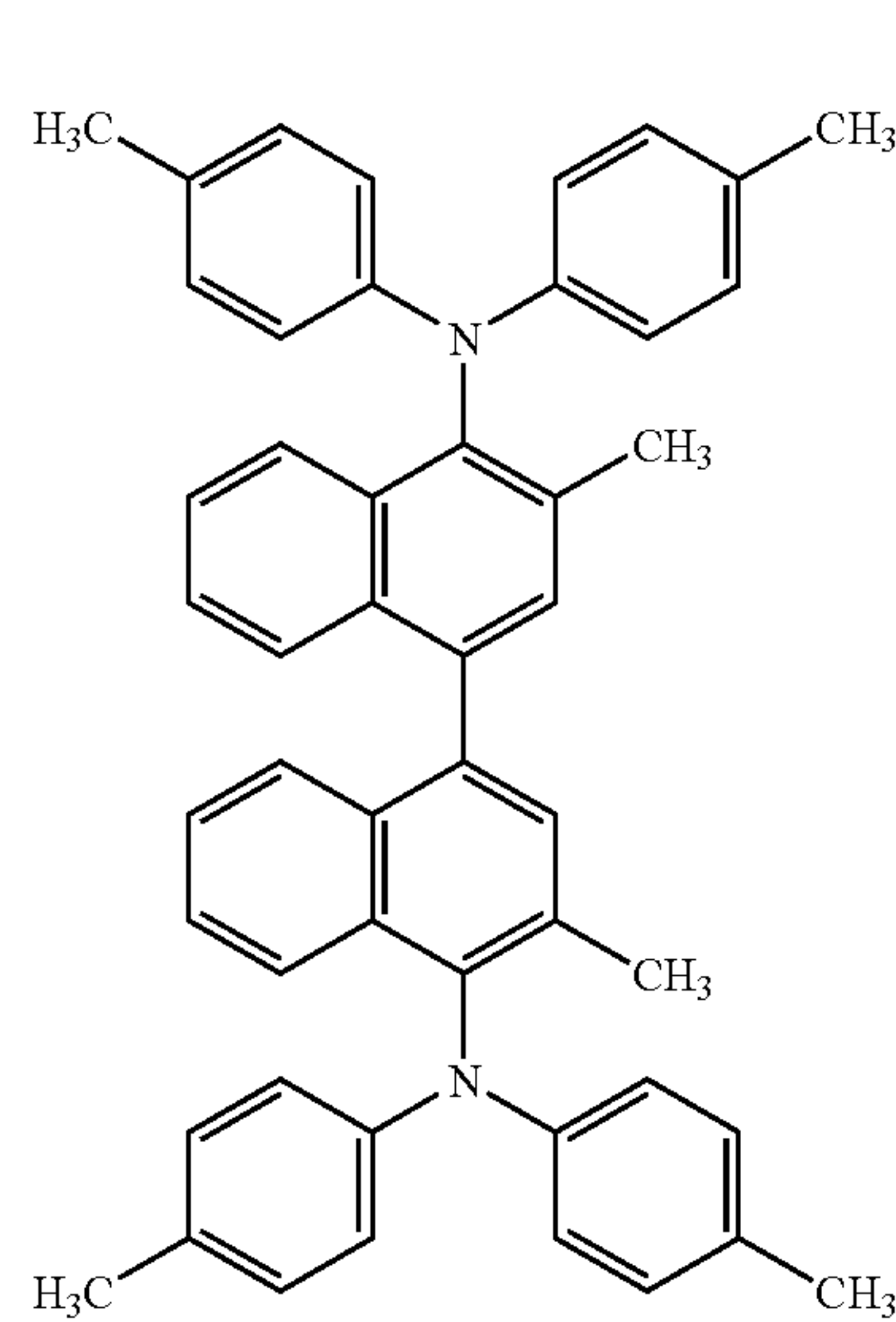
Compound described in JP-A 11-152253
