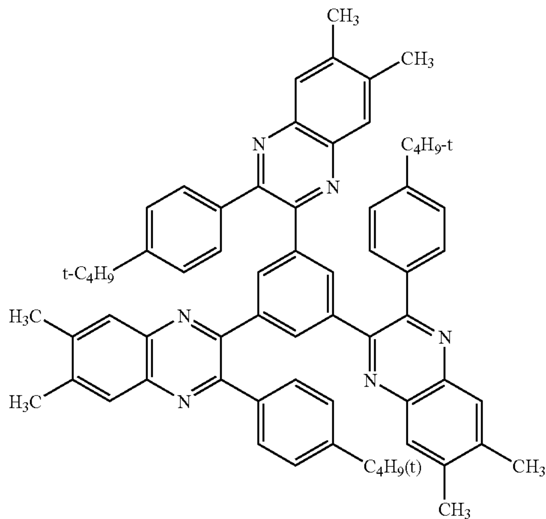
Compound described in Macromolecules 31, 6434 (1989)
