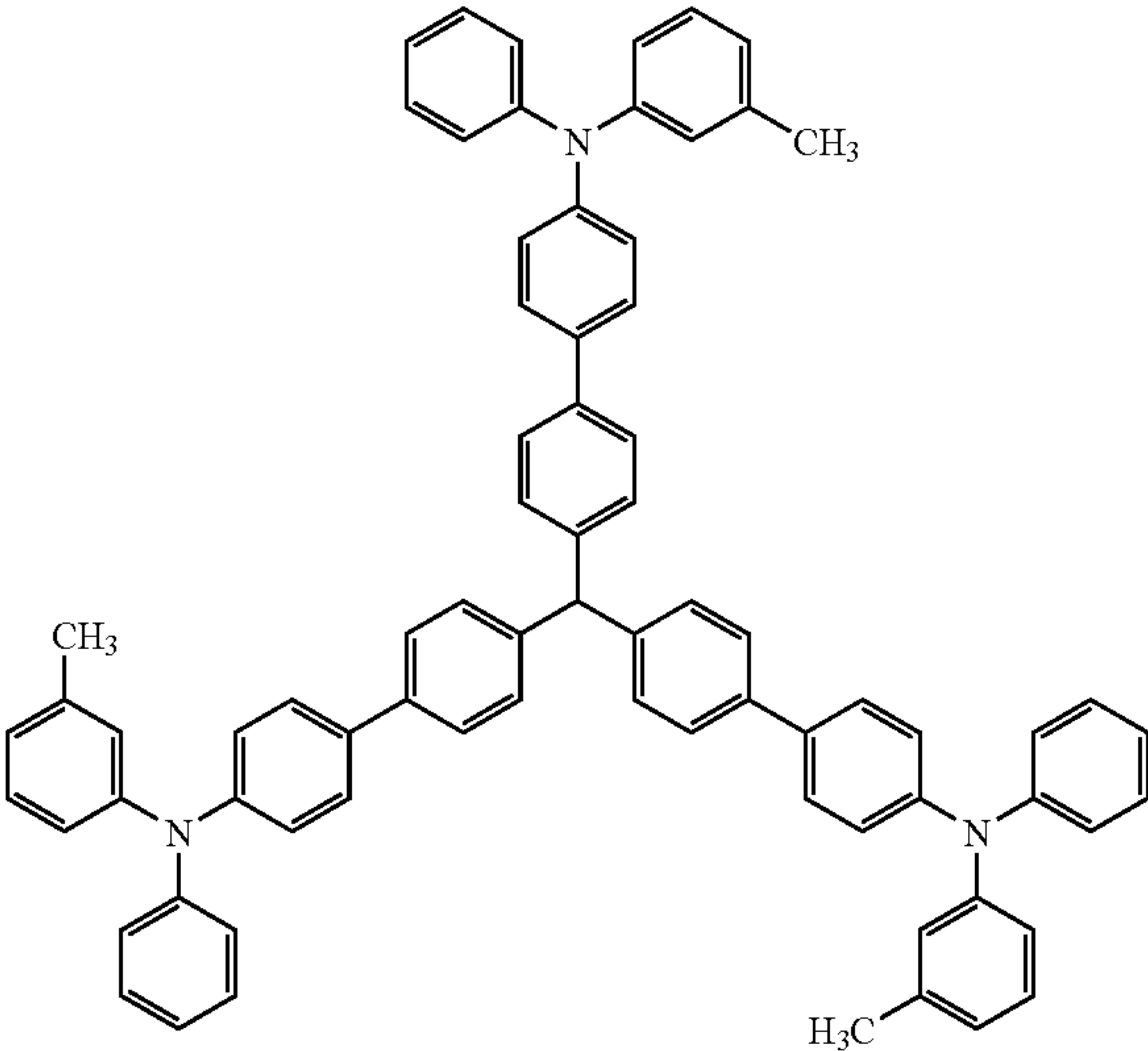
Compound described in JP-A 10-312073
