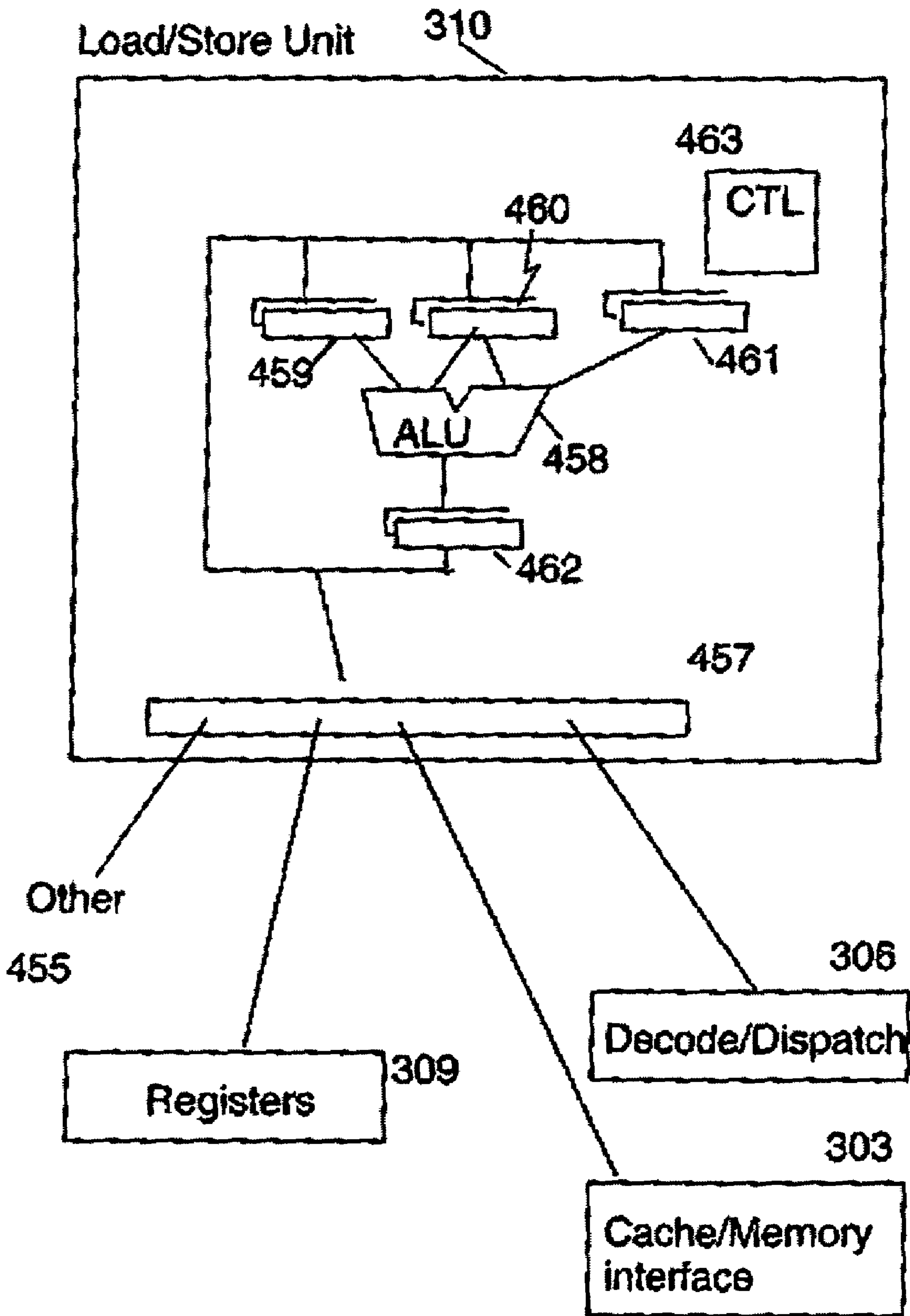
FIG. 4C Prior Art
