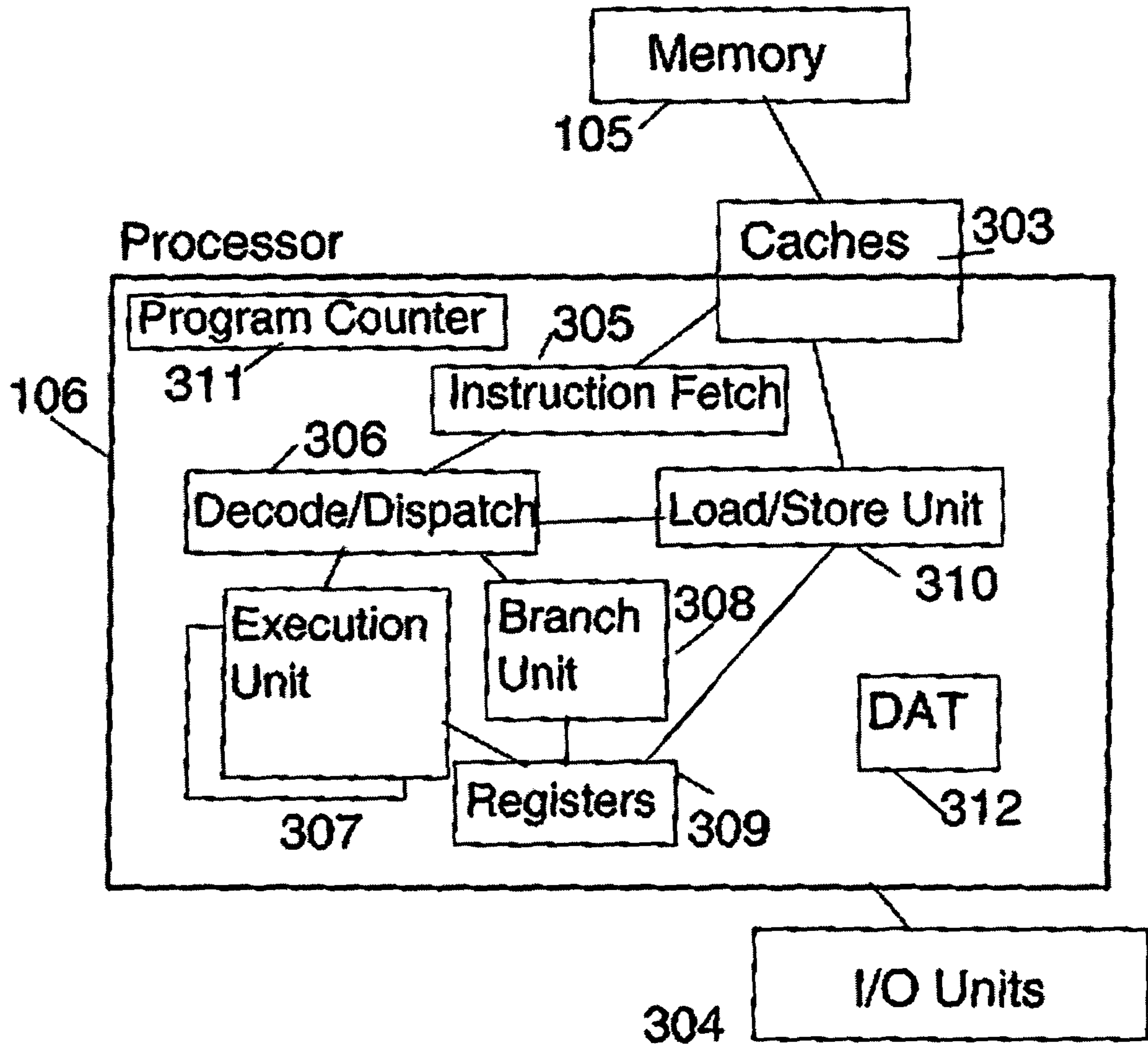
FIG. 3 Prior Art
