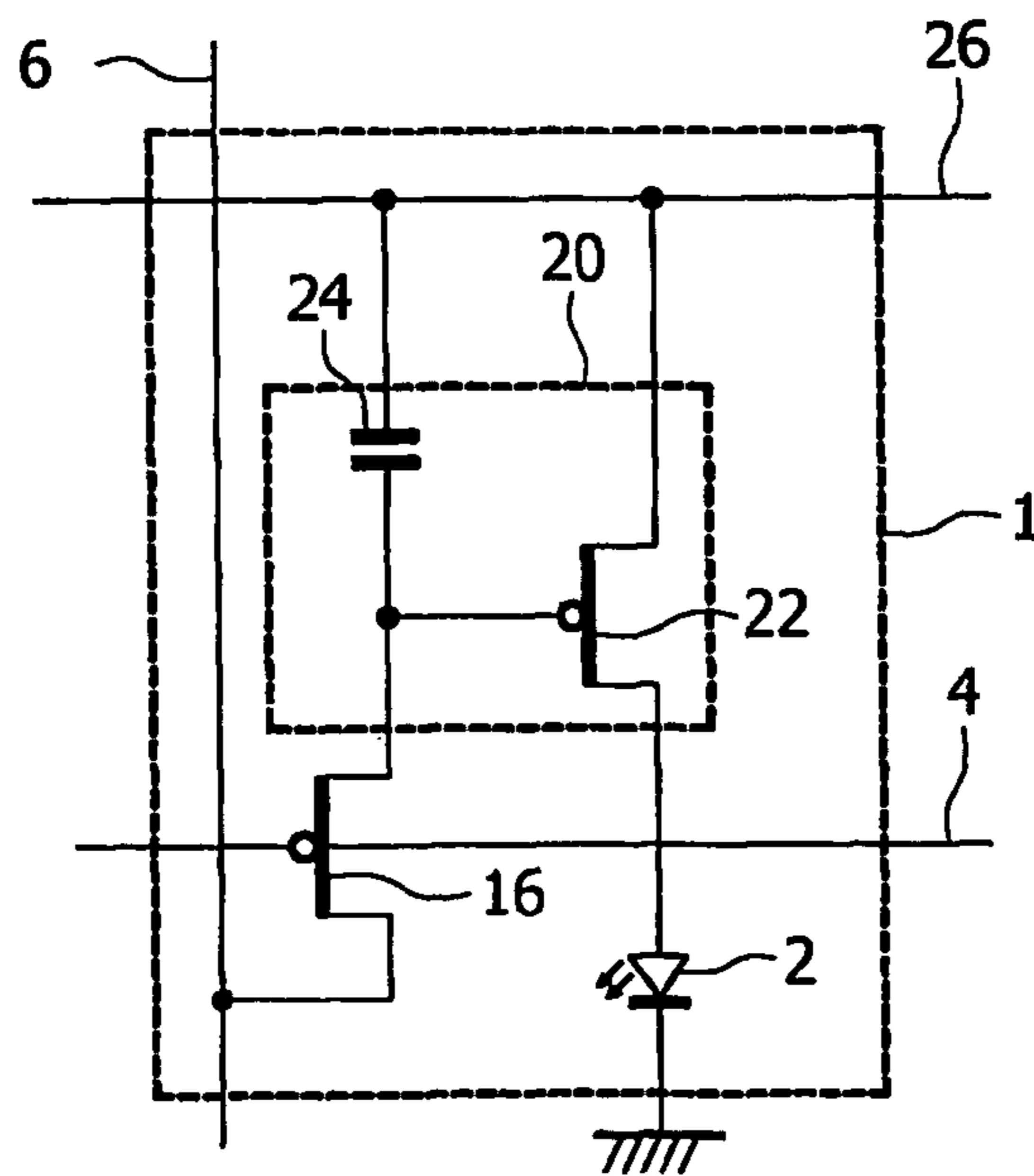
FIG. 2 PRIOR ART
