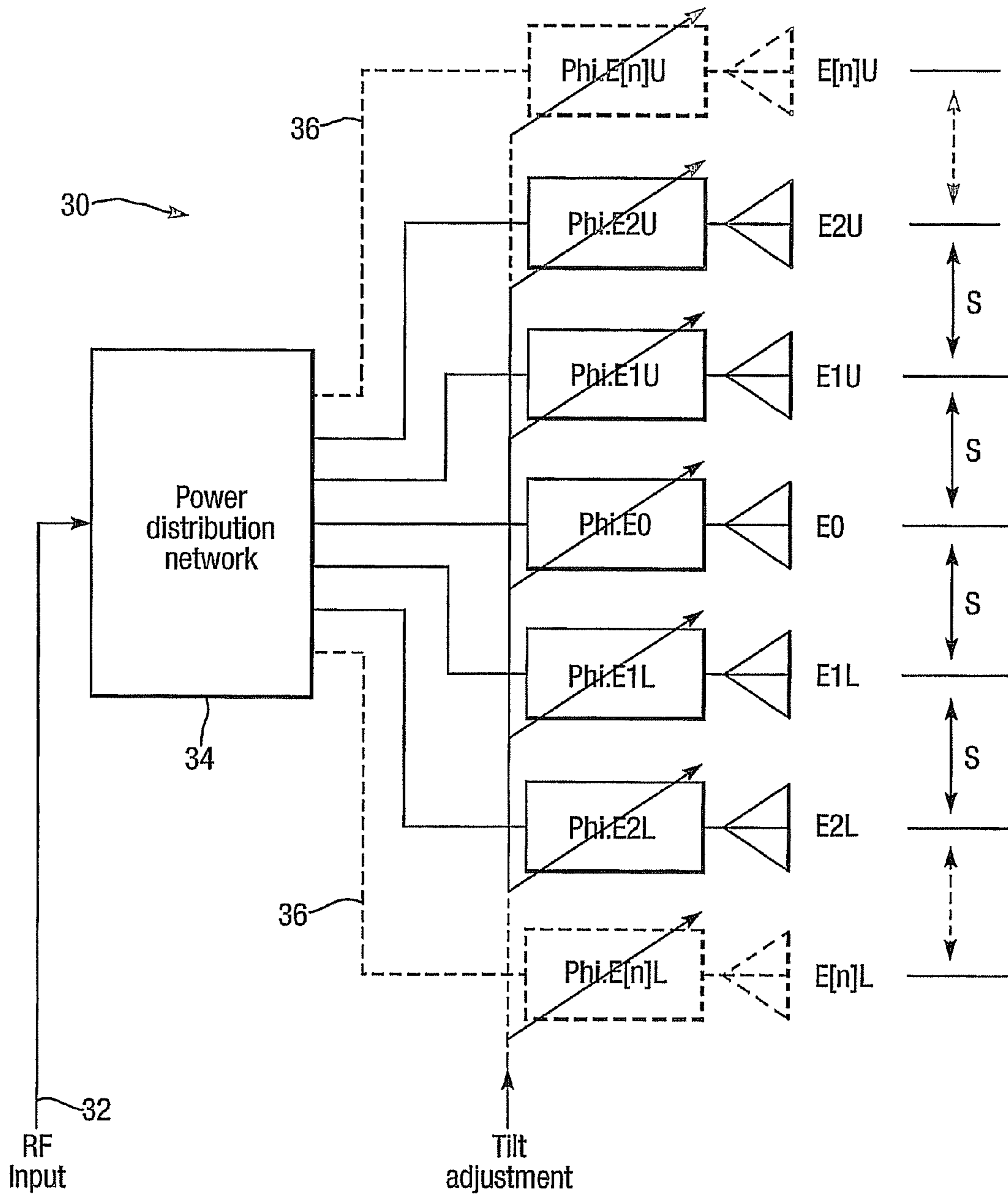
Fig.2. (Prior art)
