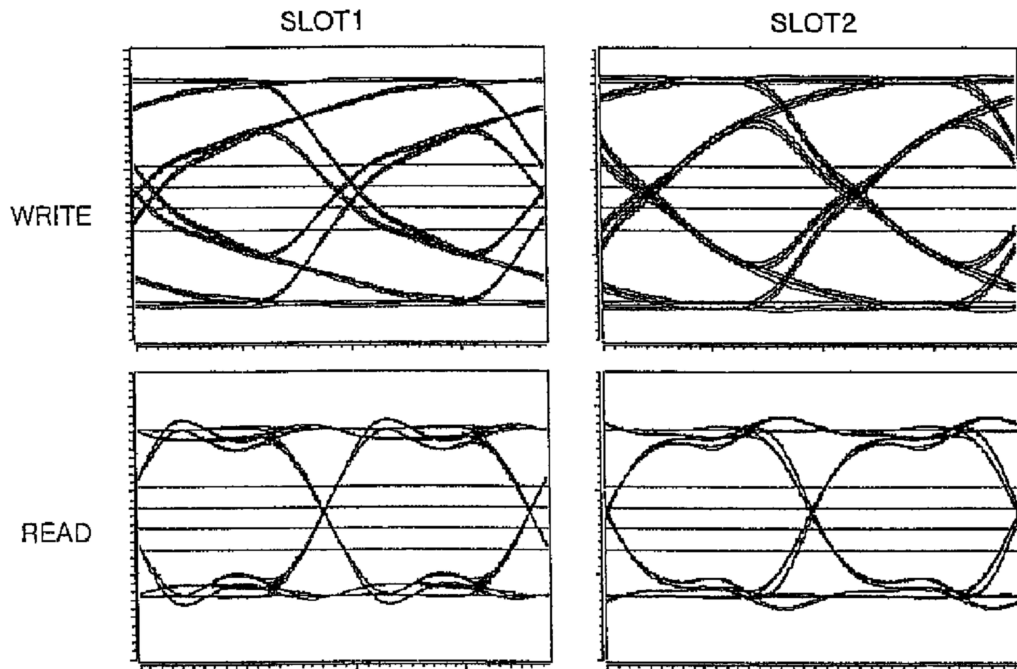
FIG. 3 Prior Art
