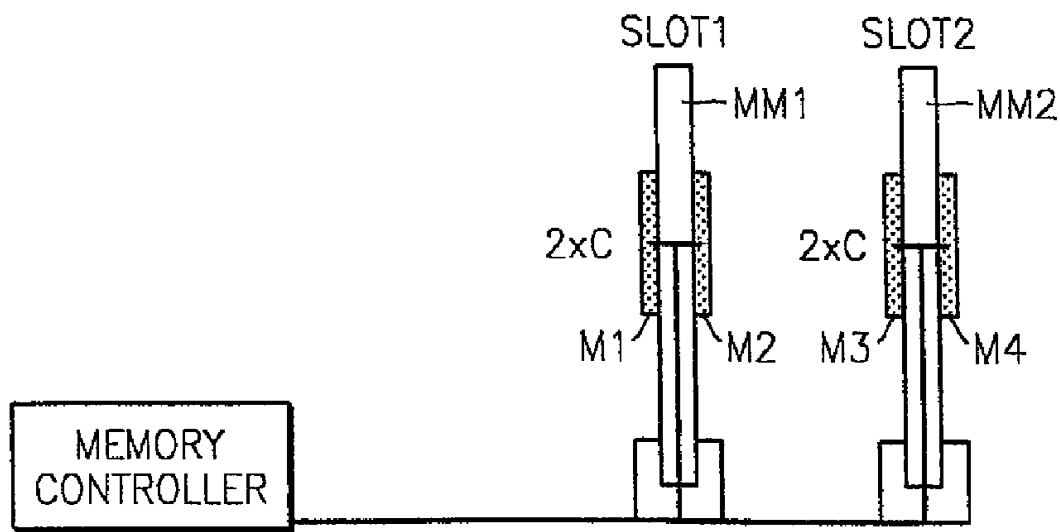
FIG. 4 Prior Art
