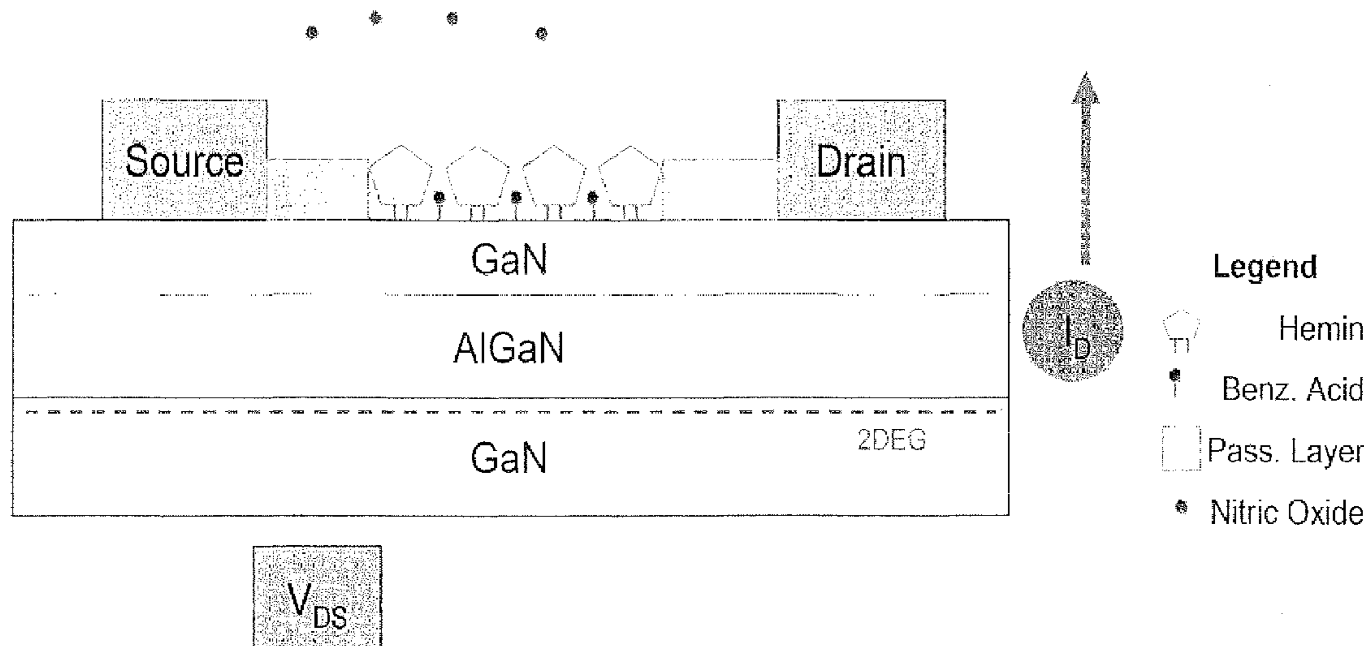
Schematic of Functionalized GaN-AlGaIn HFET
