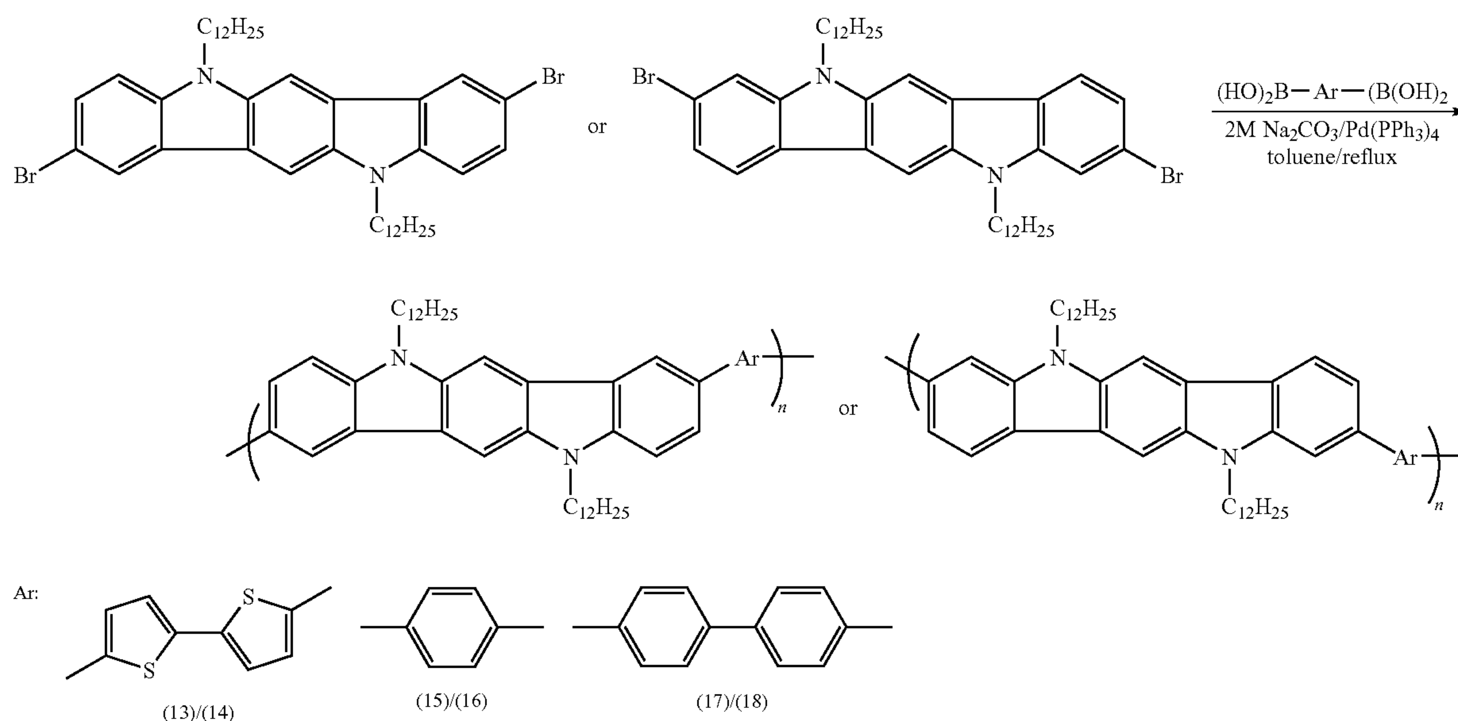
Scheme 2. Synthesis of polymer (13) through (18).
