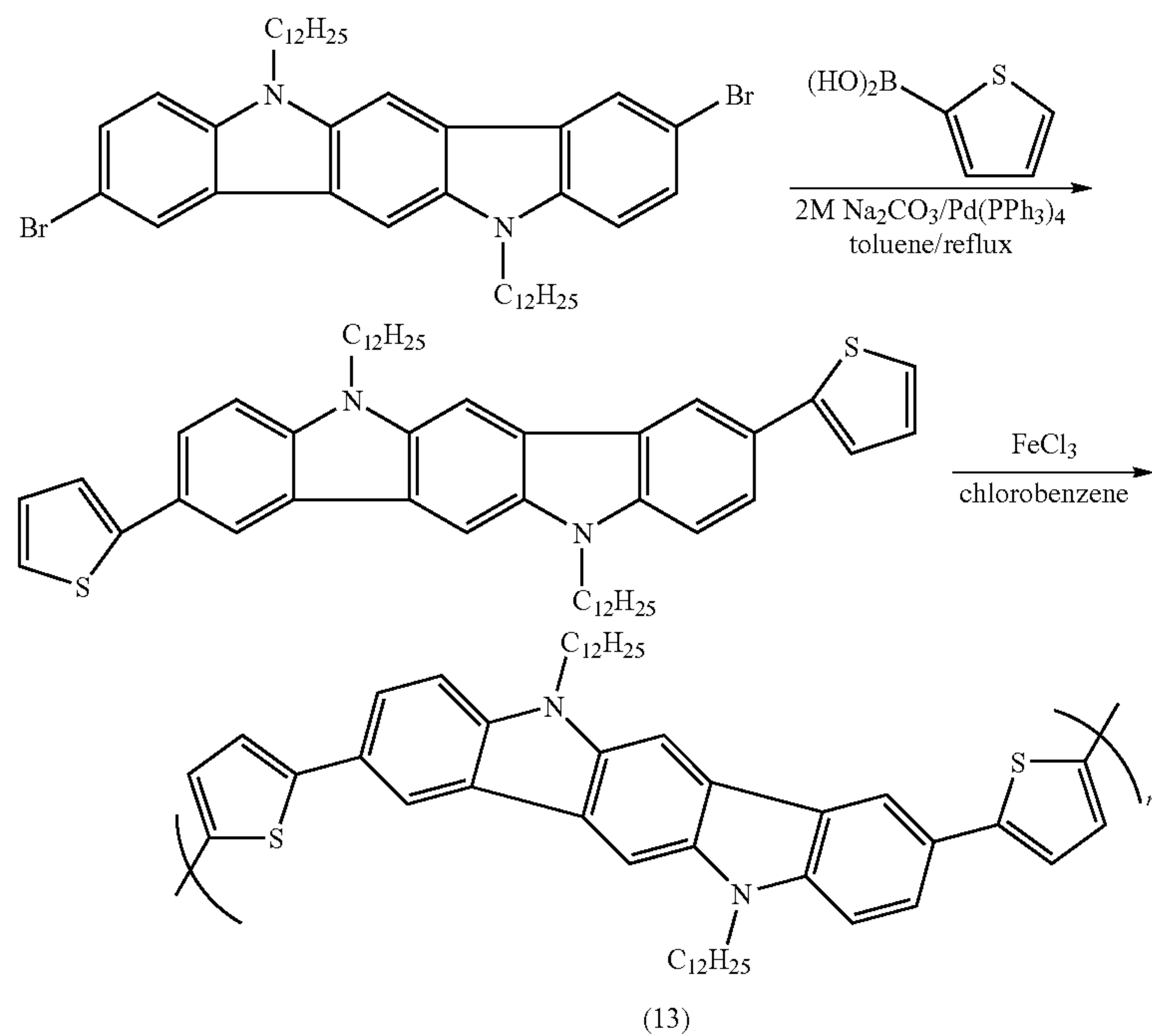
Scheme 3. Synthesis of polymer (13).
