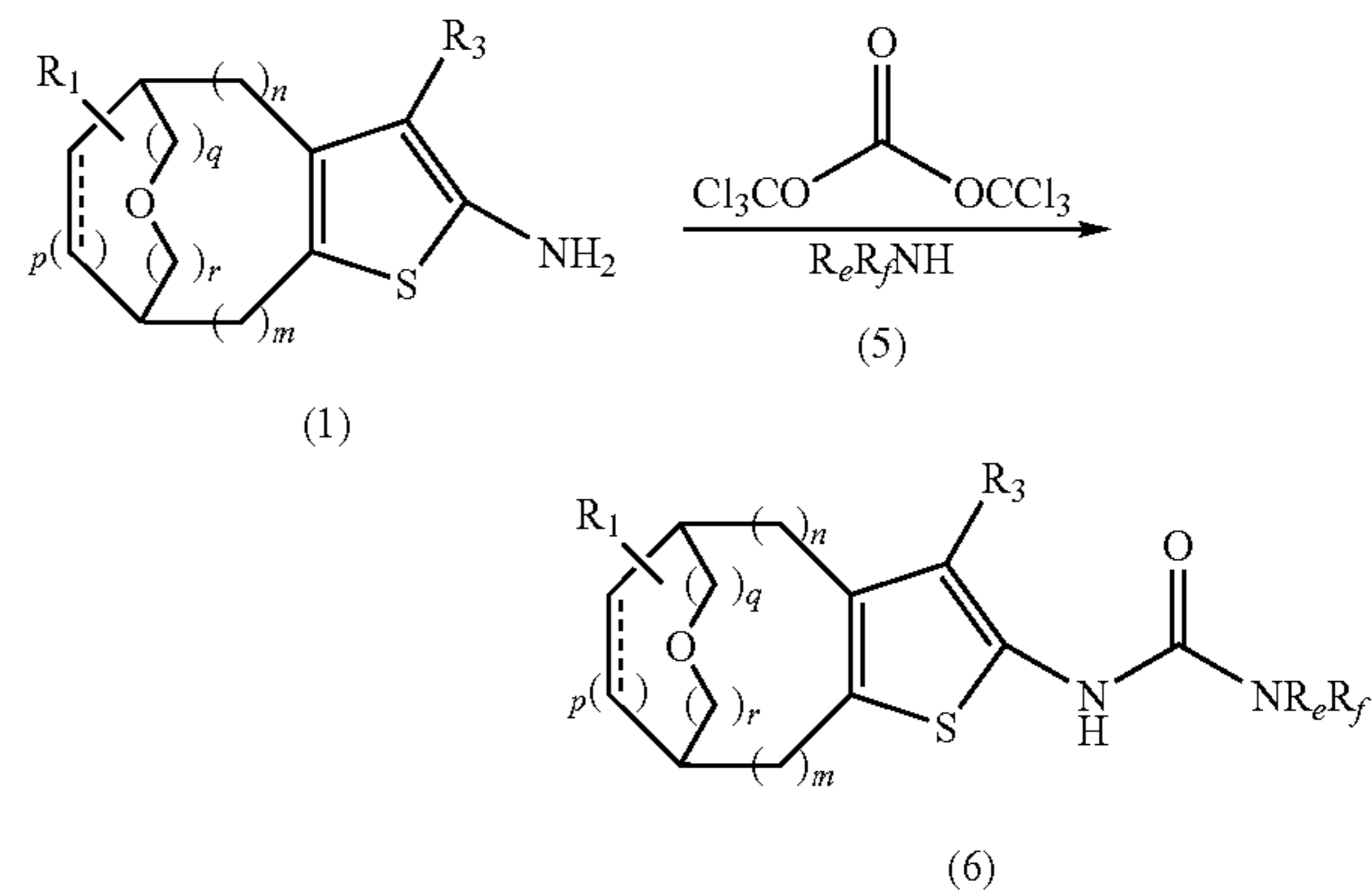
Scheme 2
