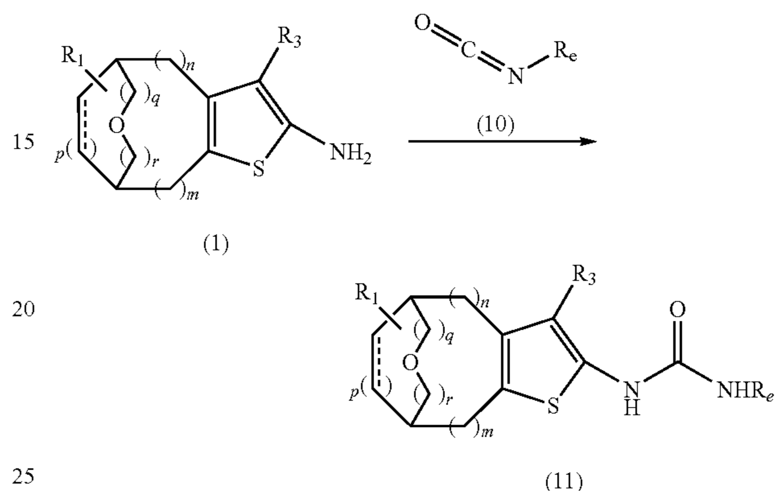
Scheme 5
