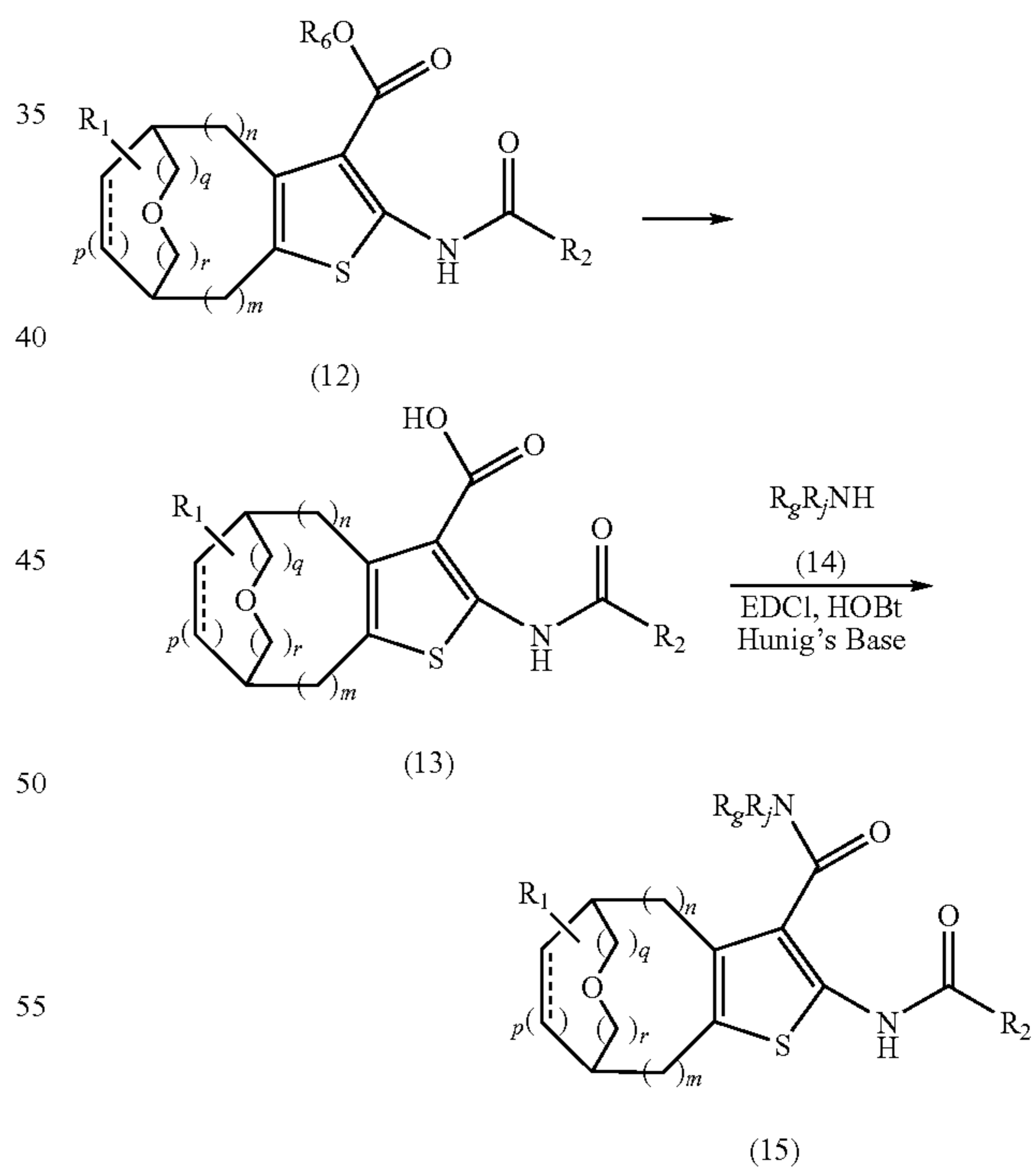
Scheme 6
