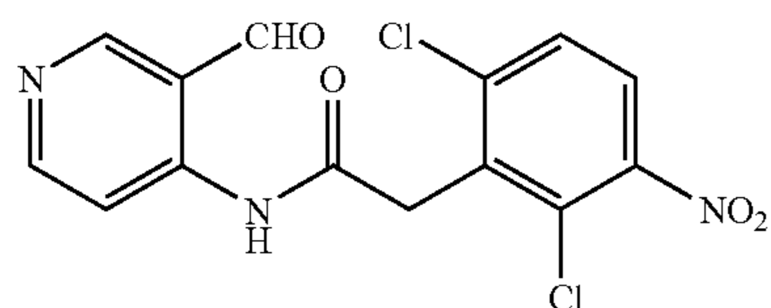
Scheme 3
