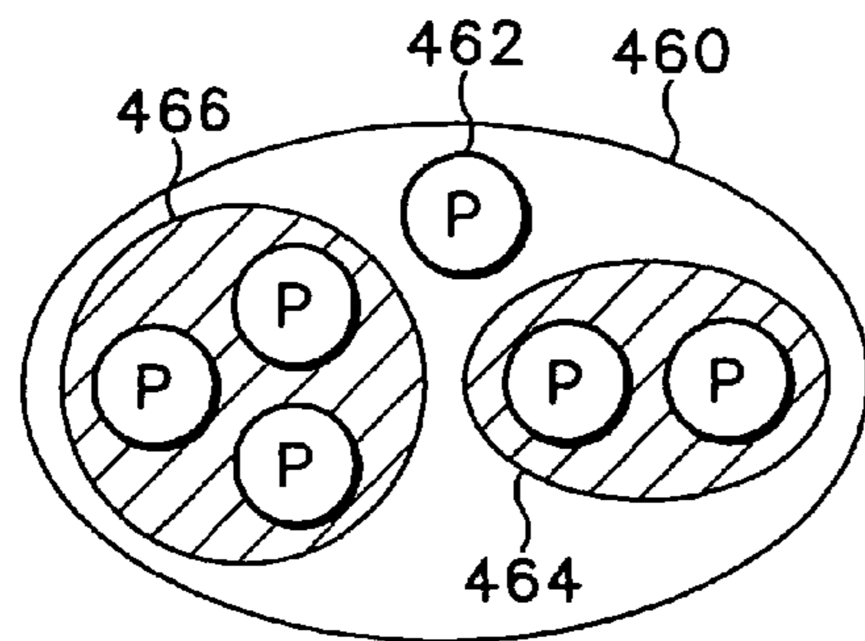
OBJECT HEIRARCHY
