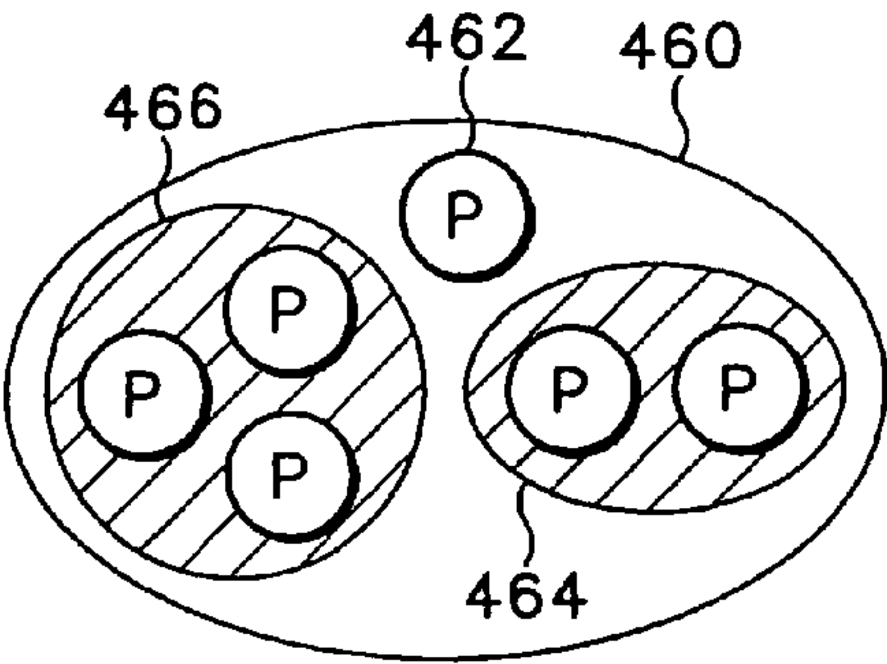
OBJECT HEIRARCHY
