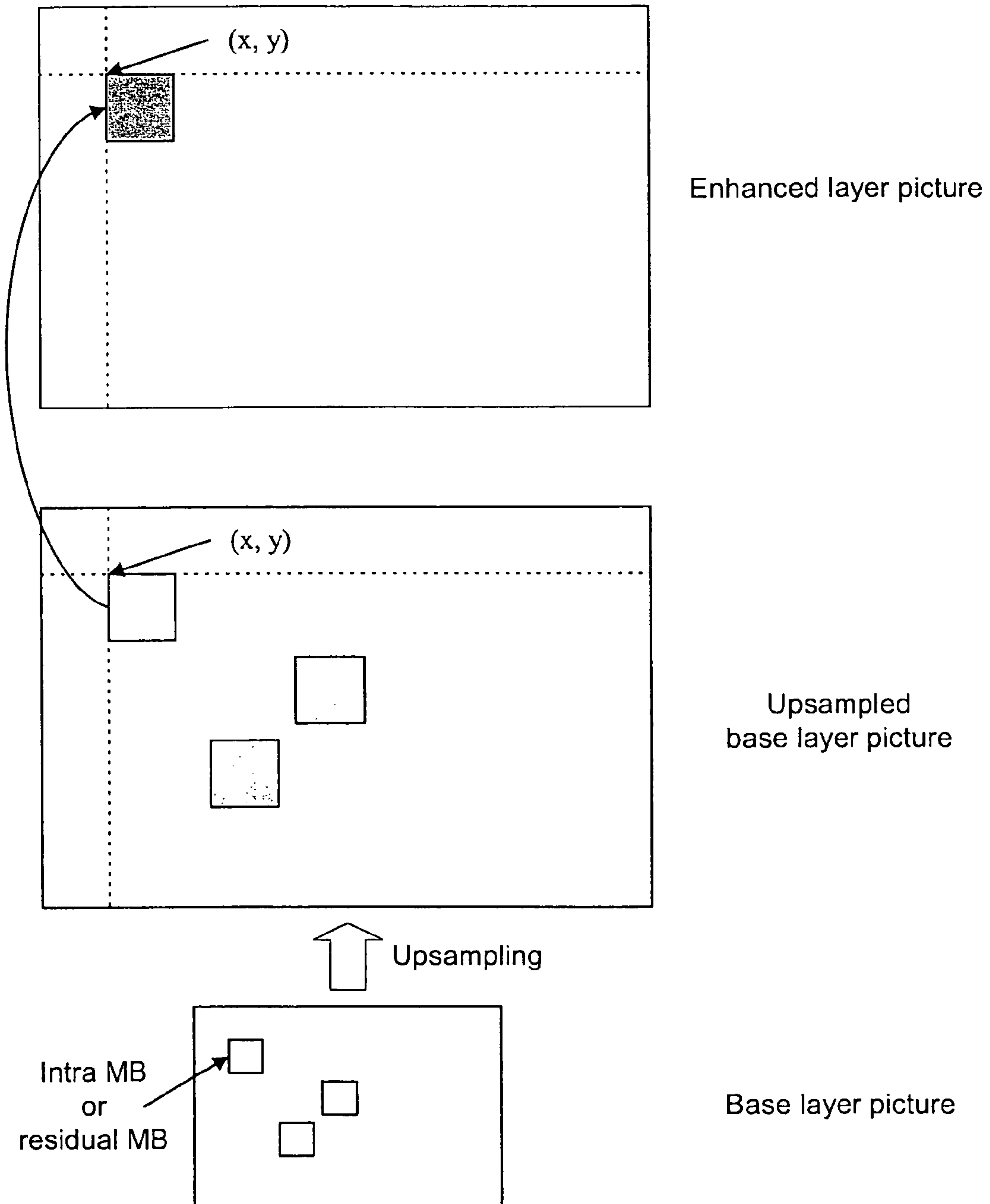
FIG. 1 (PRIOR ART)
