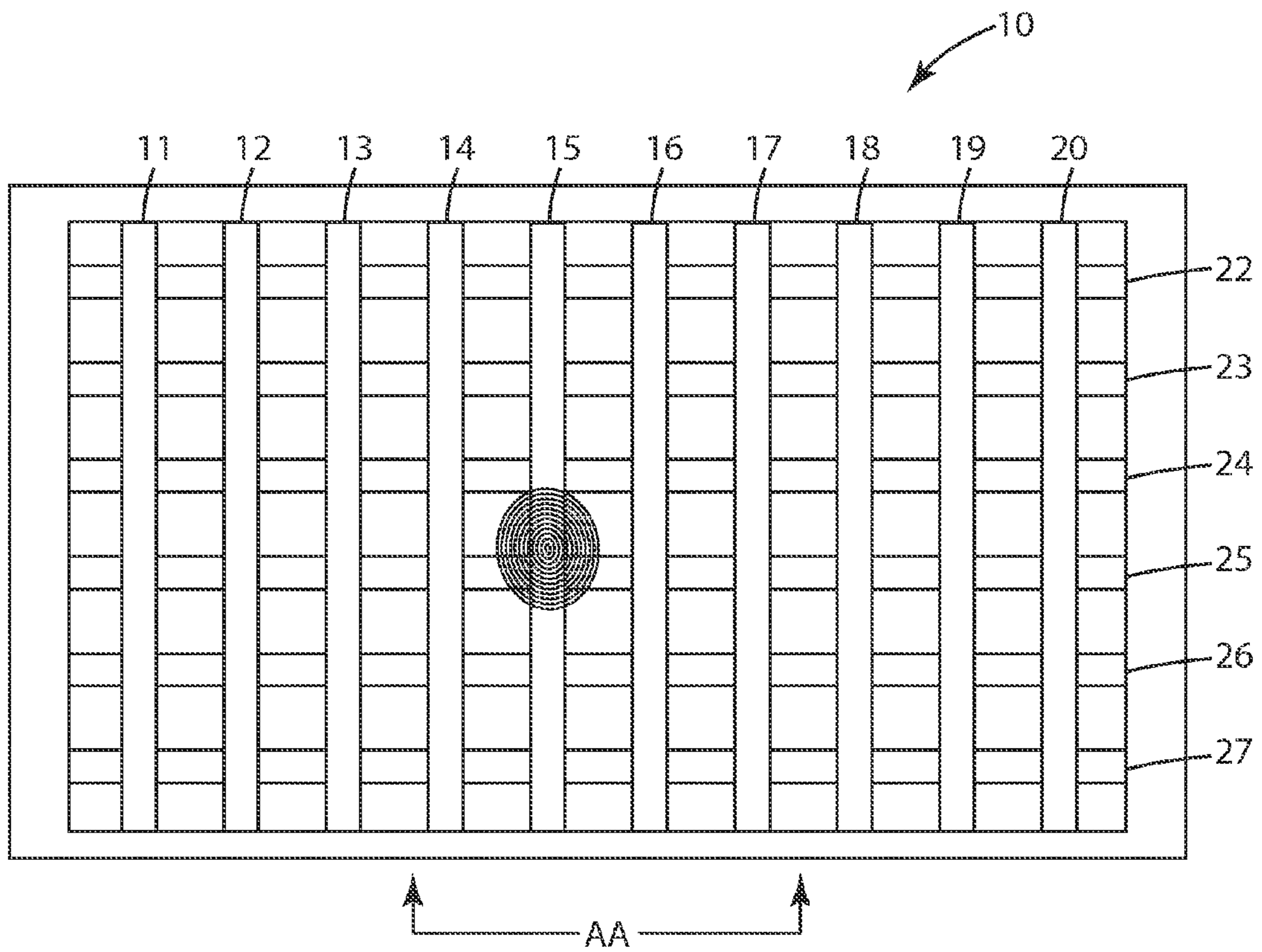
Fig. 1 Prior Art
