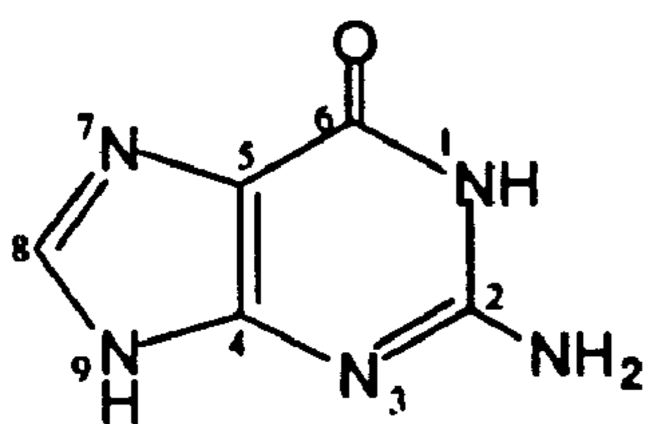
2-Amino-6-oxy-purine or Guanine
