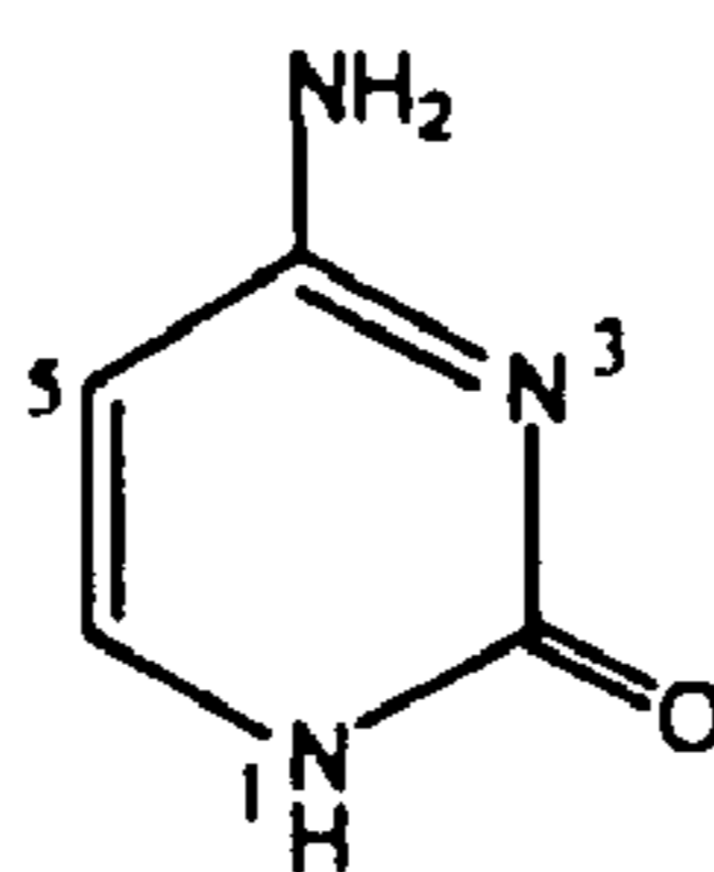
2-Oxy-4-amino pyrimidine or cytosine
