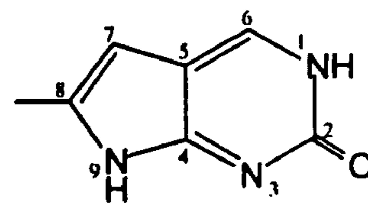
2-Oxy-7-deaza-8-methyl purine
