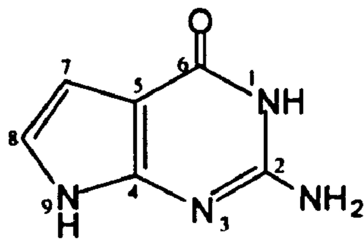
2-Amino-6-oxy-7-deaza-purine or 7-Deaza-guanine
