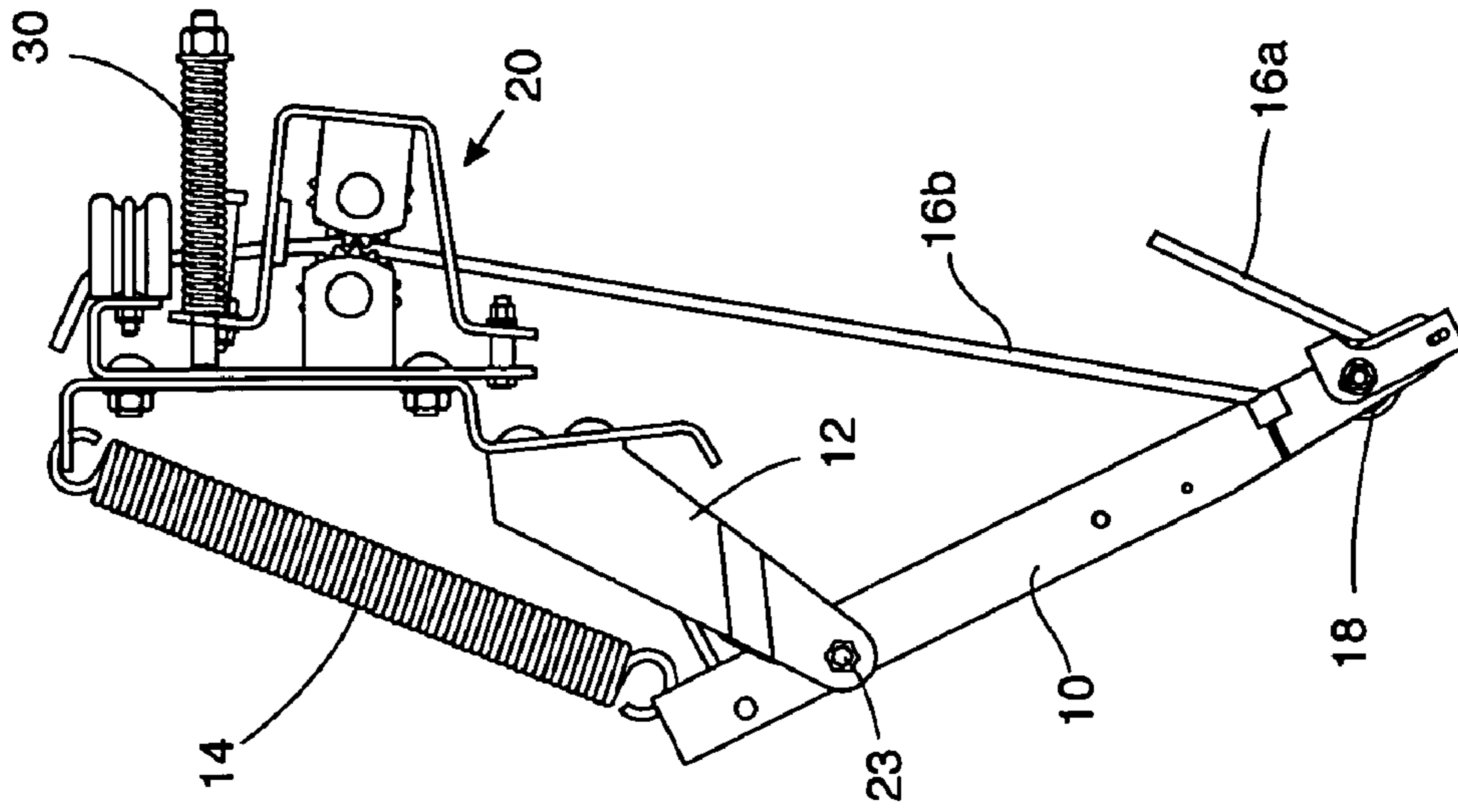
FIG. 2 (Prior Art)
