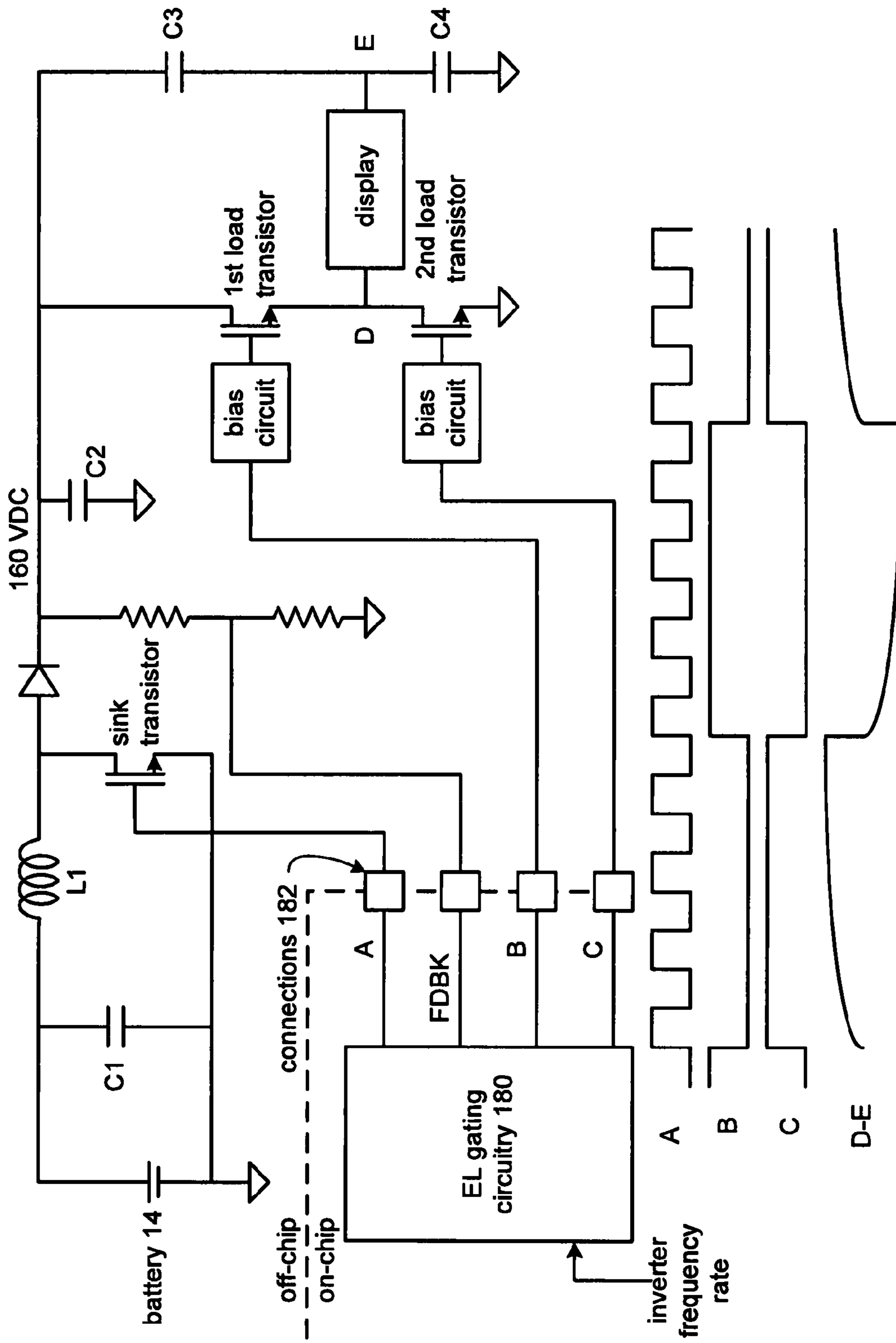
FIG. 8 EL backlighting drive circuitry 70
