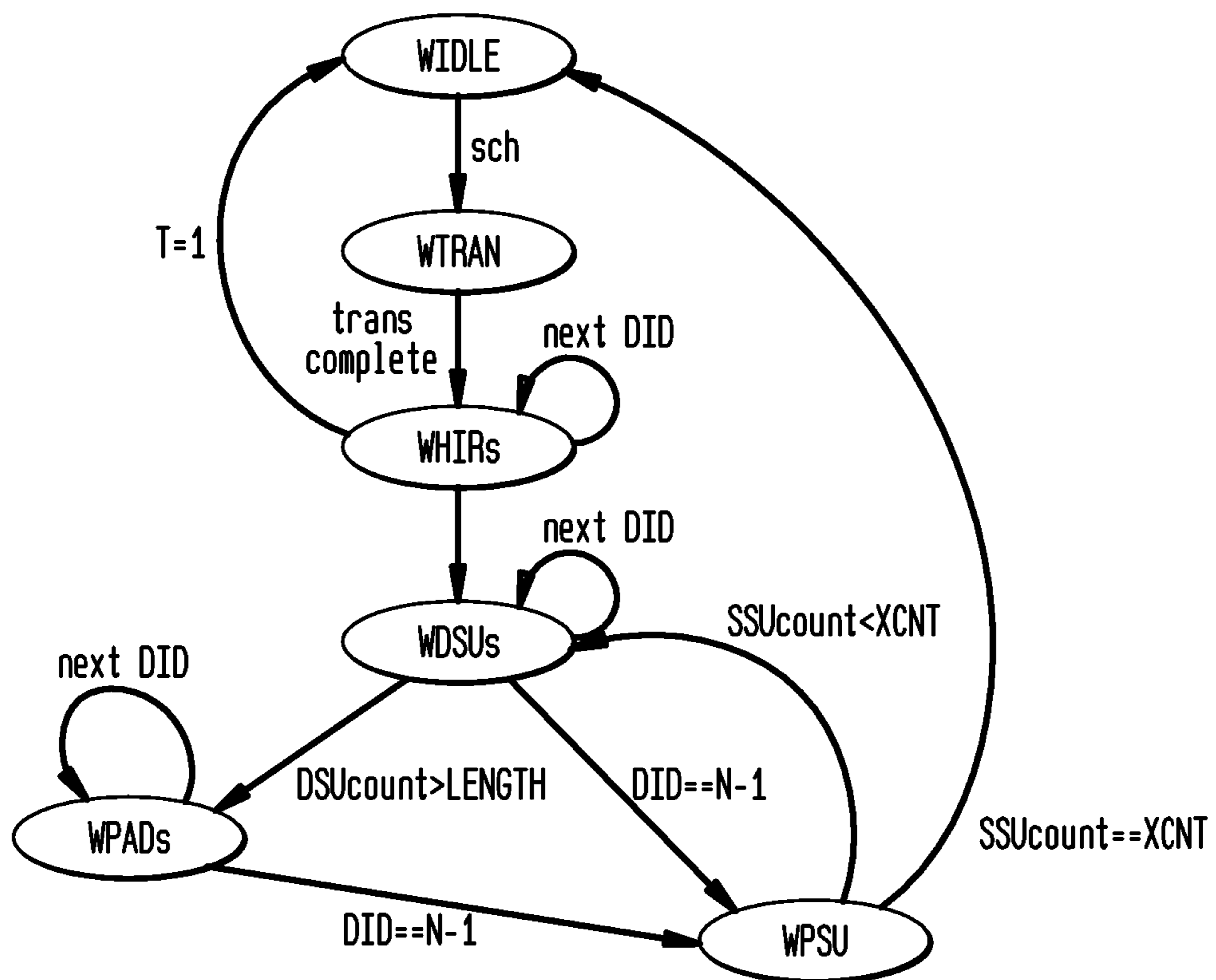
FIG. 24 WRITE OPERATION STATE MACHINE (WOSM) STATE DIAGRAM
