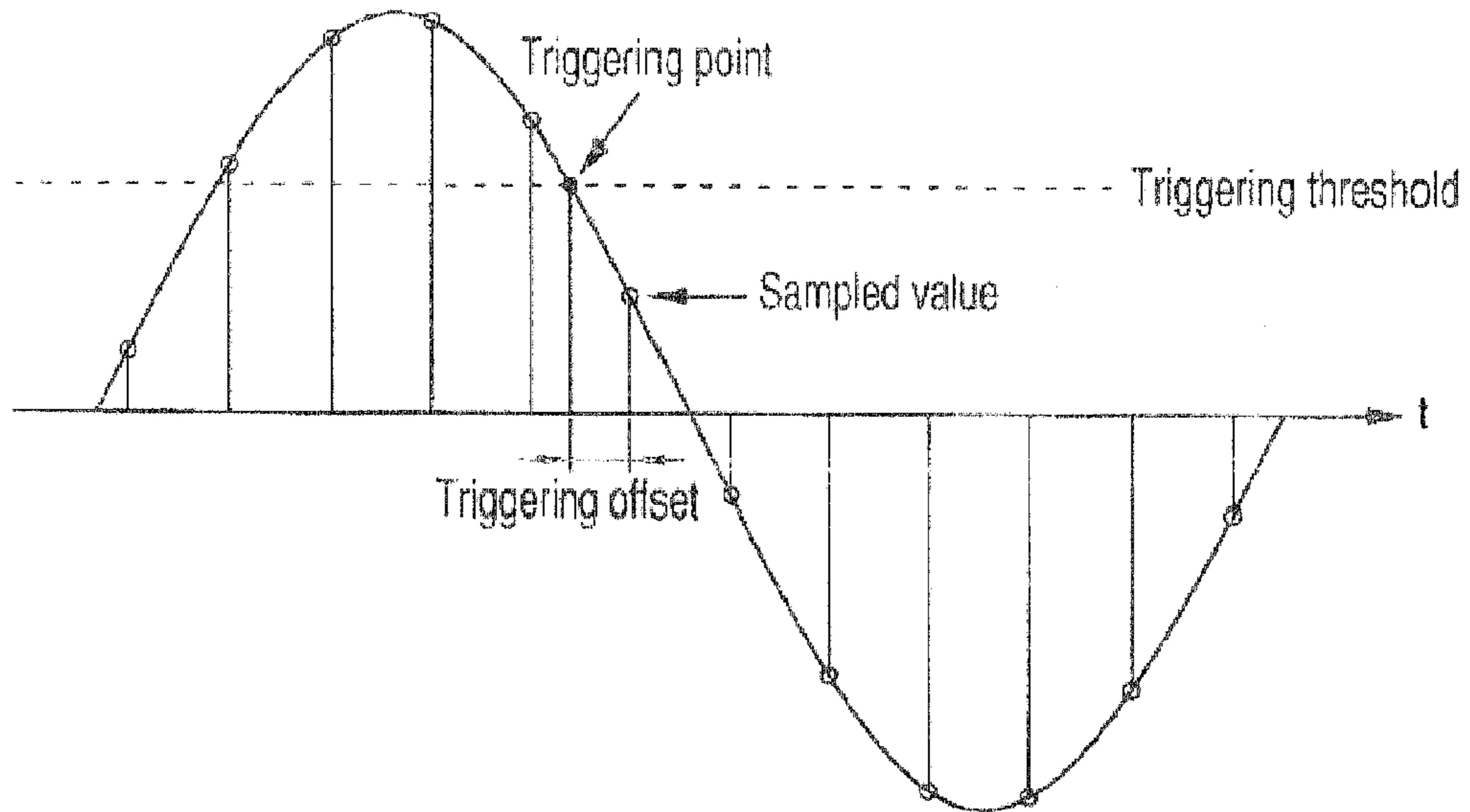
Fig. 3 (Prior art)
