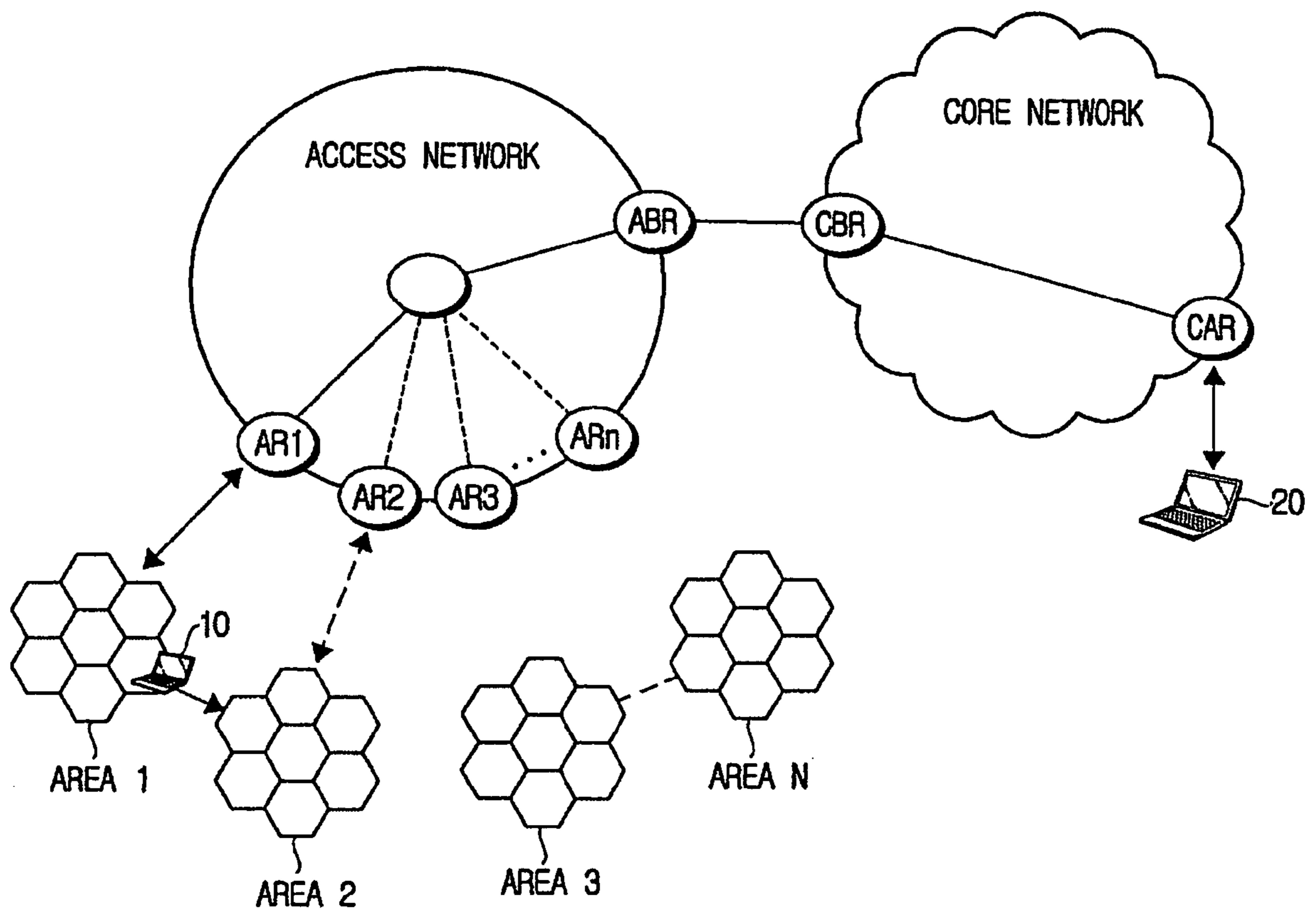
FIG. 3 (PRIOR ART)
