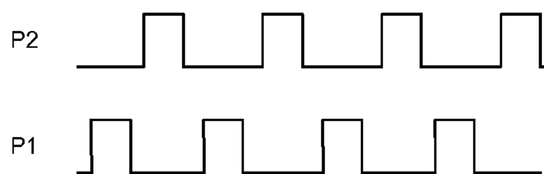
P1 AND P2 TIMING DIAGRAM
