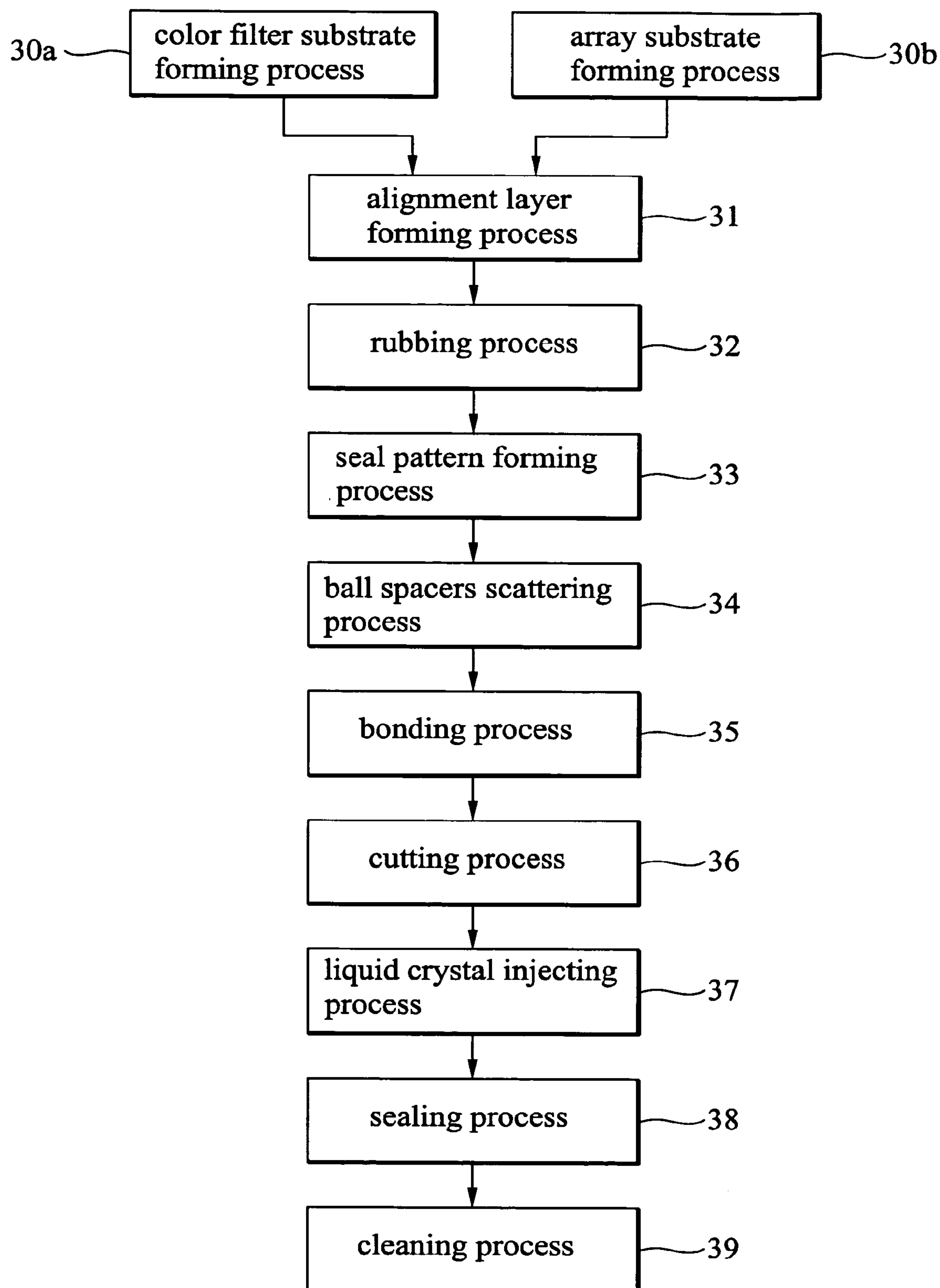
FIG. 3 ( RELATED ART )
