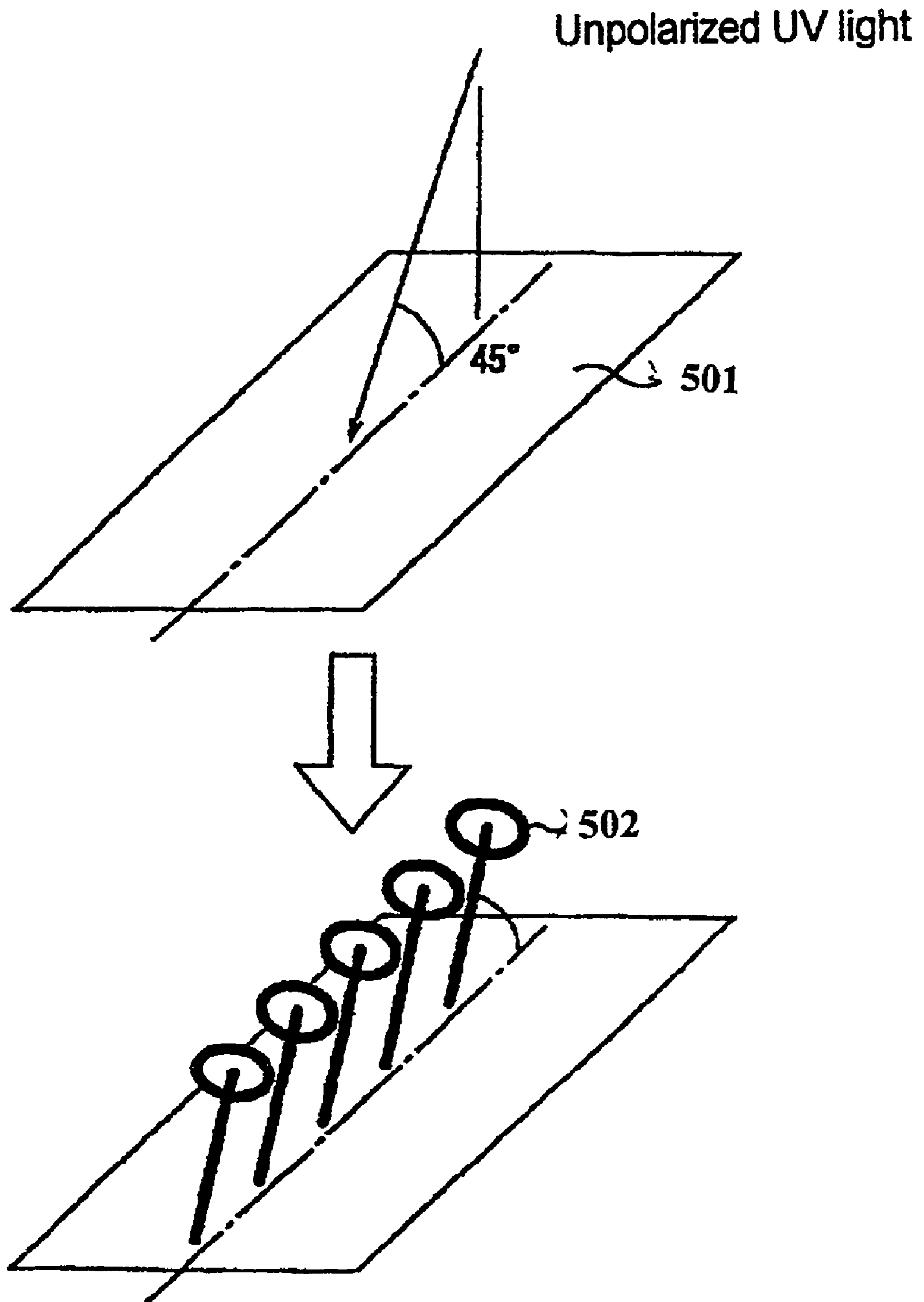
orientation of liquid crystal molecules
