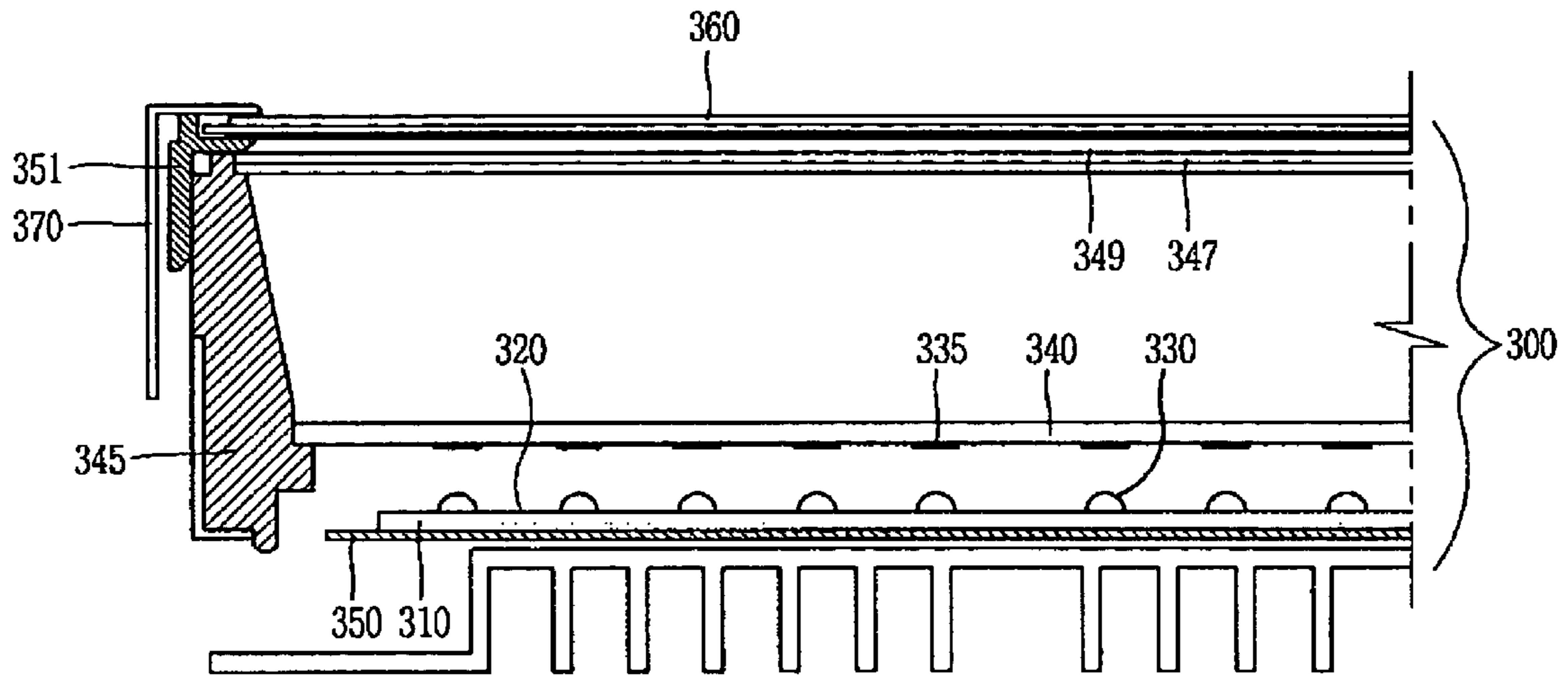
FIG. 1 RELATED ART
