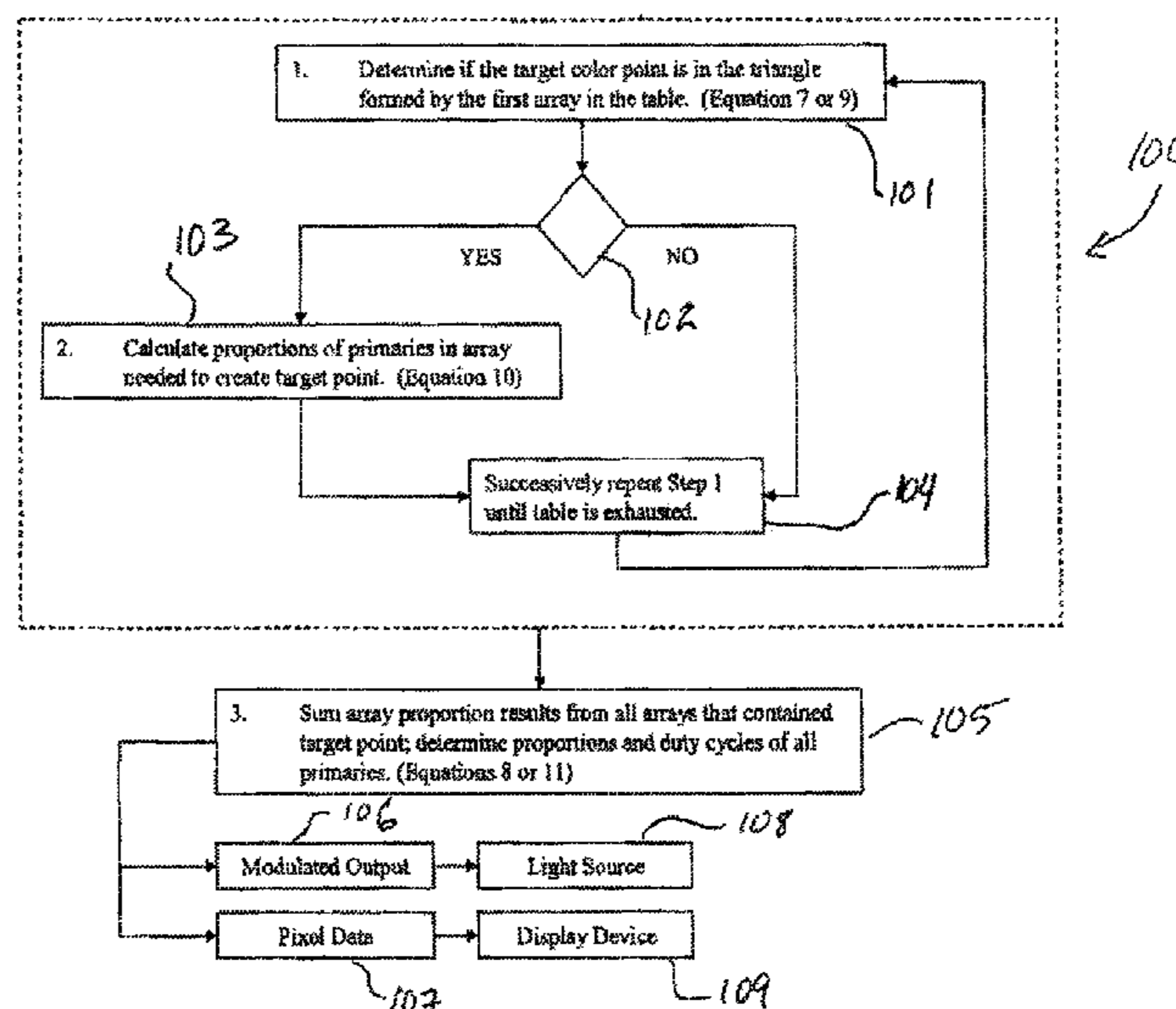
TRIANGLE VERTICES
