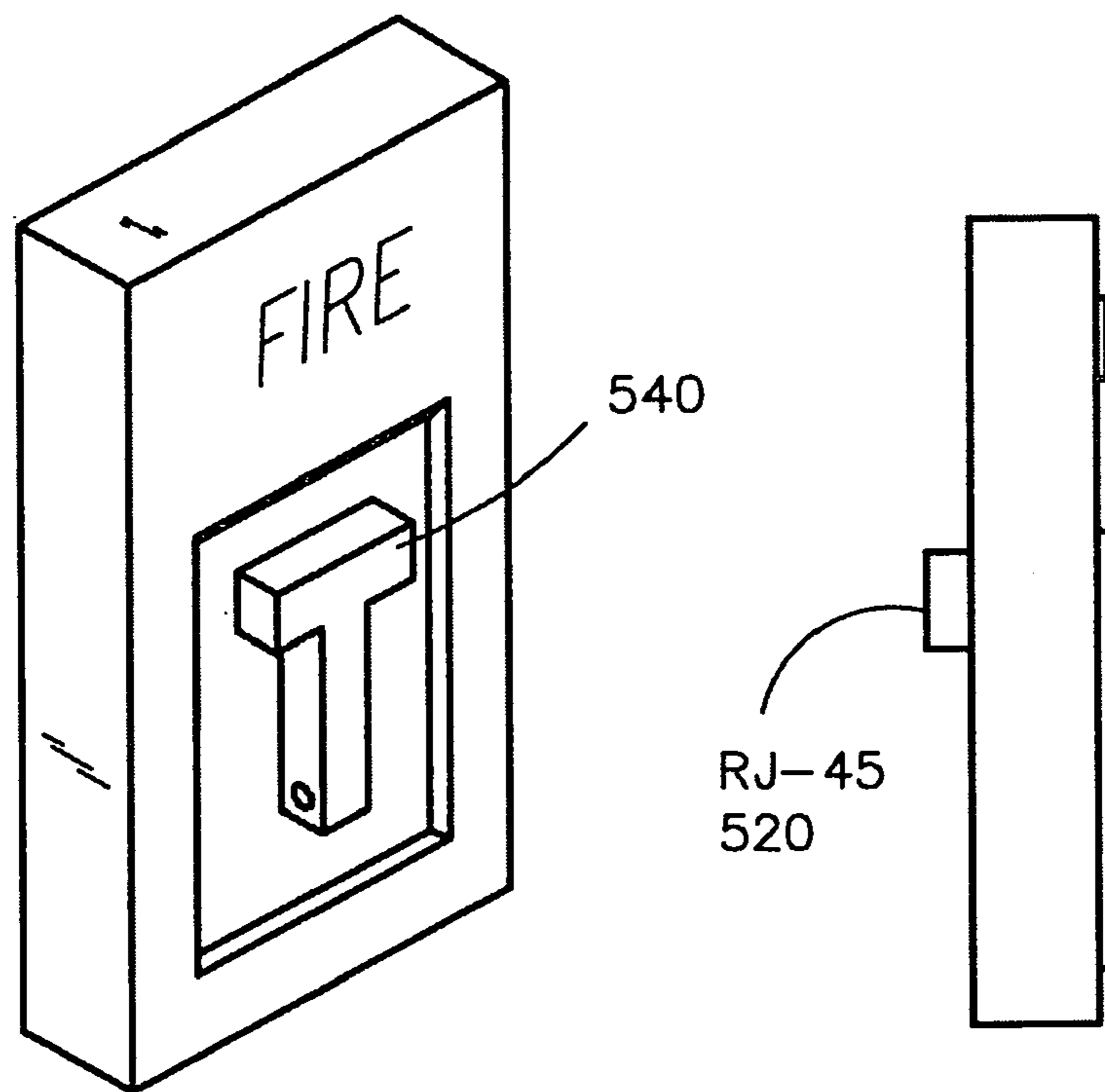
PULL HANDLE
