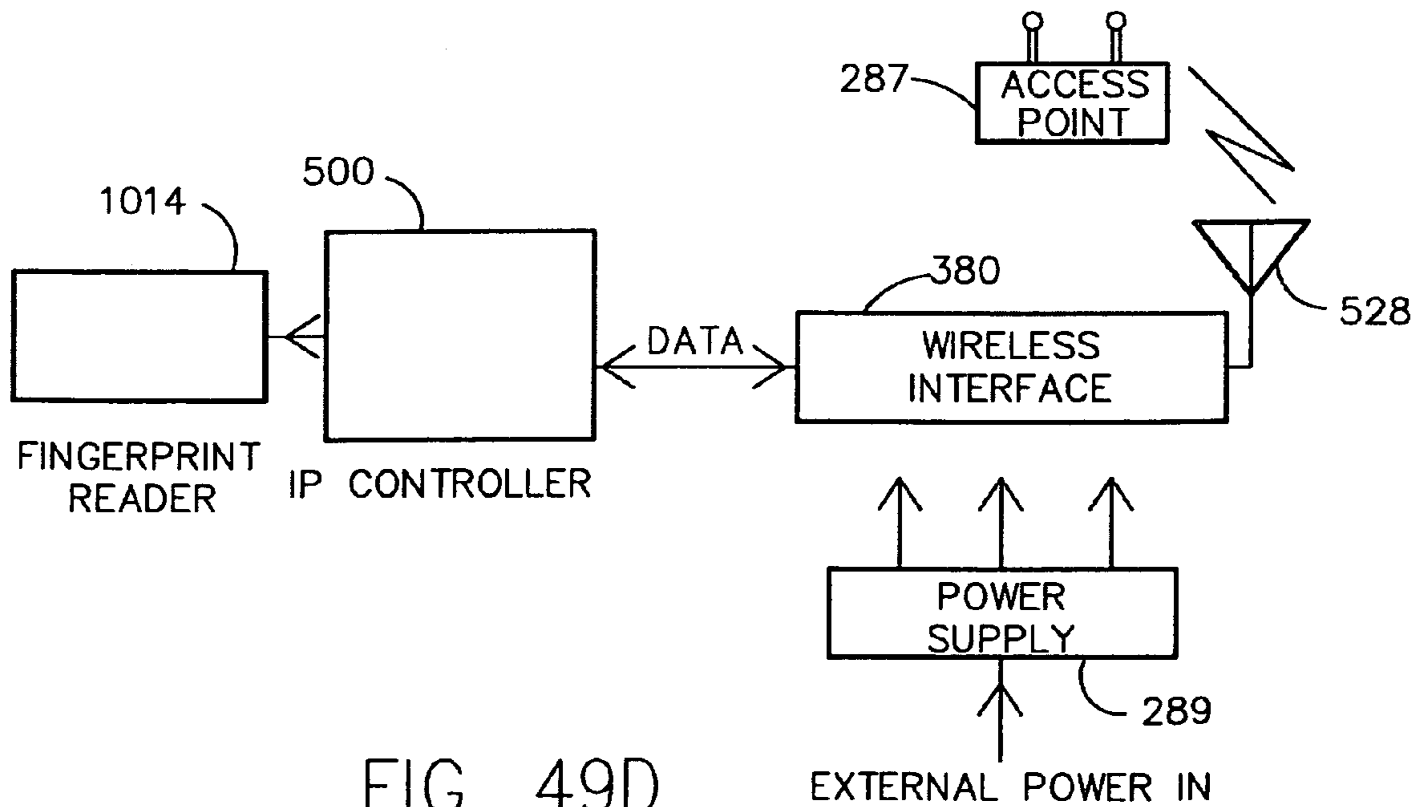
FINGERPRINT READER
