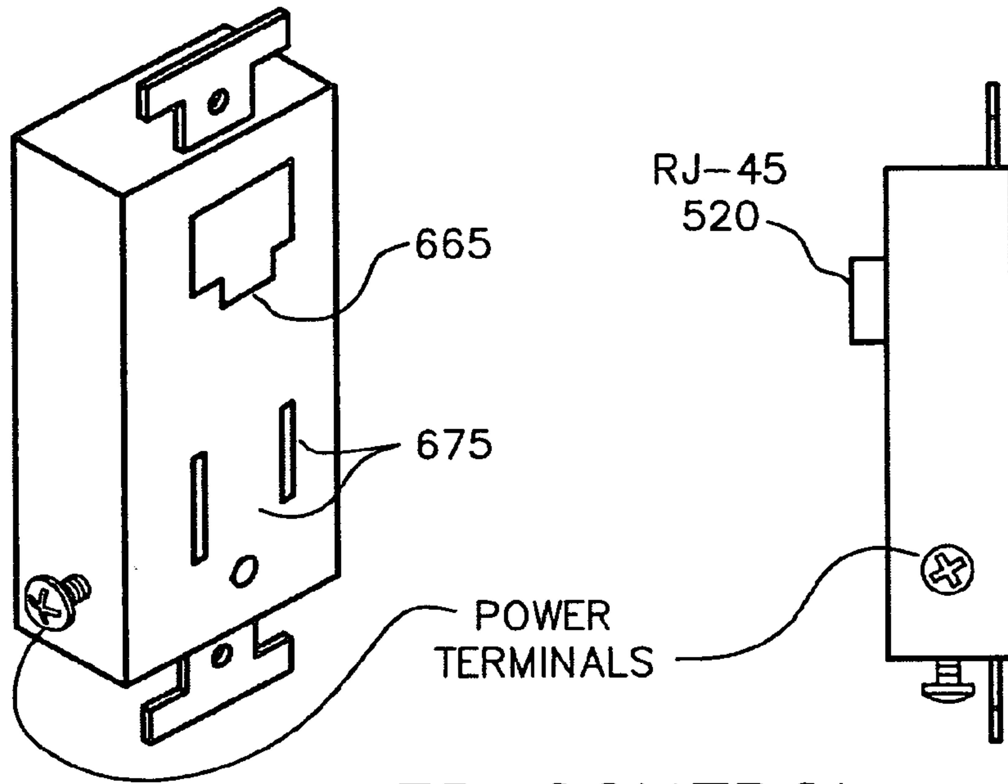
POWER CONTROL (SWITCH OR DIMMER)
