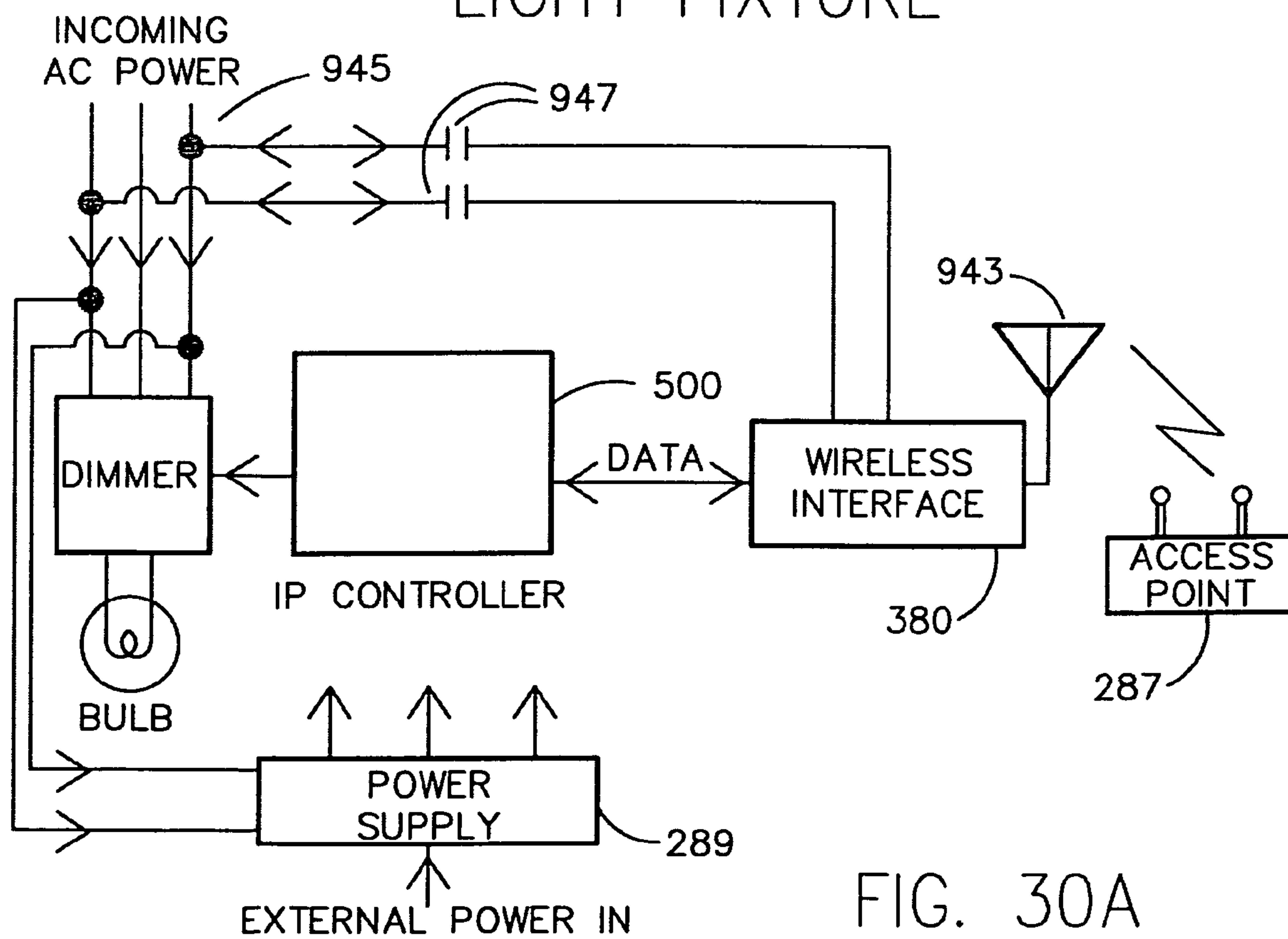
LIGHT FIXTURE
