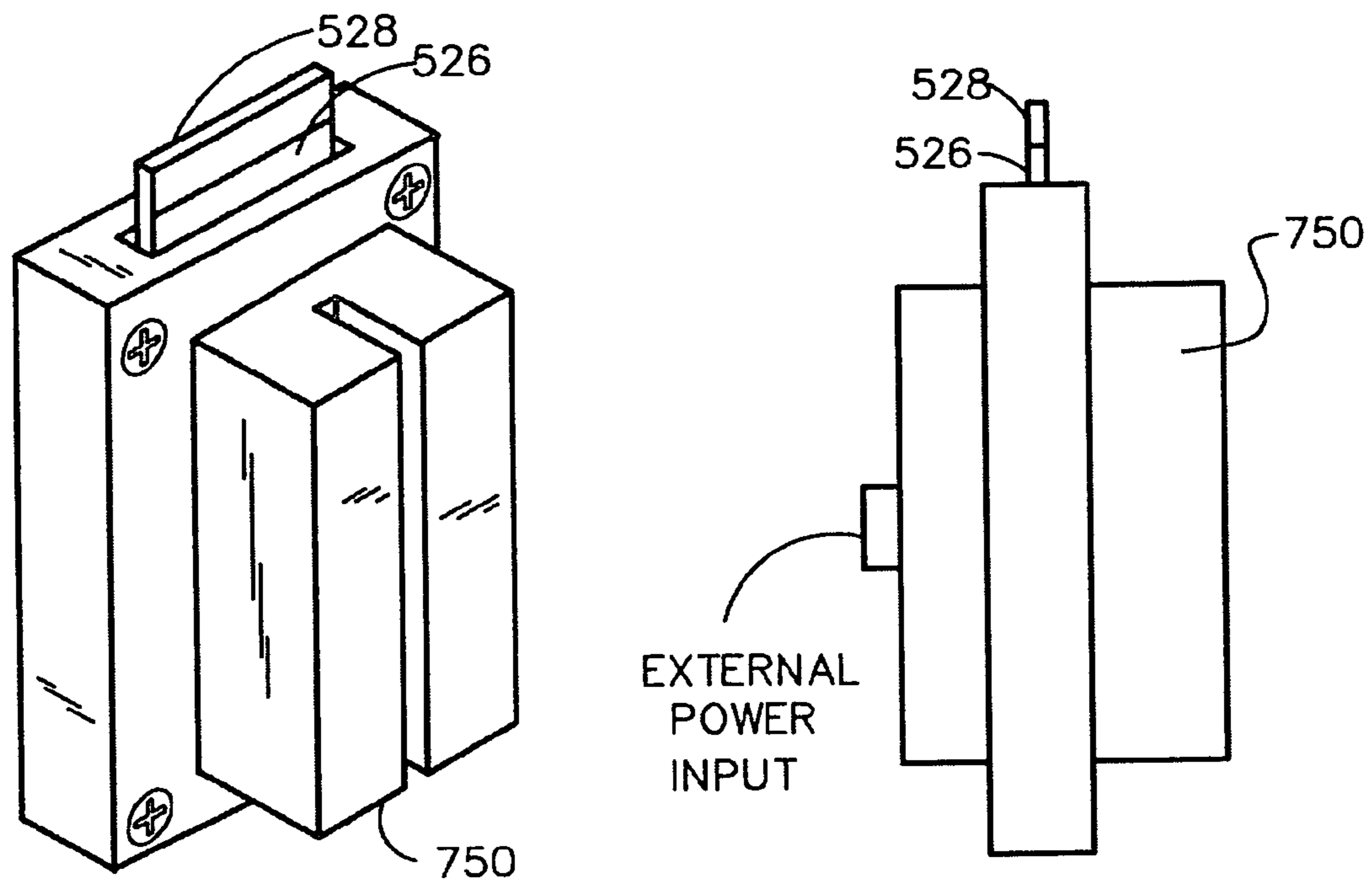
MAG STRIP READER
