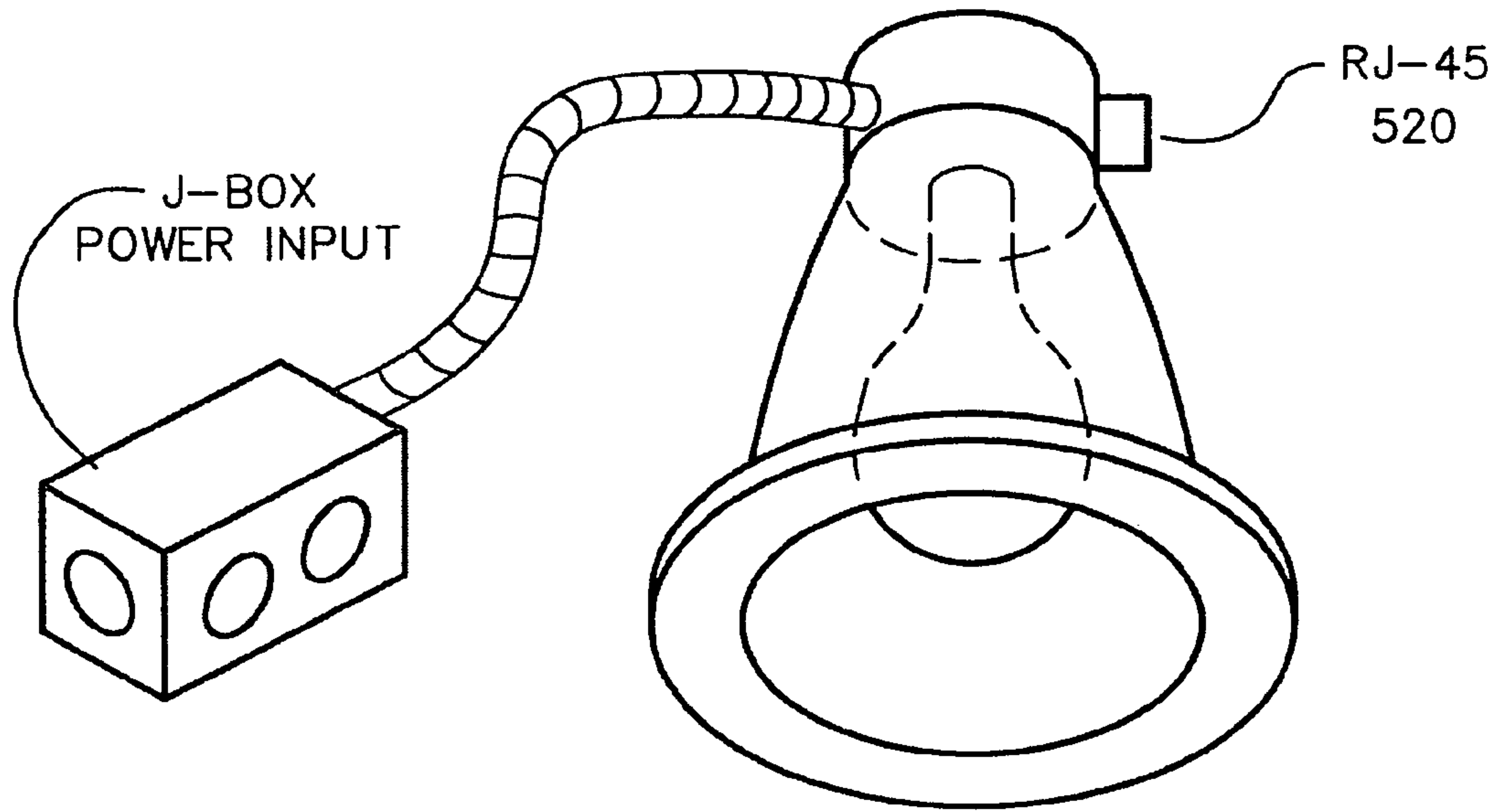
LIGHT FIXTURE
