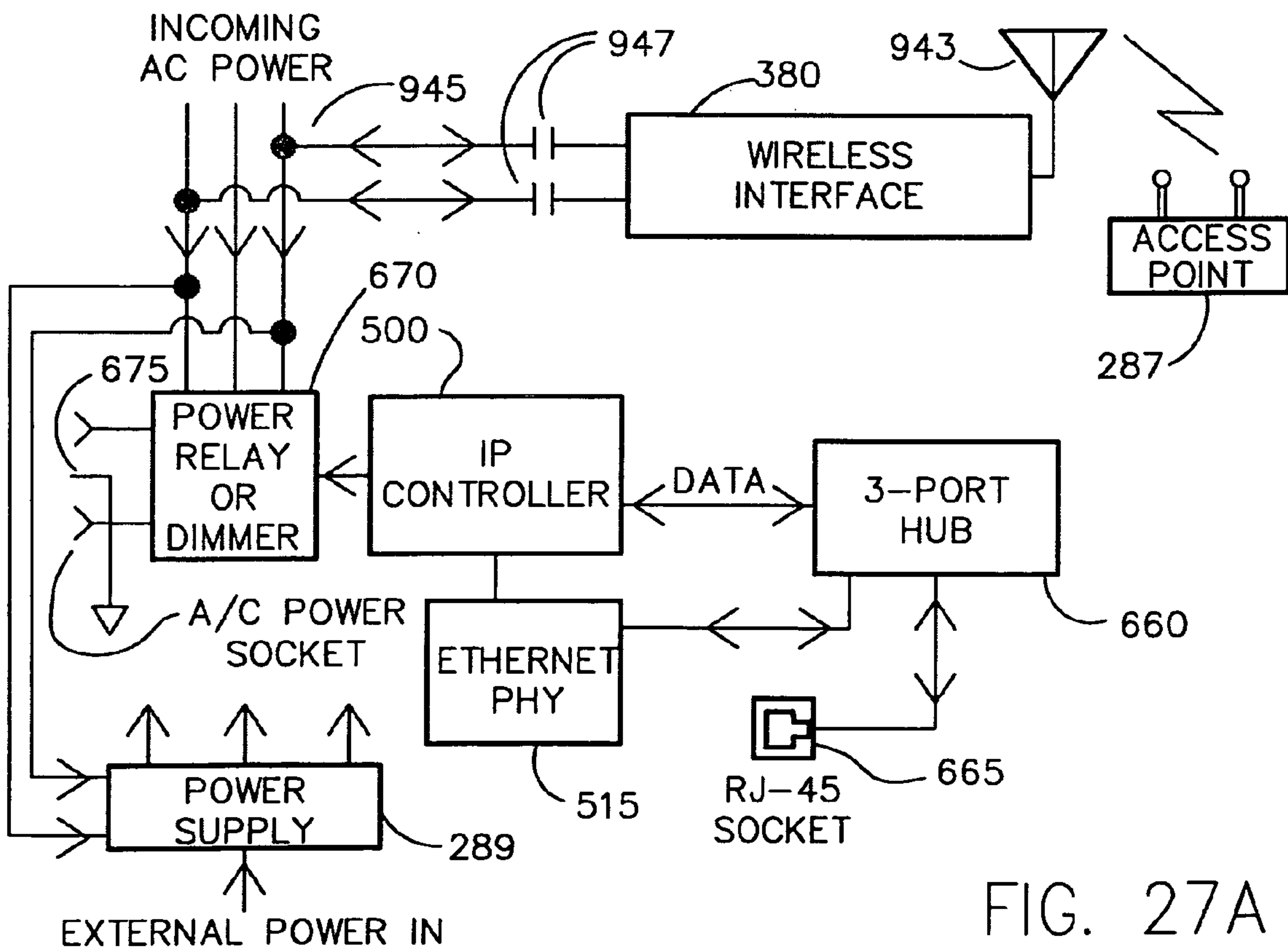
POWER CONTROL (SWITCH OR DIMMER)
