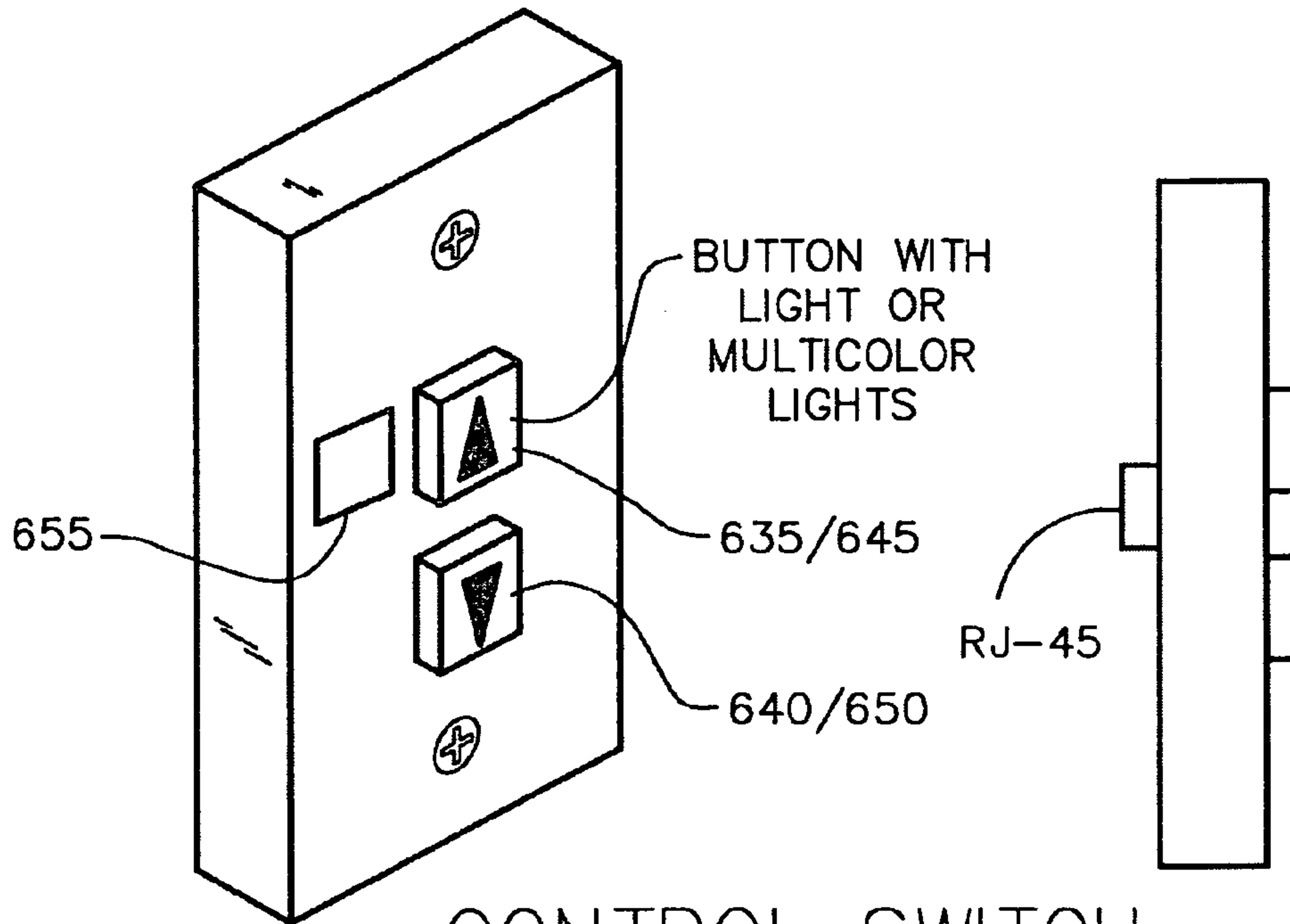
CONTROL SWITCH INDICATOR LIGHT
