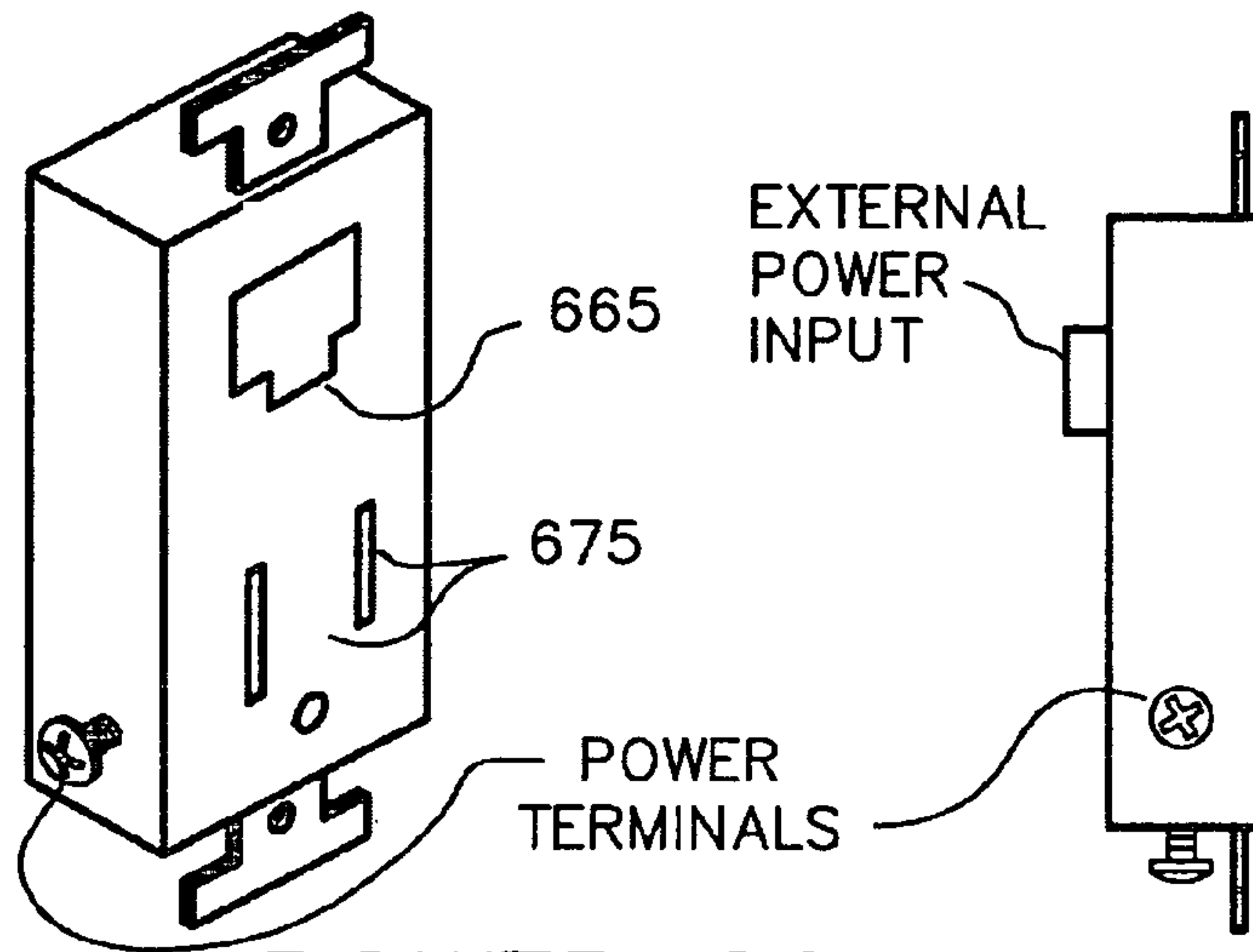
POWER CONTROL (SWITCH OR DIMMER)
