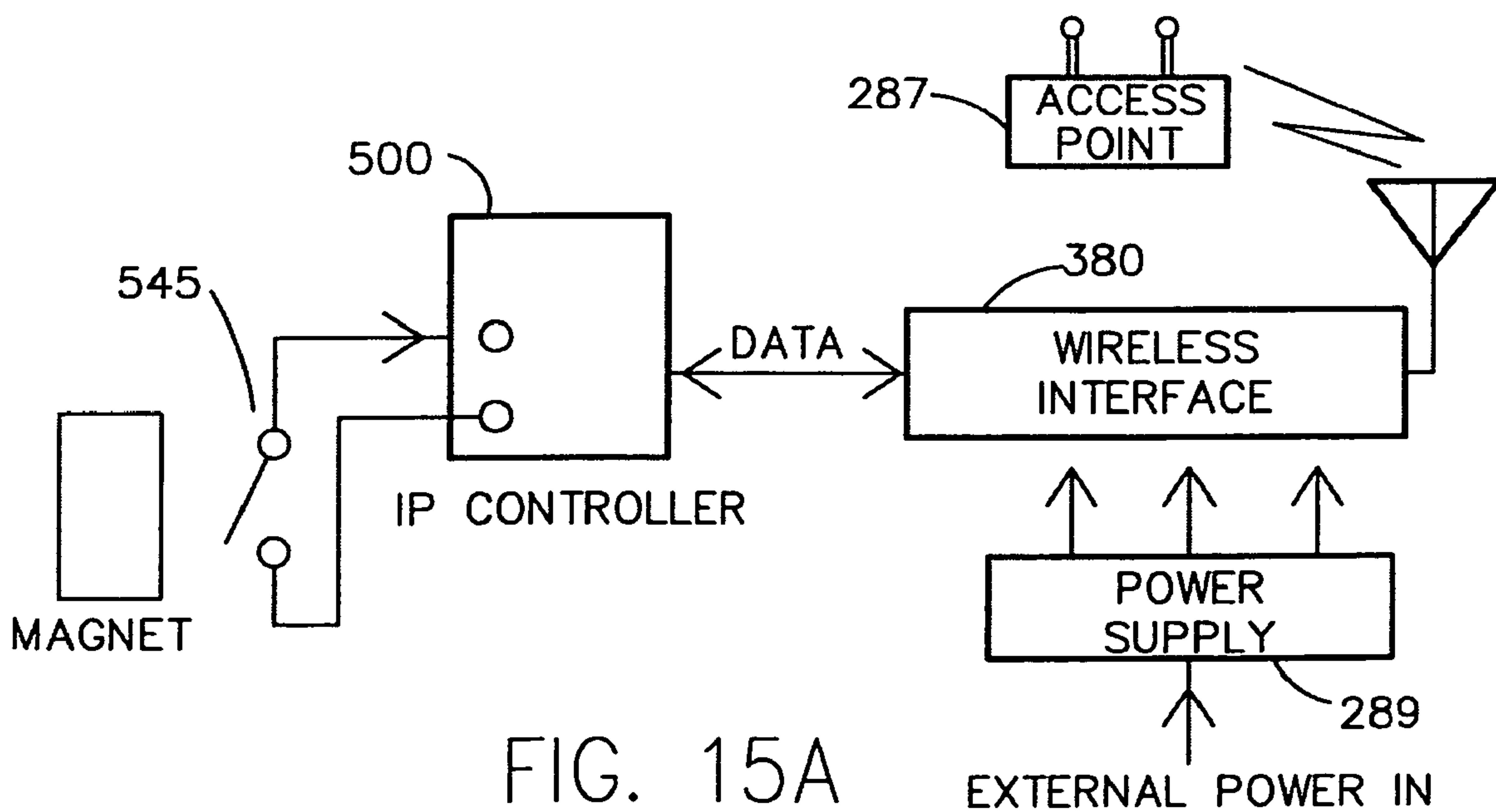
INTERNAL CONTACT INTERFACE
