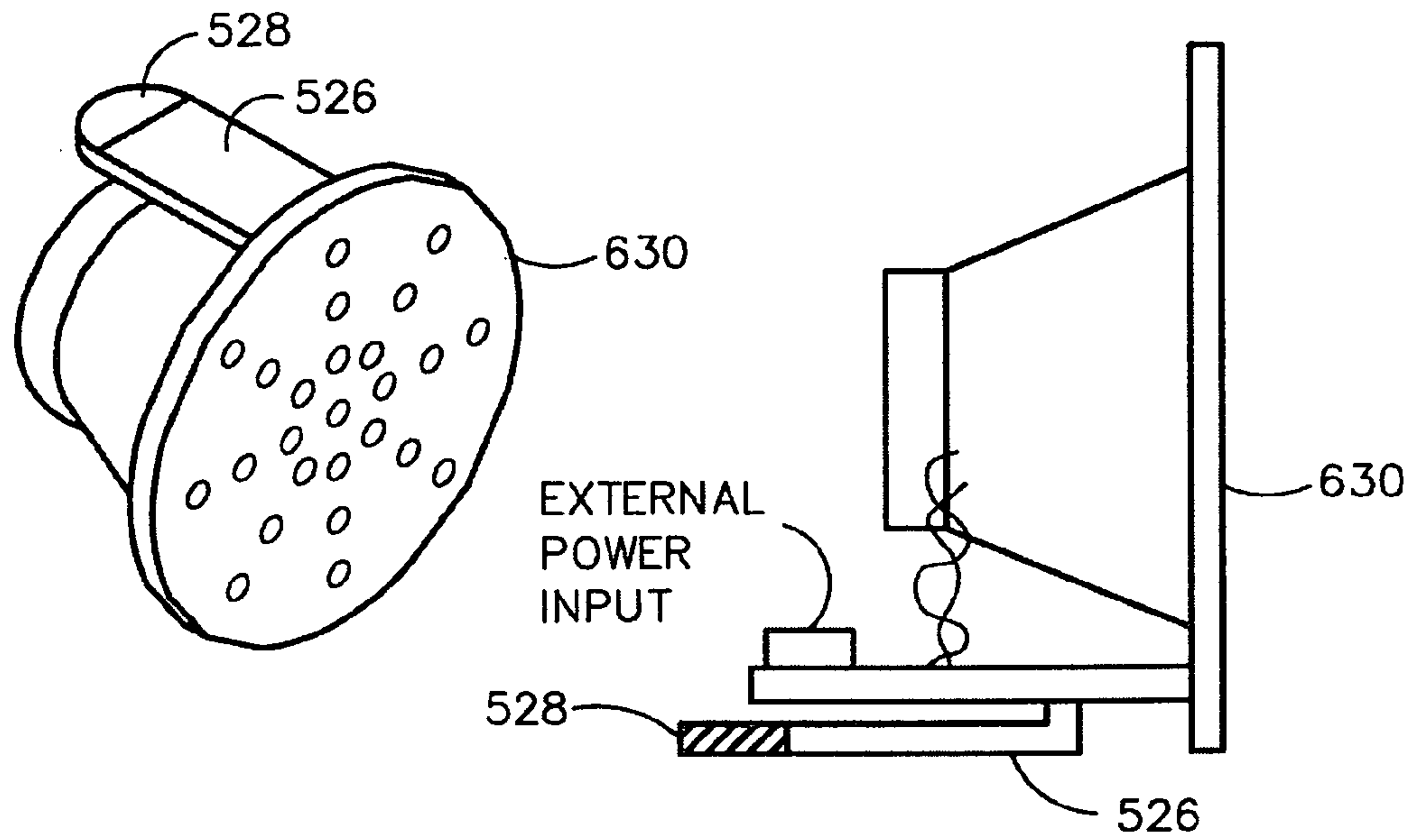
LOUDSPEAKER WITH AMPLIFIER
