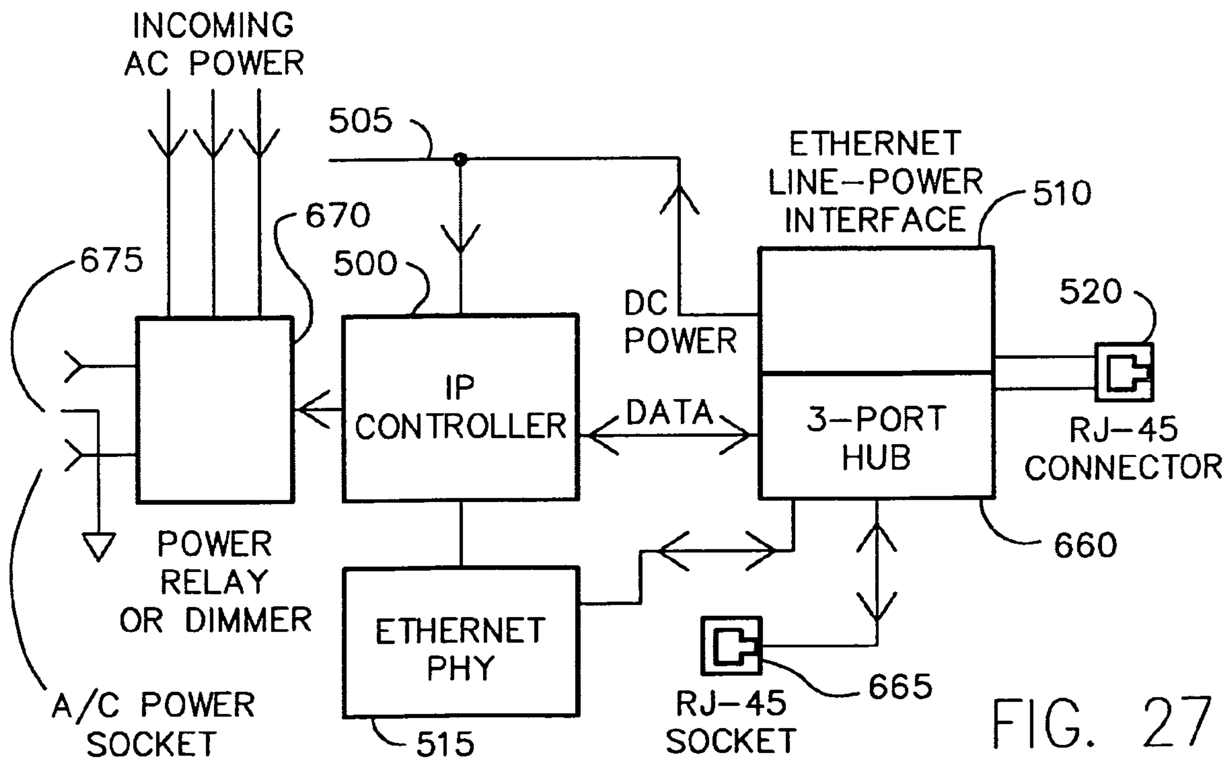
POWER CONTROL (SWITCH OR DIMMER)
