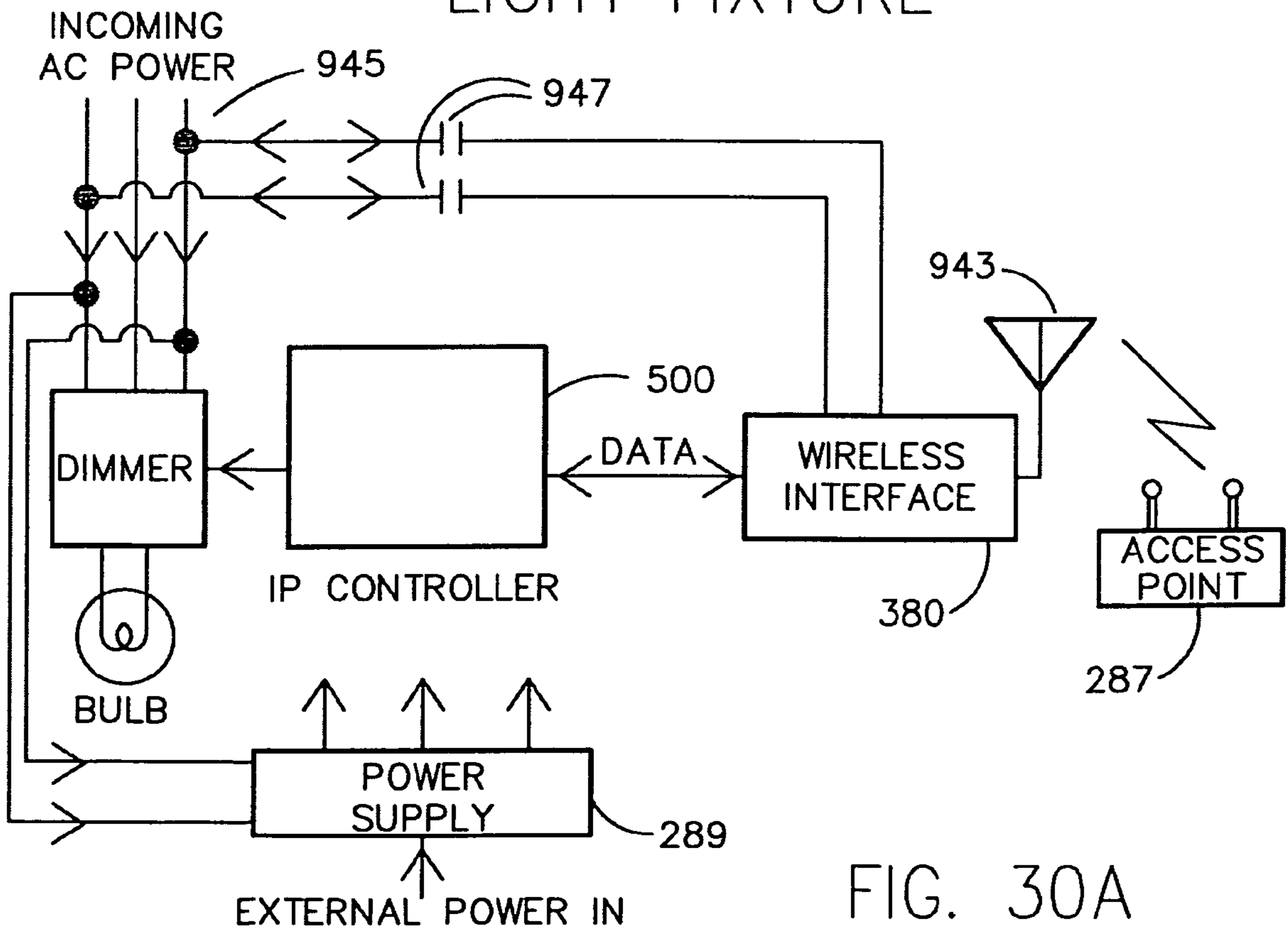
LIGHT FIXTURE
