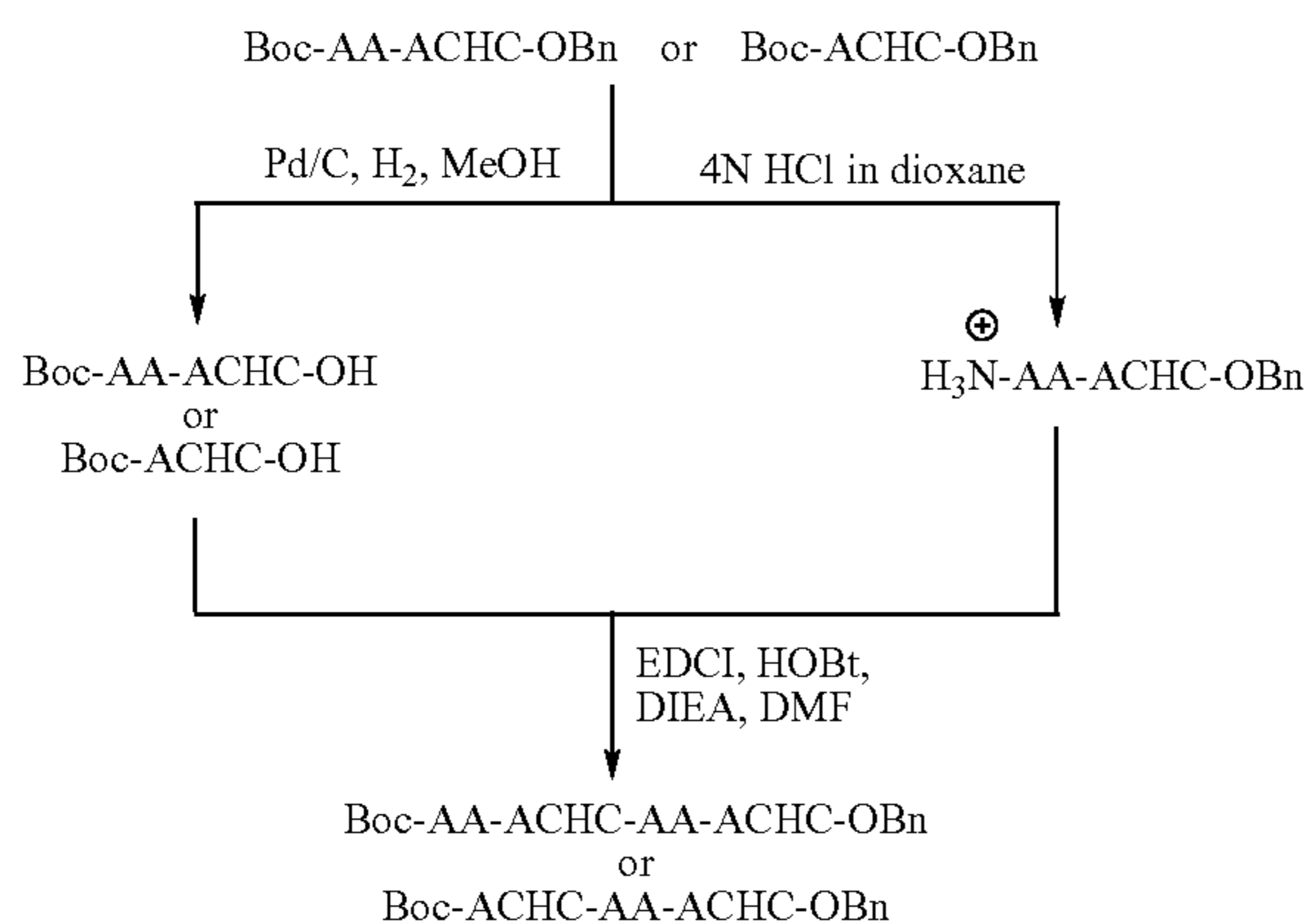
Scheme 2. Synthetic Route to Oligomers with more than 3 Residues; AA = \alpha -amino acid
