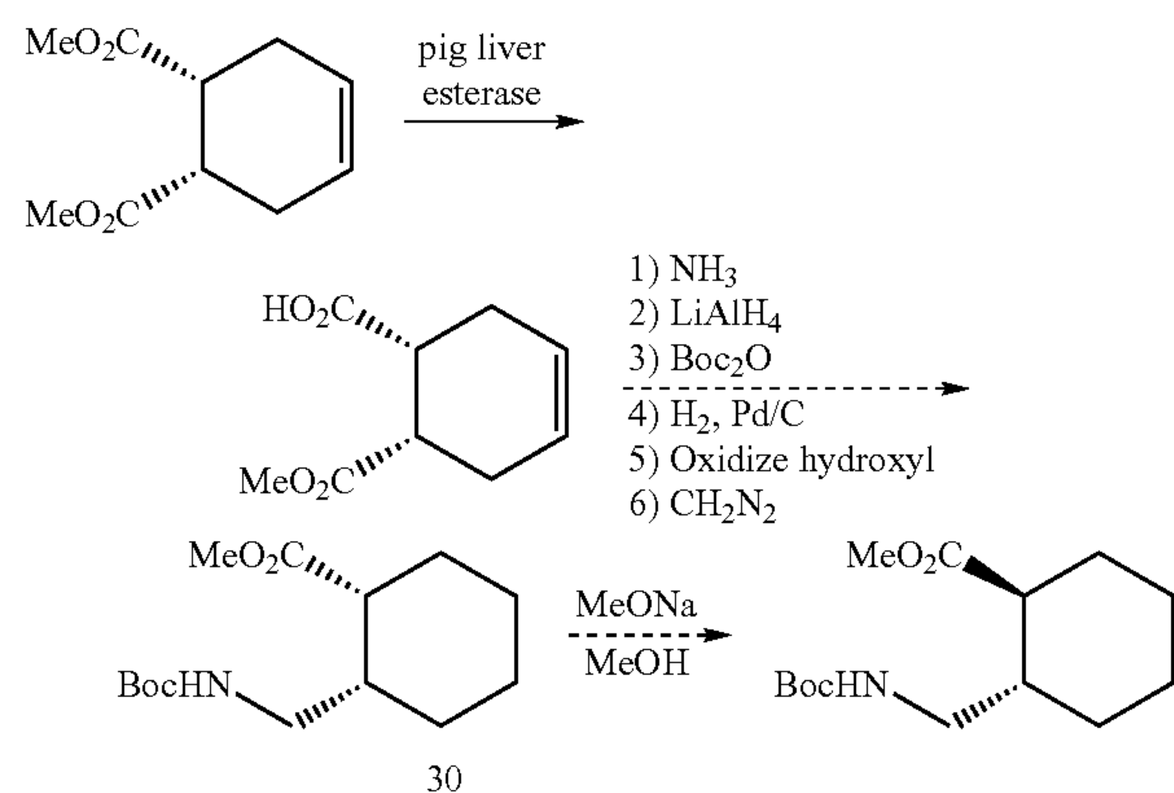
SCHEME 2
