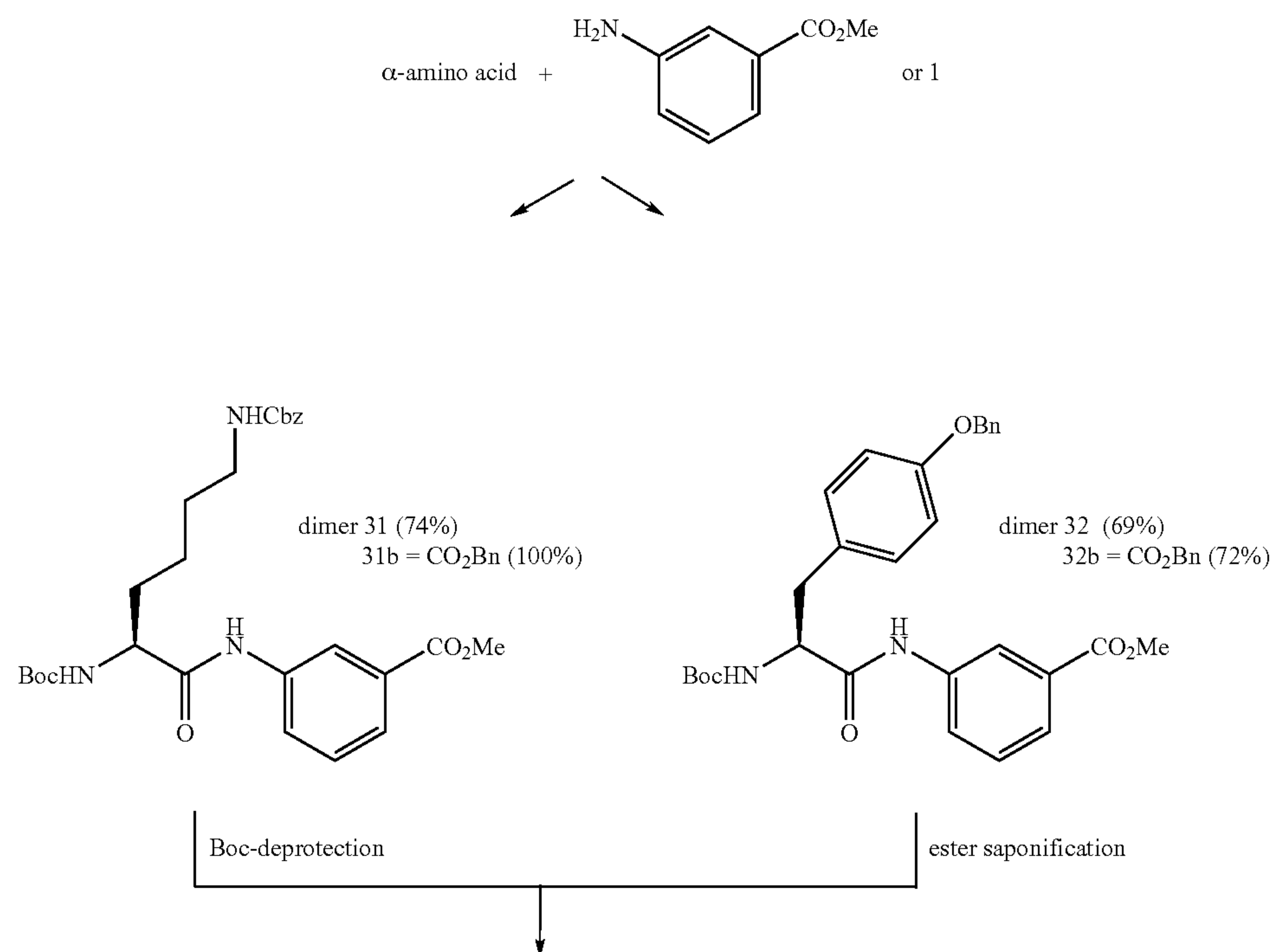
Scheme 11
