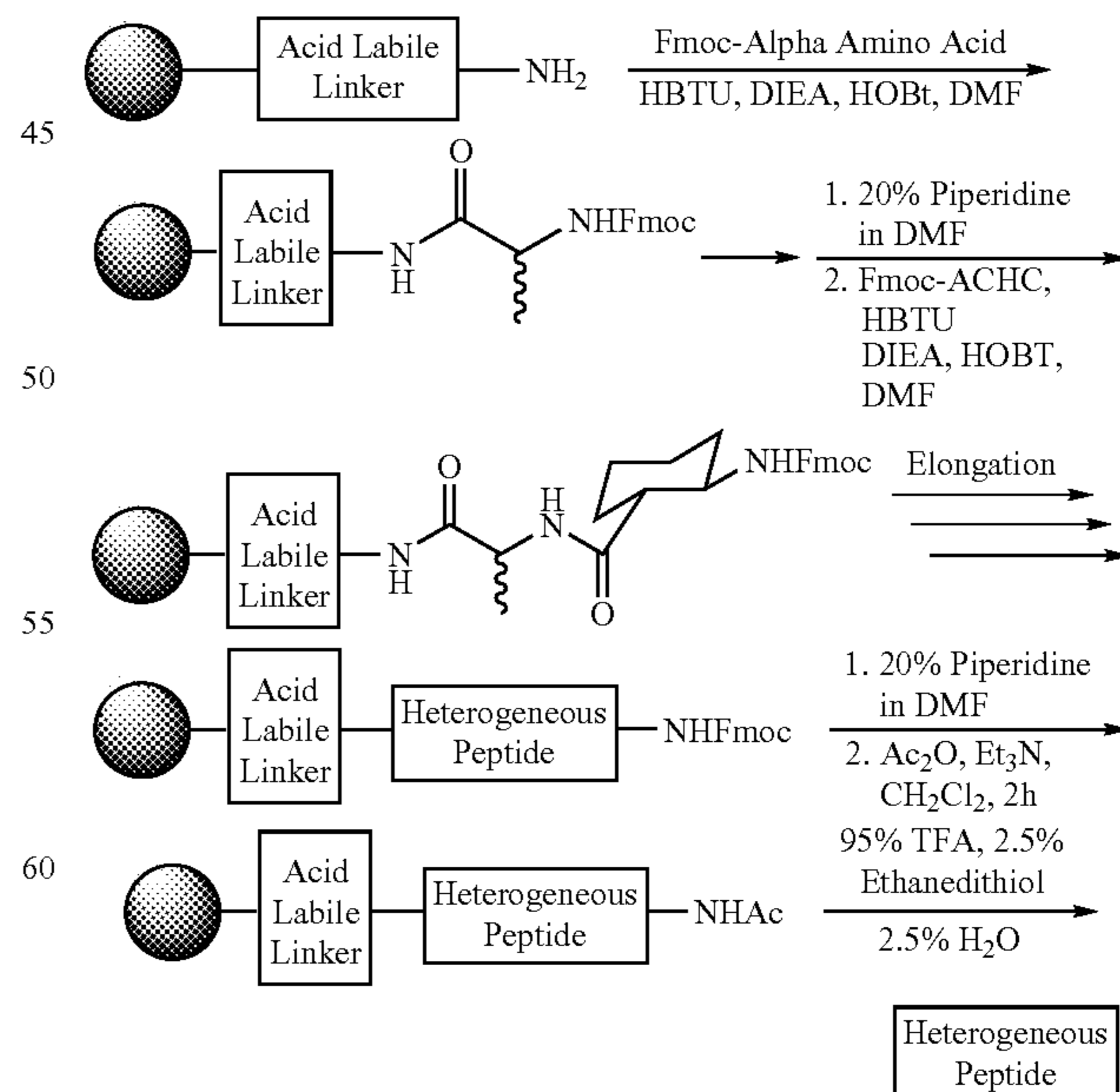
Scheme 3. Generalized Route for Solid Phase Synthesis
