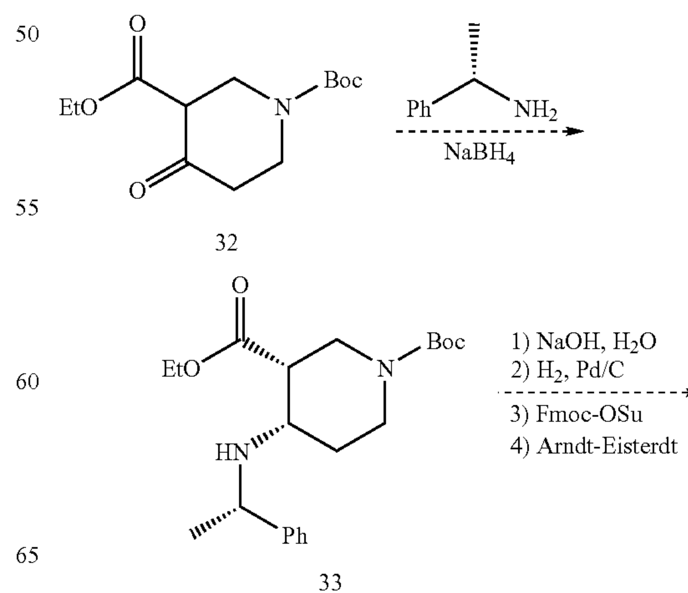
SCHEME 3
