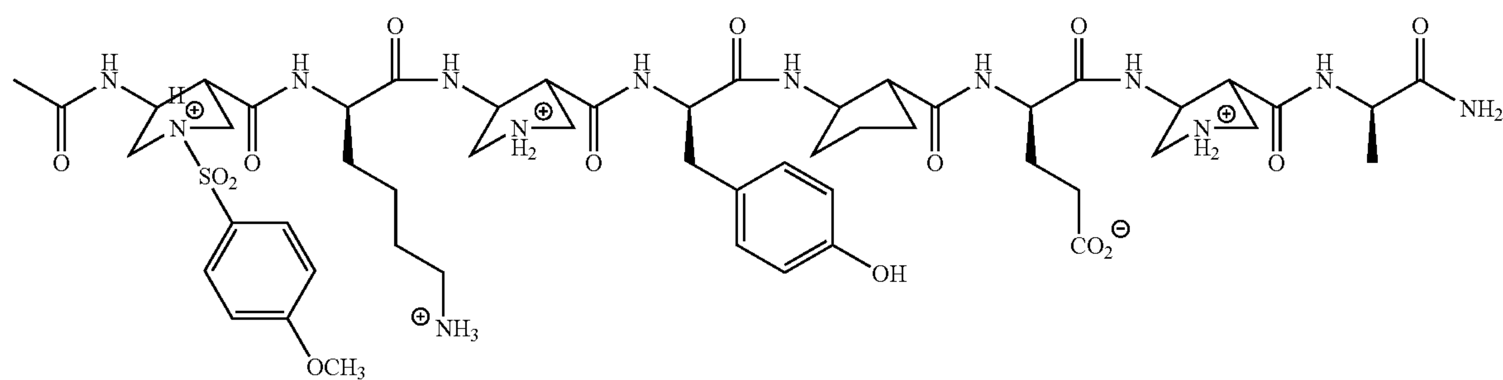
Ac-APC(SO 2 R)-K-APC-Y-ACPC-E-APC-A-NH 2
