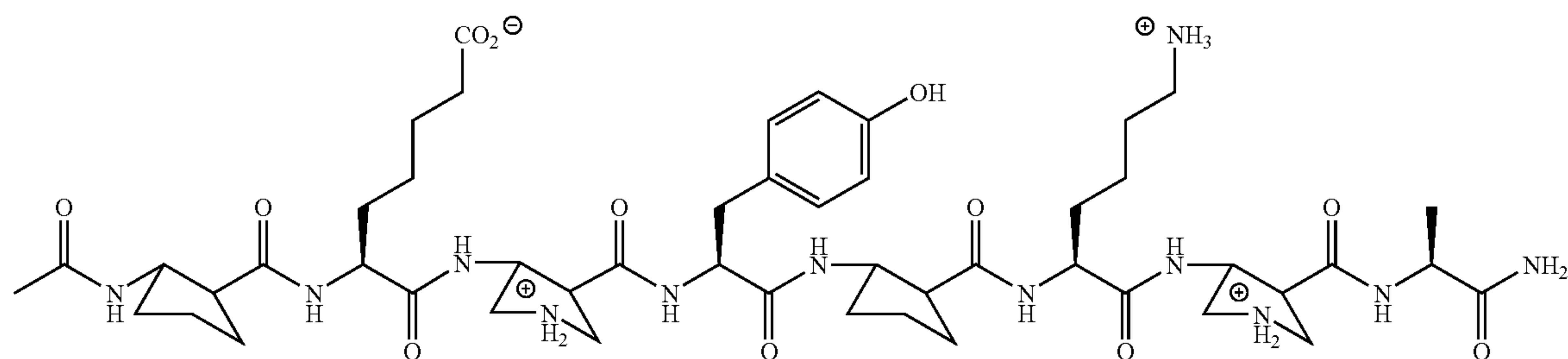
Ac-ACPC-E-APC-Y-ACPC-K-APC-A-NH 2
