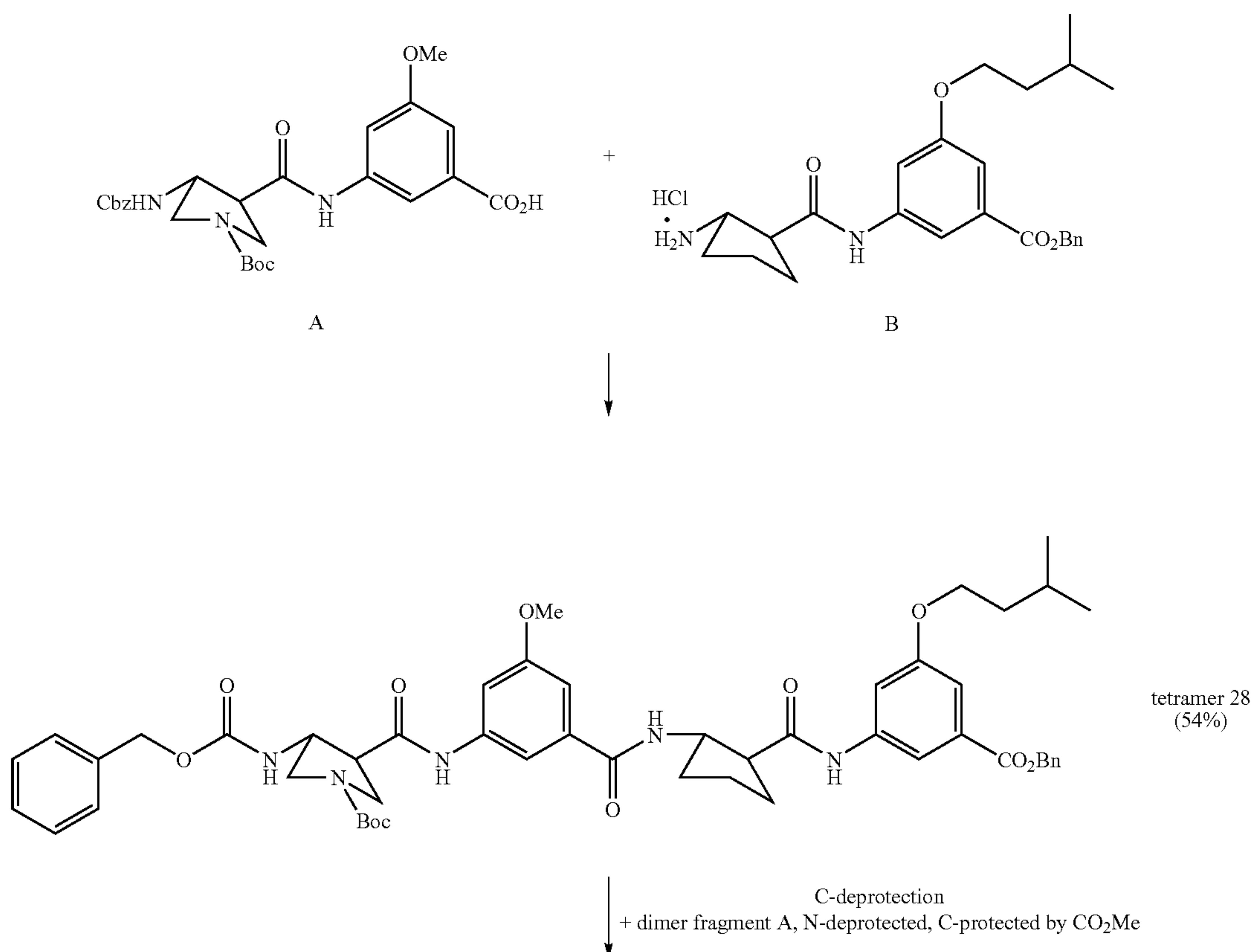
Scheme 10
