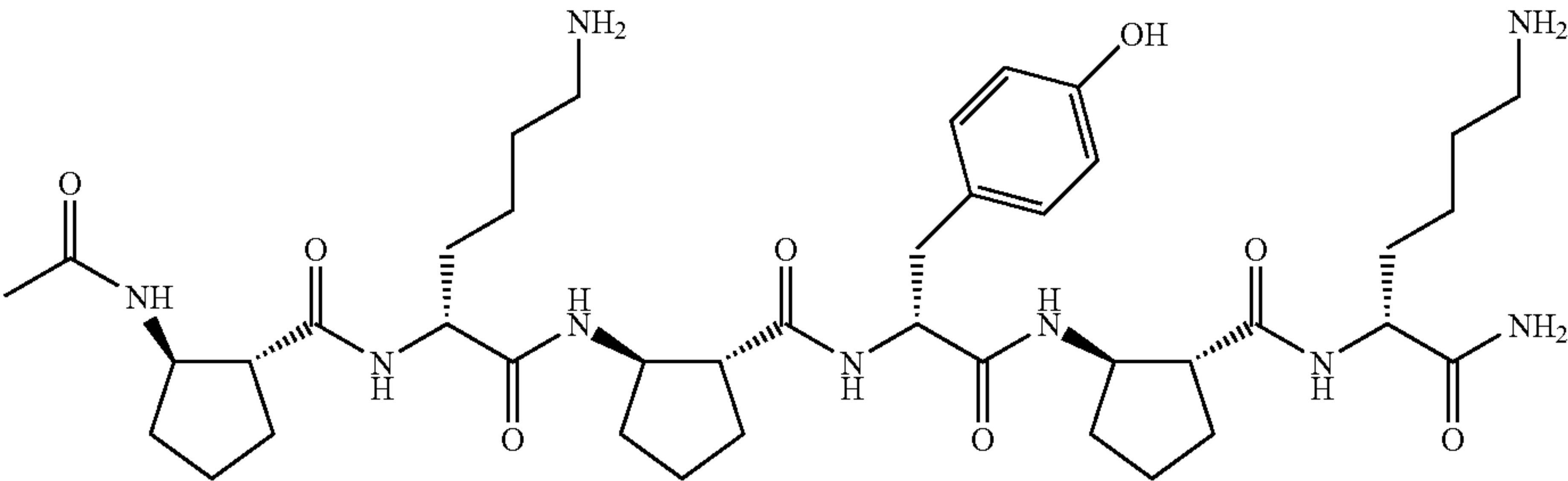
(R,R)-ACPC D-amino acids
