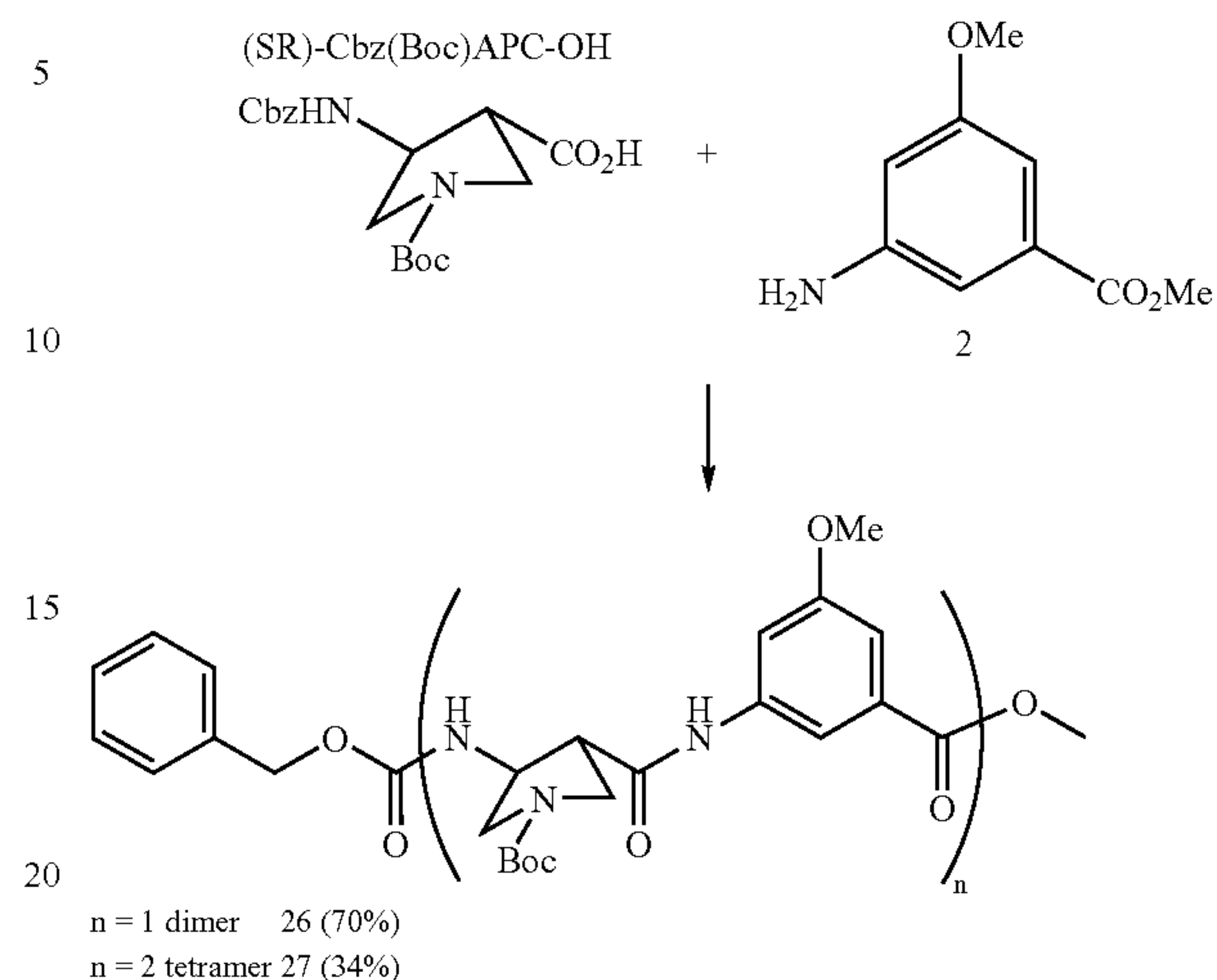
Scheme 9
