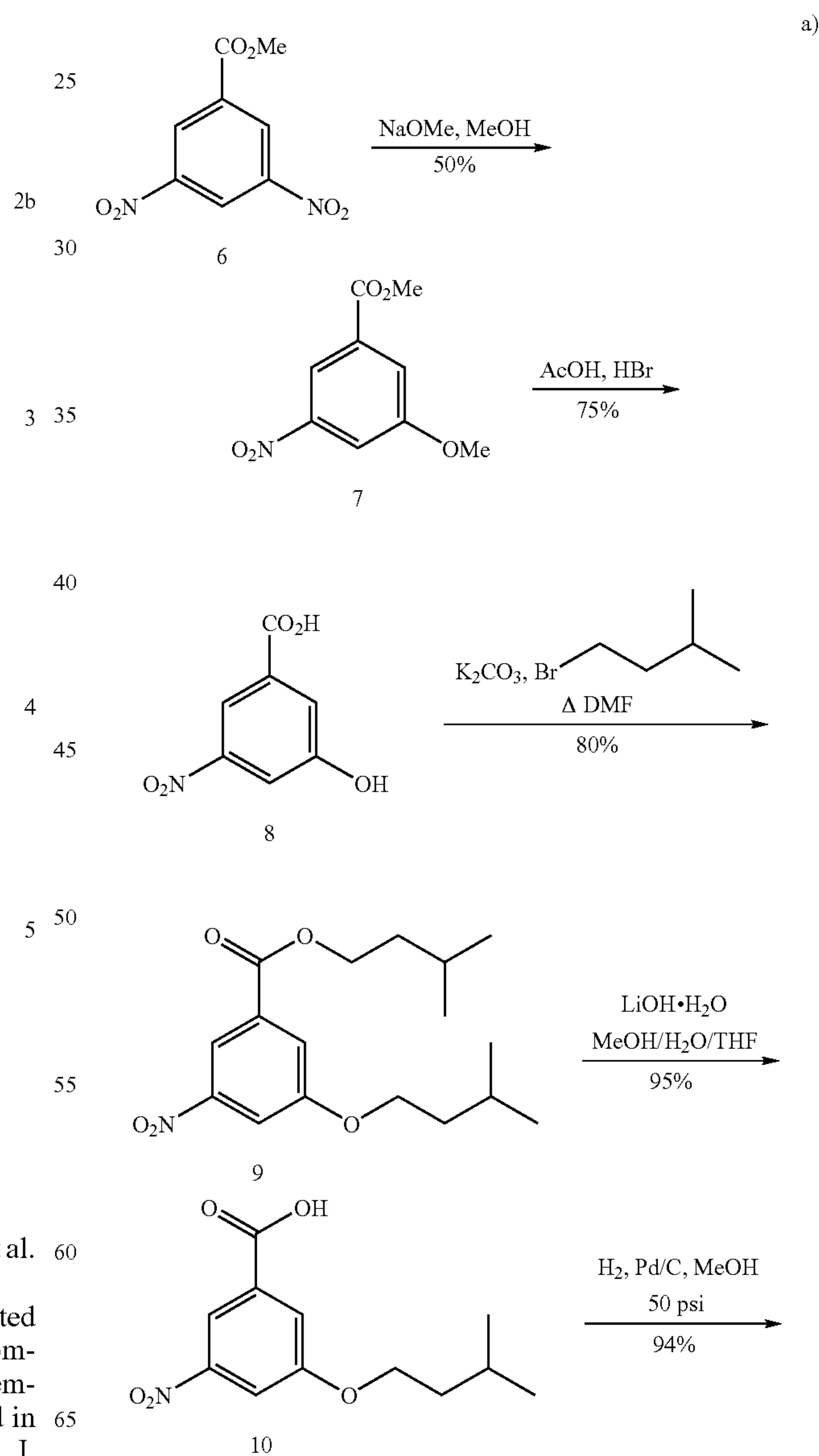
Scheme 4
