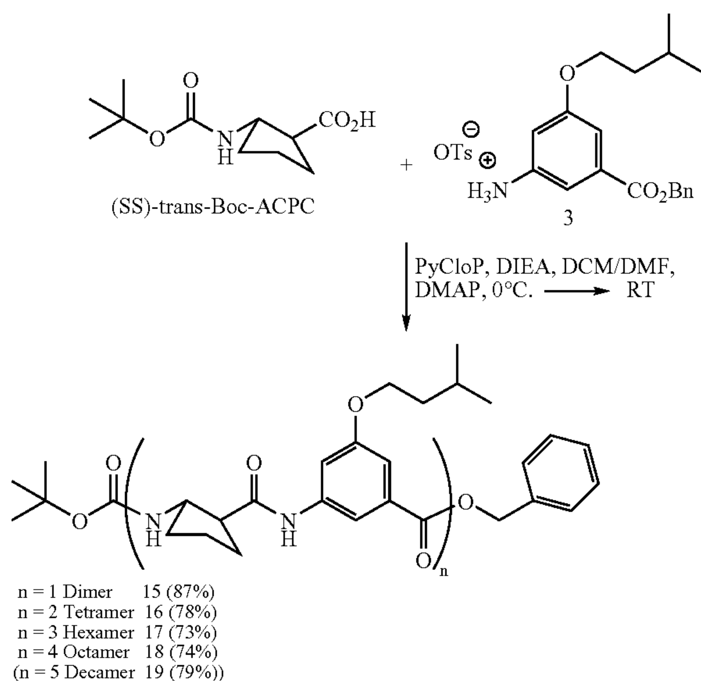
Scheme 7
