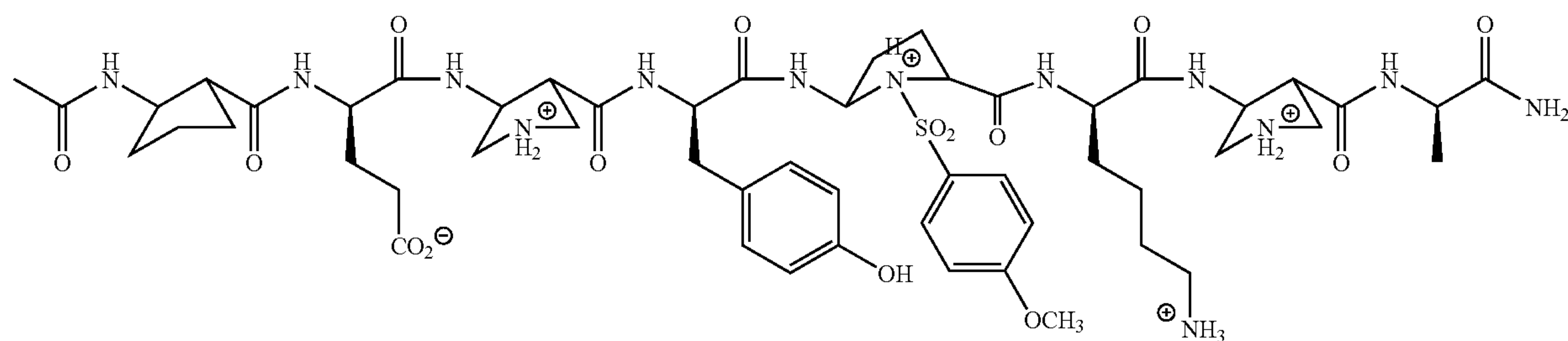
AC-ACPC-E-APC-Y-APC(SO 2 R)-K-APC-A-NH 2
