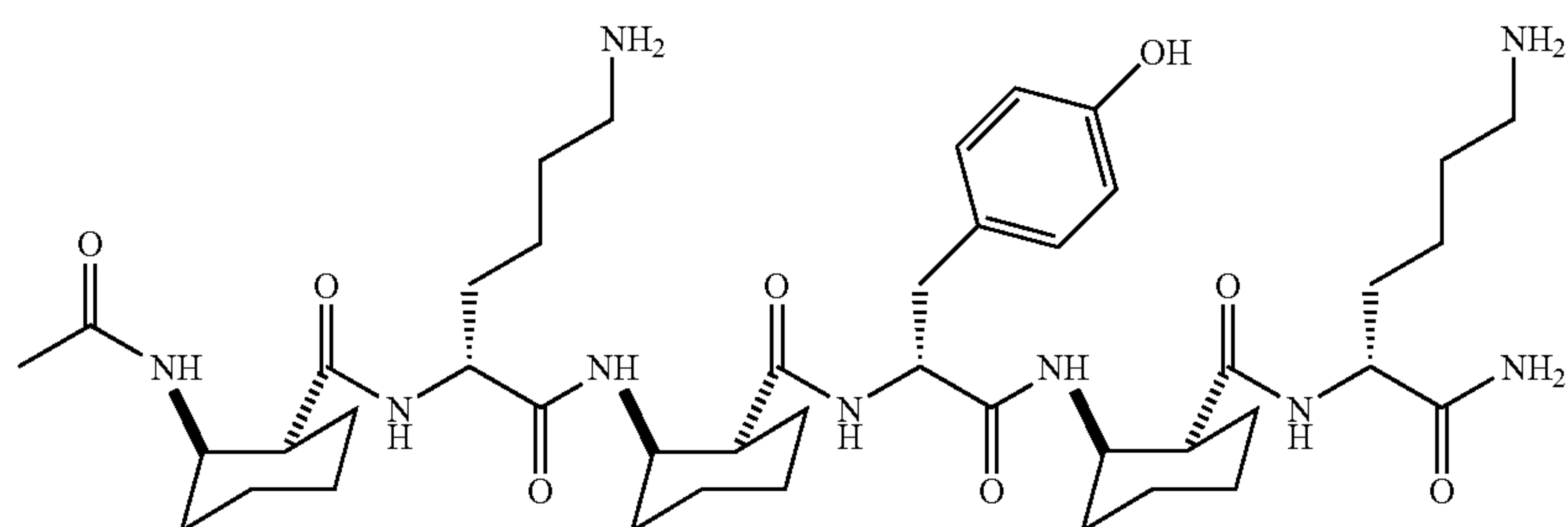
R,R-ACHC and D-Alpha Amino Acid
