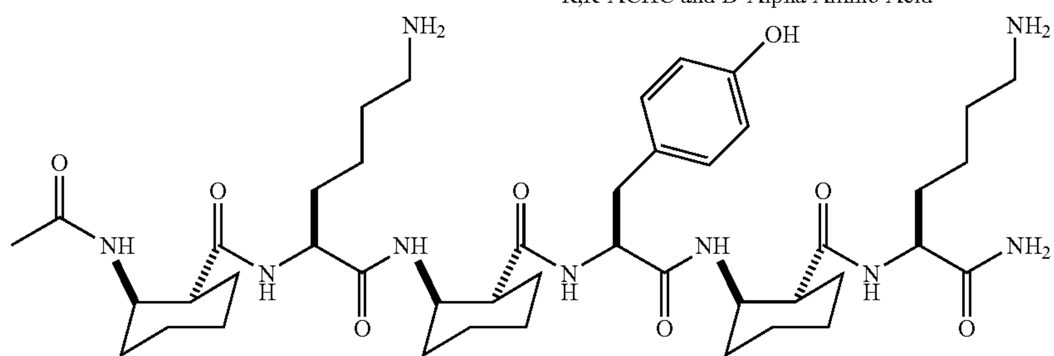
R,R-ACHC and L-Alpha Amino Acid
