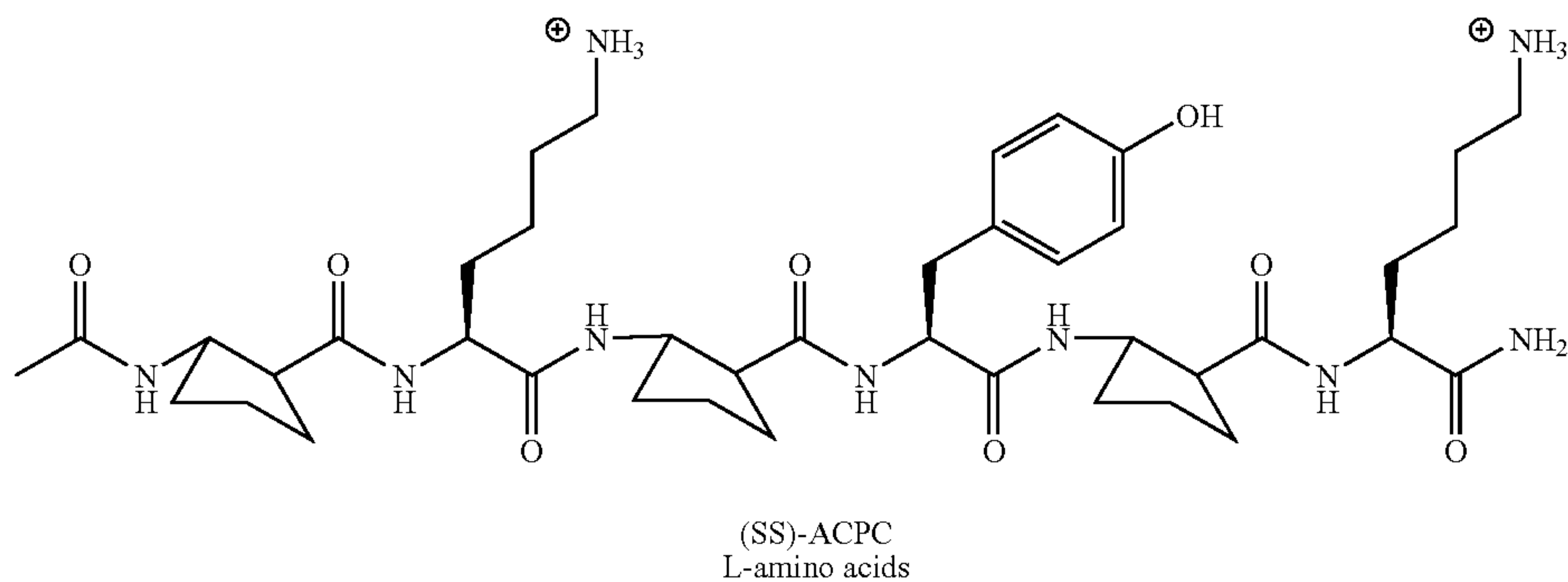
First generation \alpha/\beta peptides
