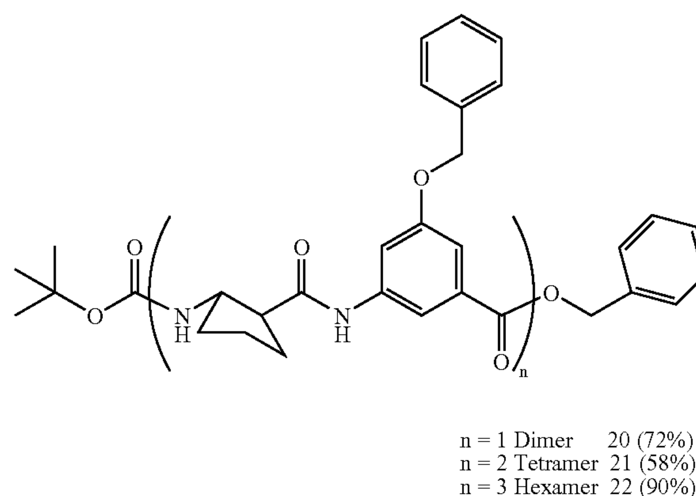
Scheme 8
