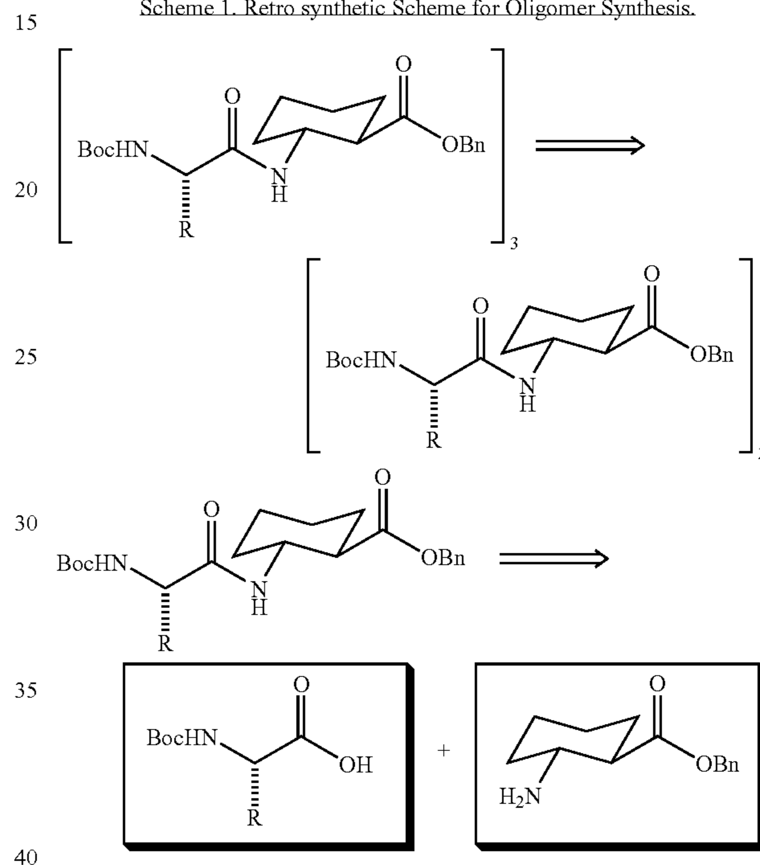
Scheme 1. Retro synthetic Scheme for Oligomer Synthesis.
