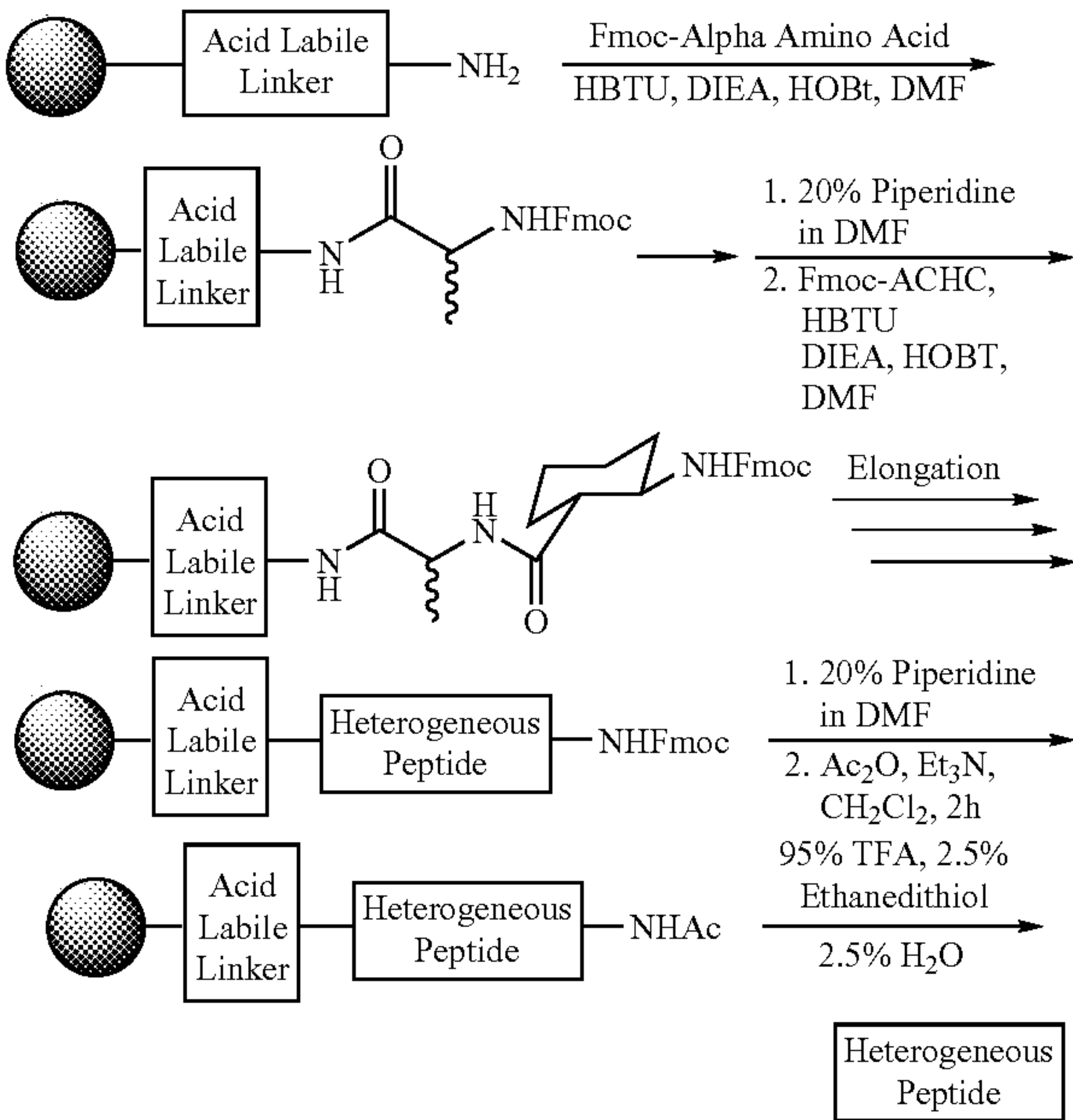
Scheme 3. Generalized Route for Solid Phase Synthesis
