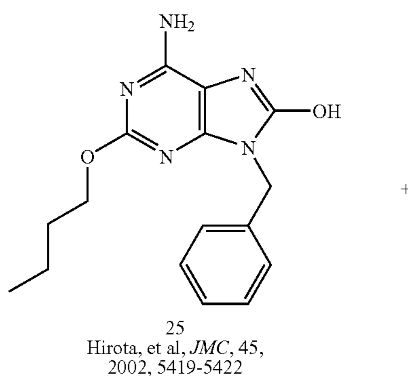
Scheme 7
