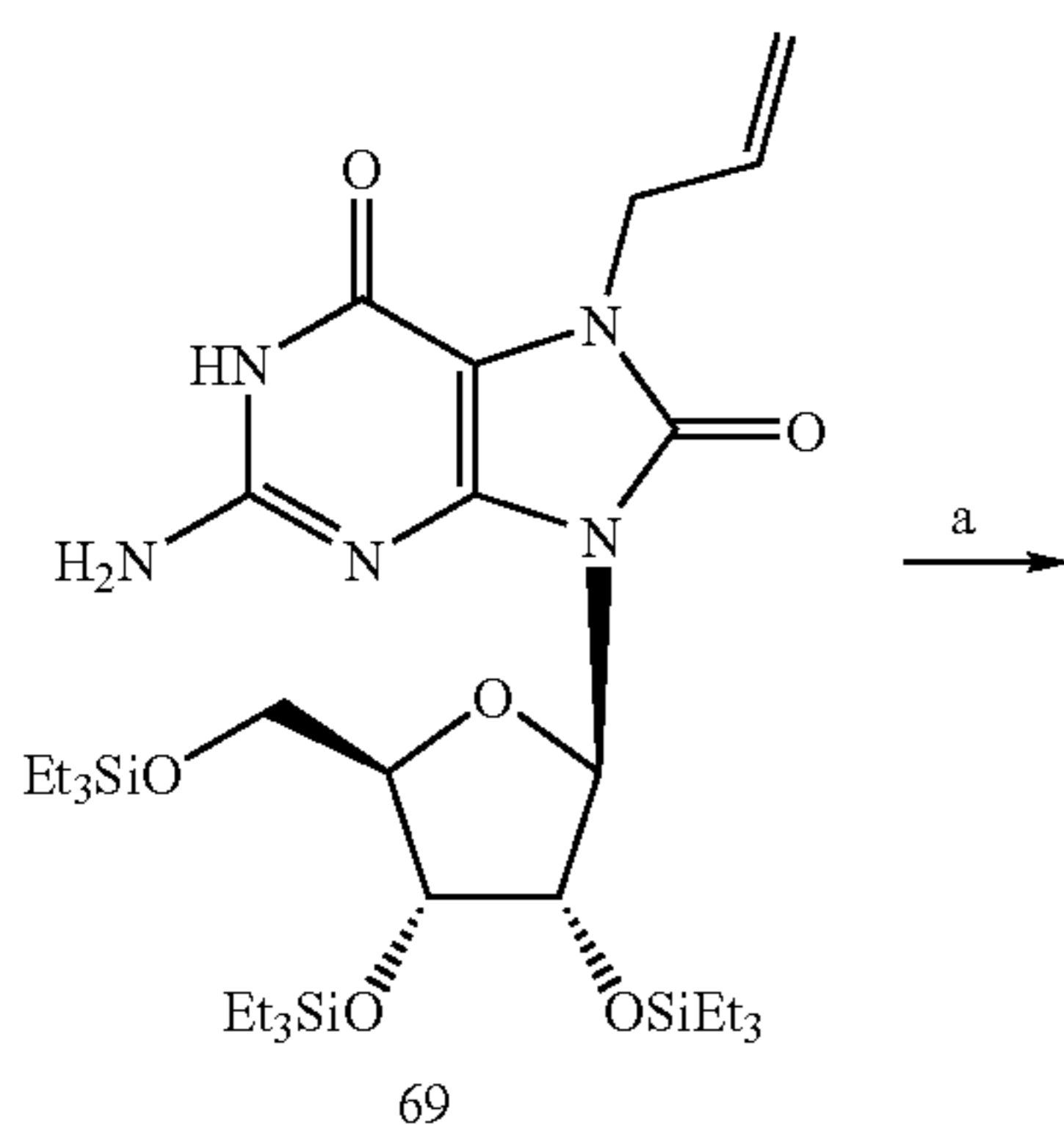
Scheme 18
