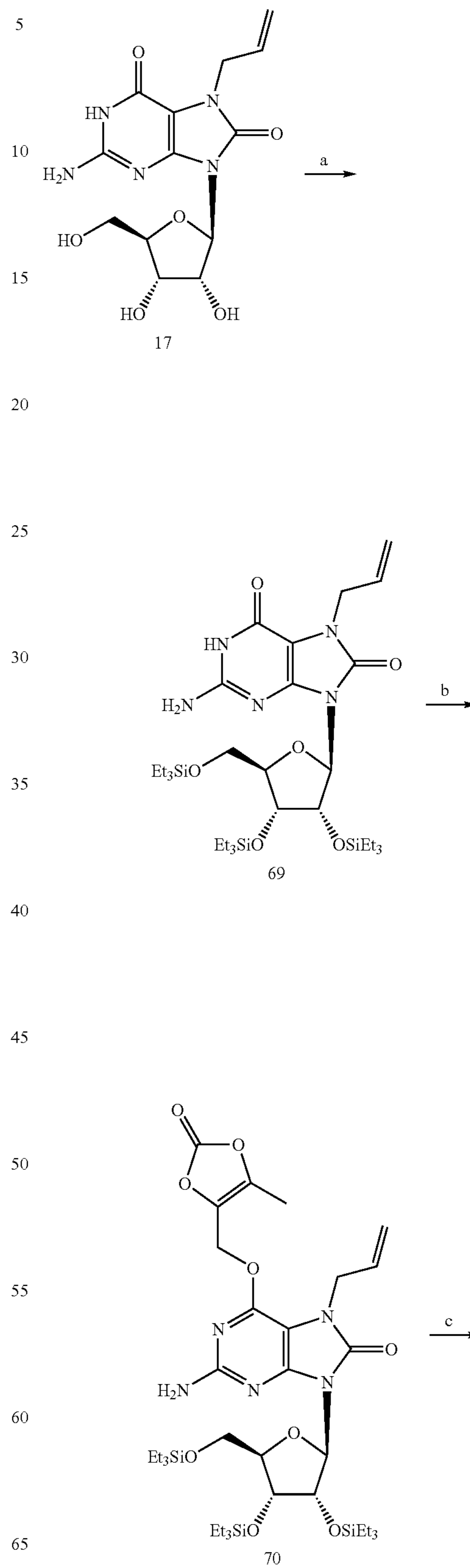
Scheme 17
