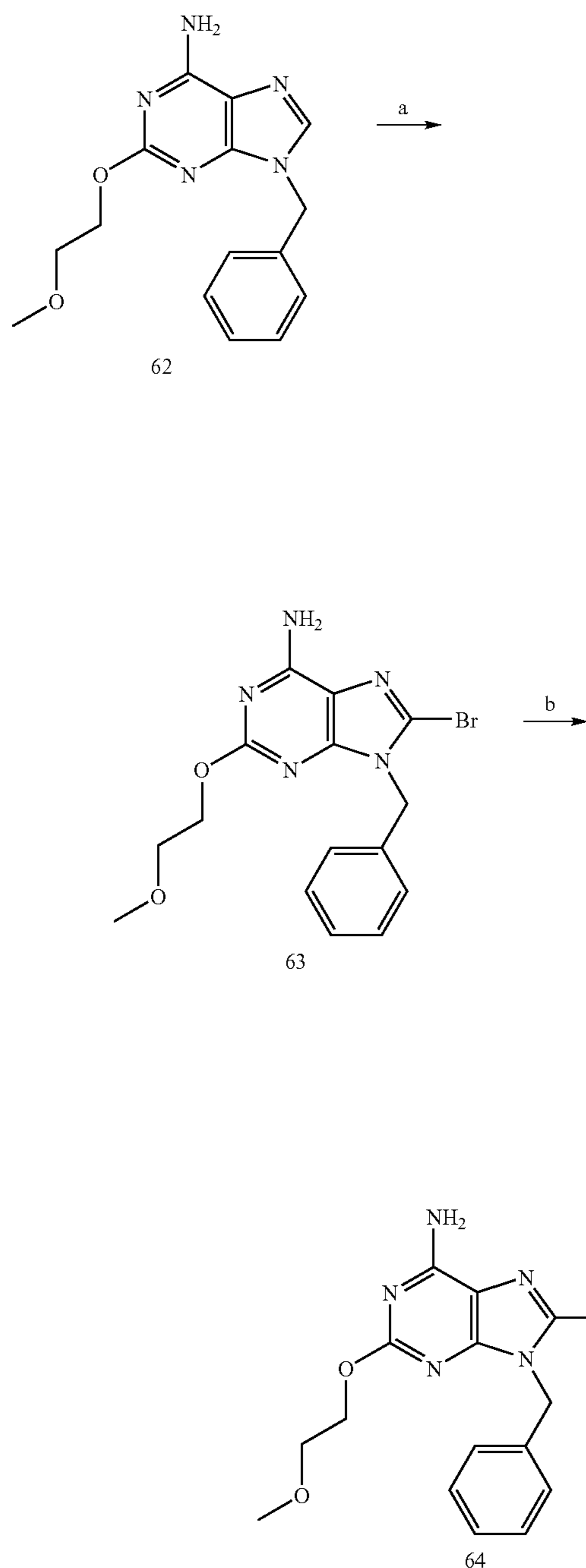
Scheme 16
