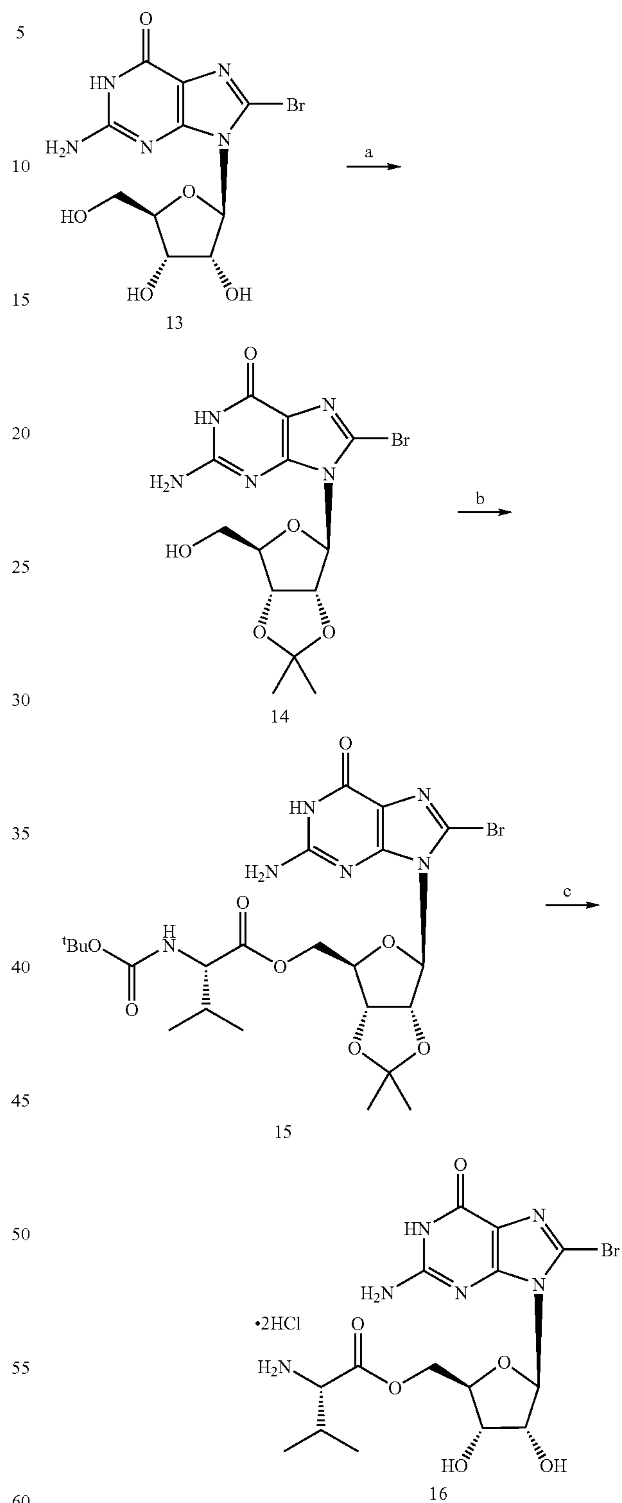
Scheme 4
