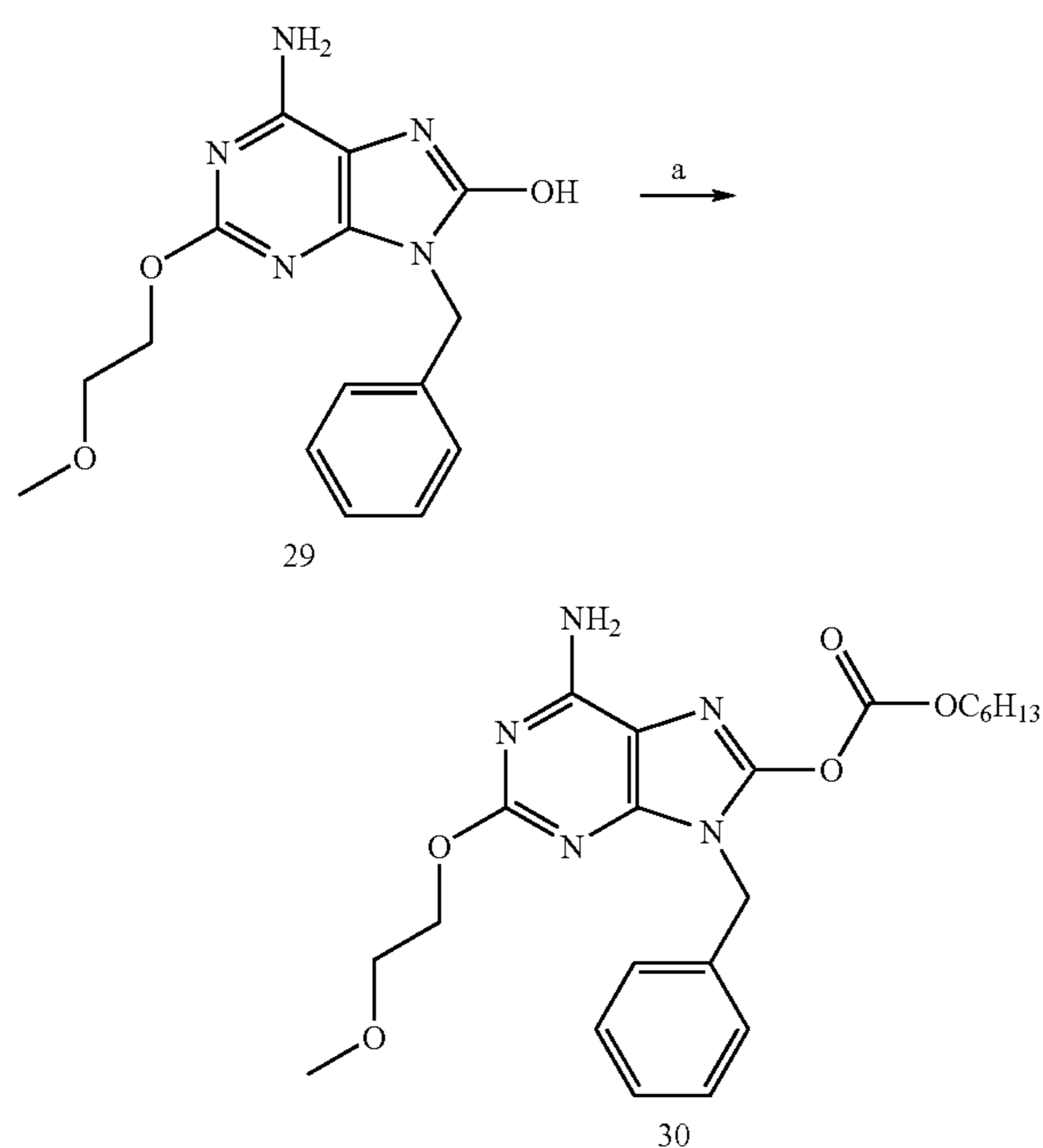
Scheme 8
