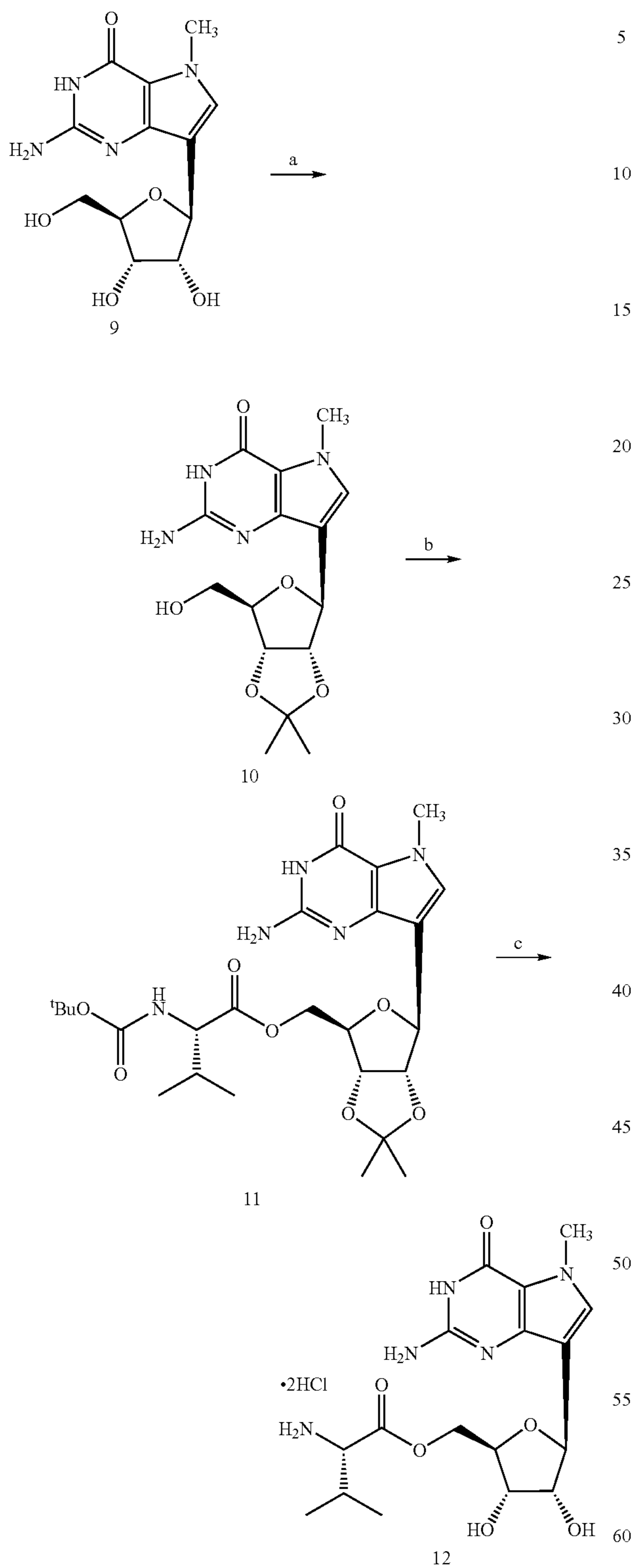
Scheme 3
