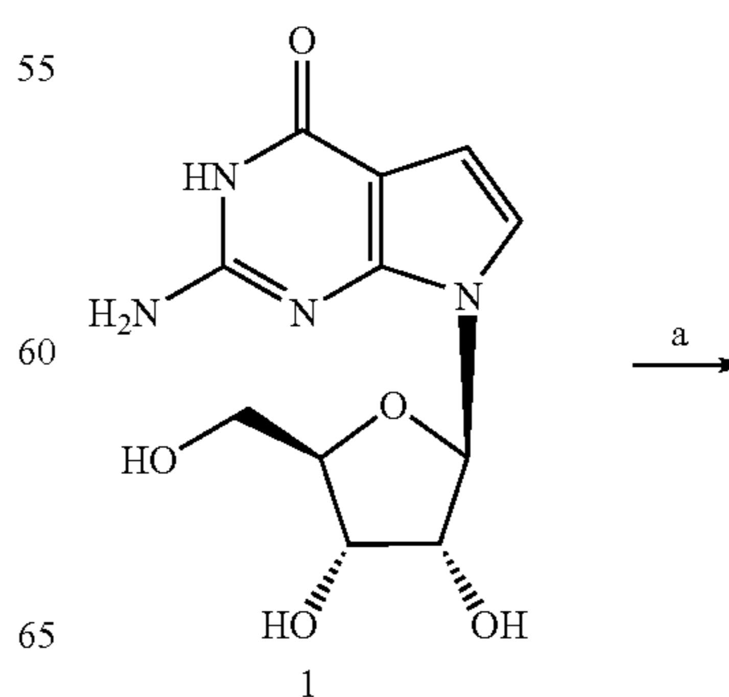
Scheme 1
