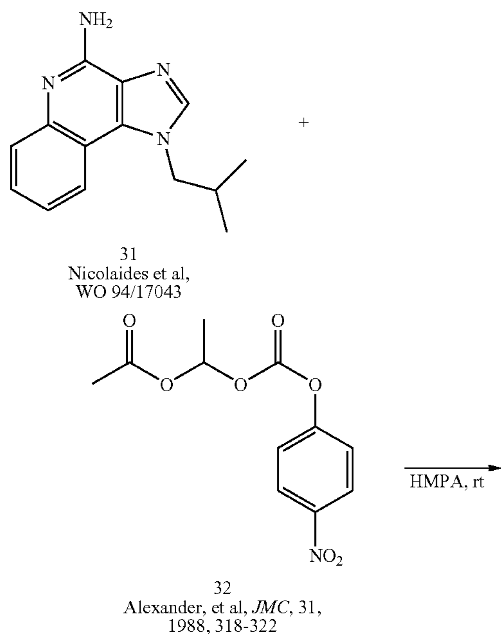
Scheme 9
