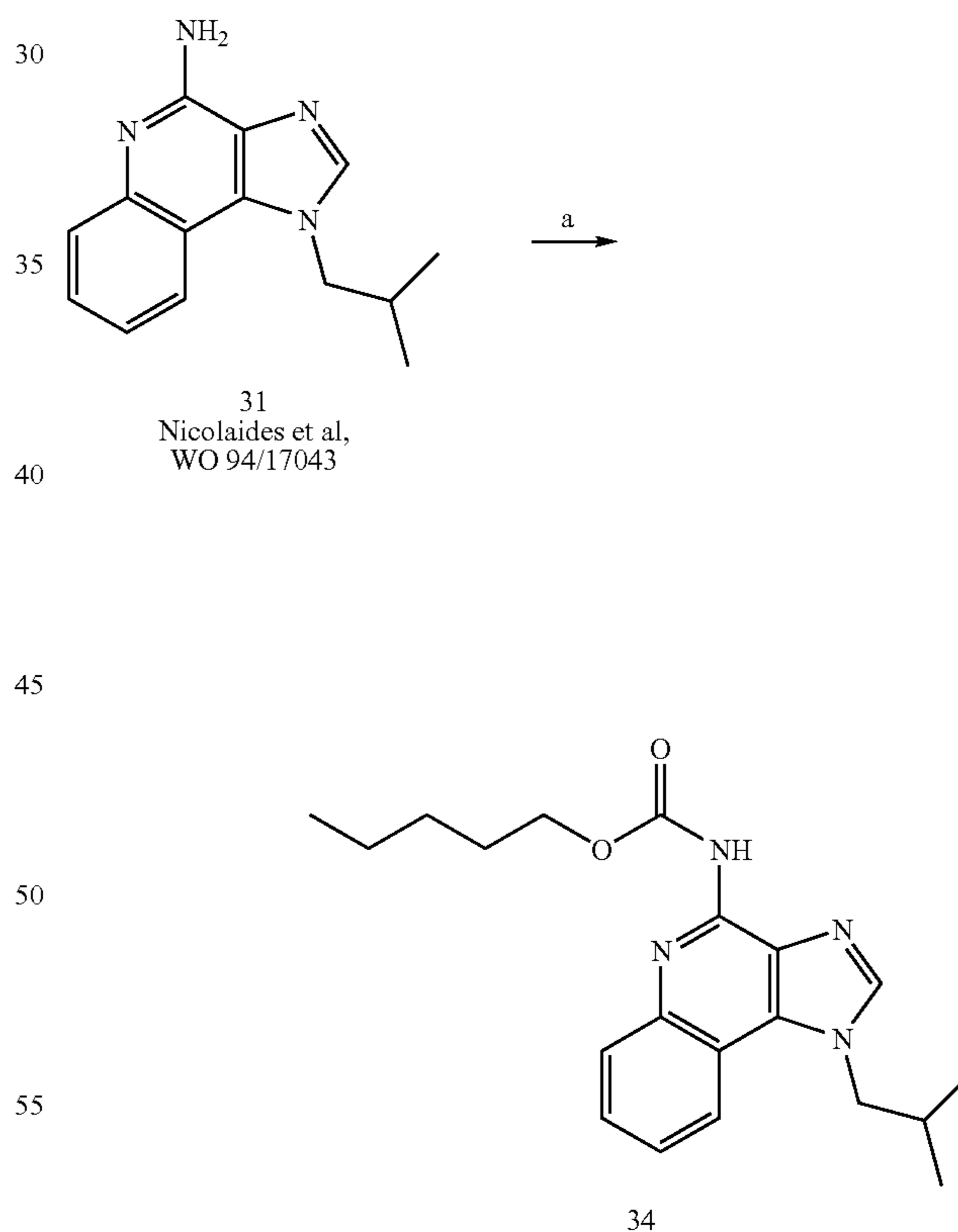
Scheme 10
