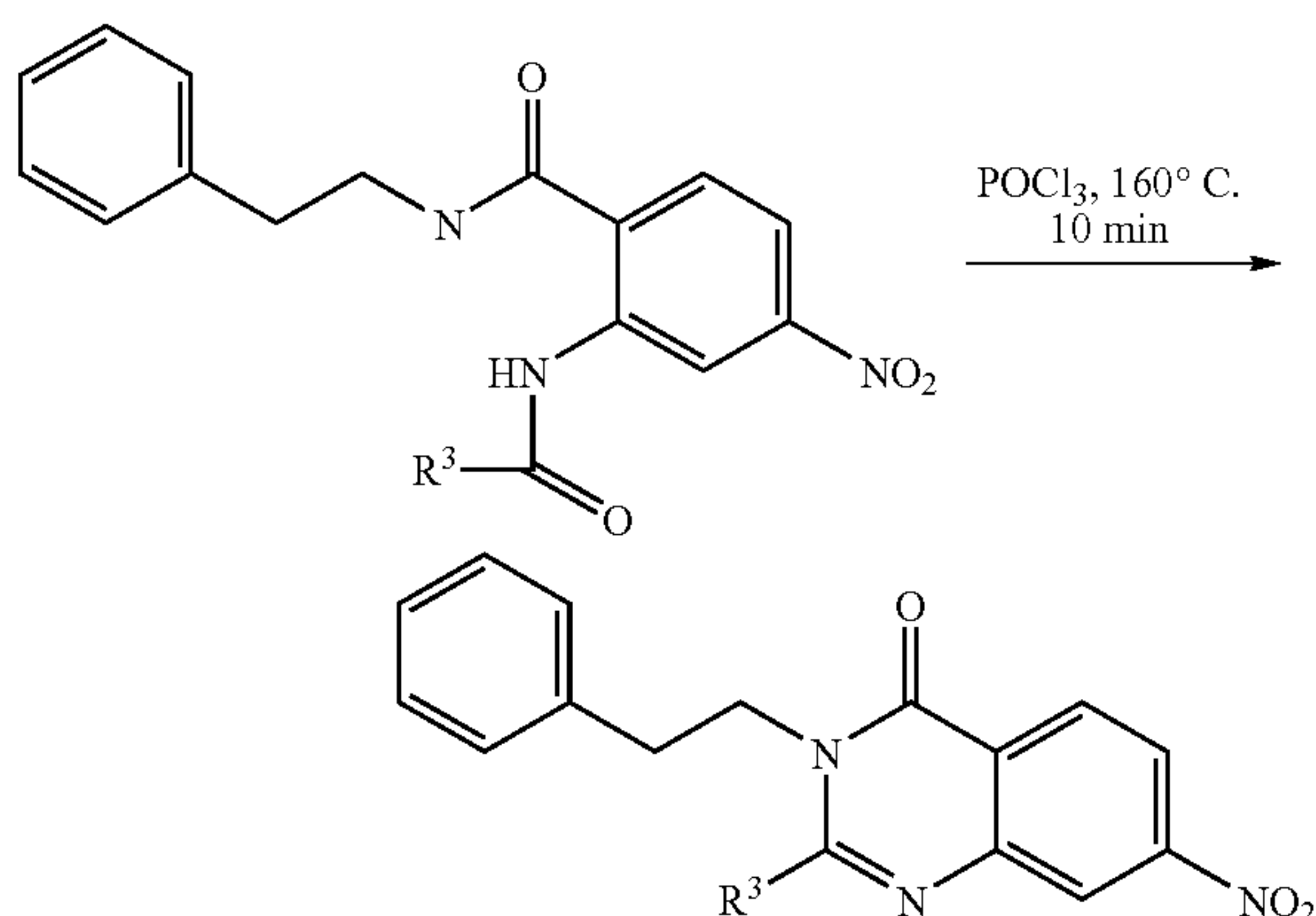
SCHEME 2c
