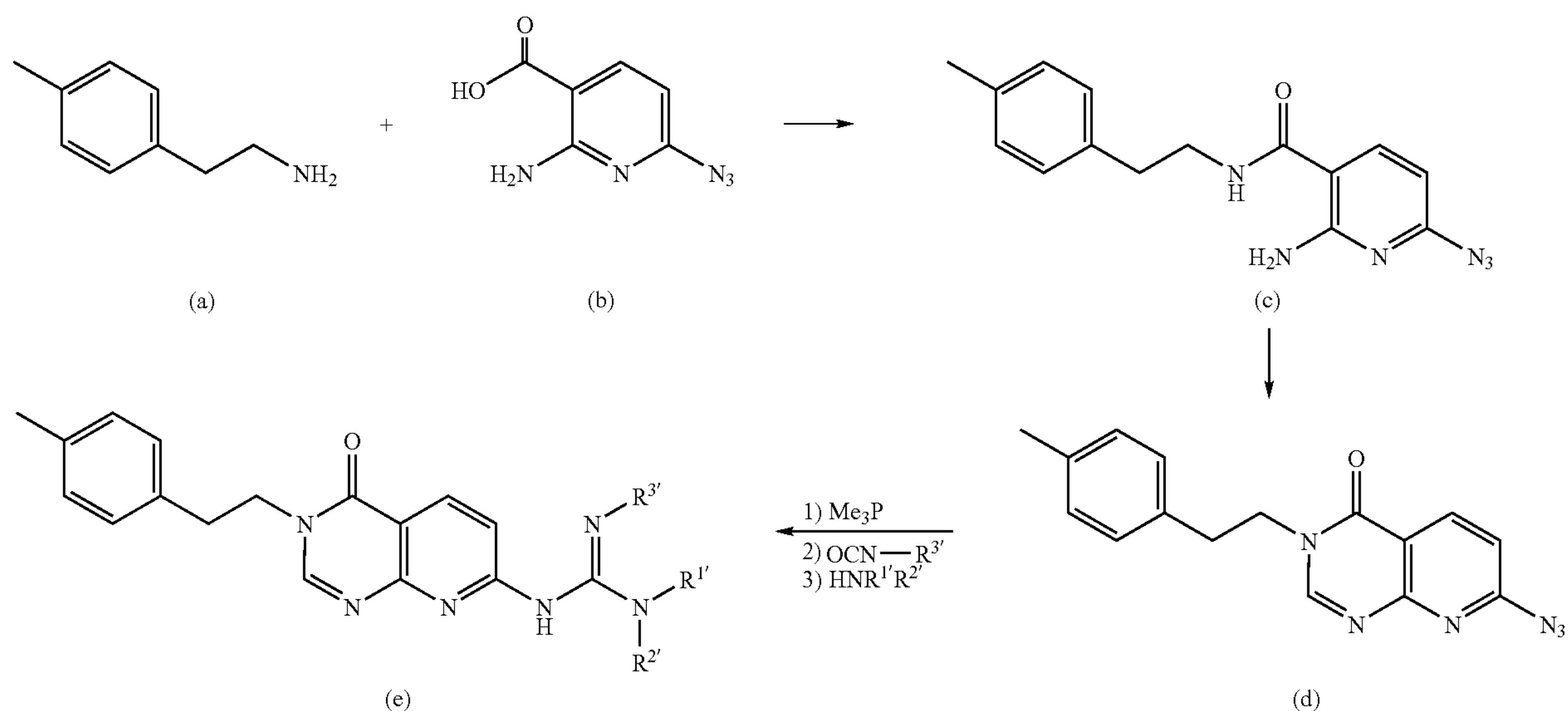
Scheme 1b
