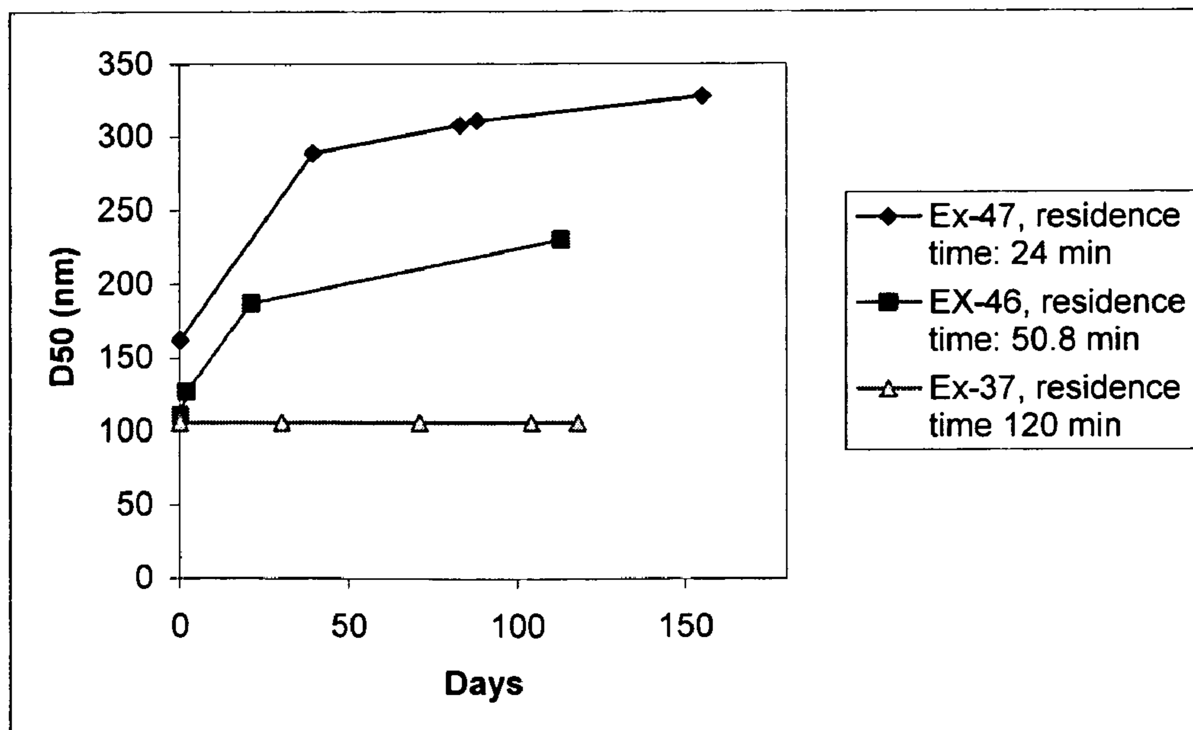
FIGURE 3. Stability plots (D50 vs time) of ganaxalone particles containing no complexing agent: ganaxalone particles without a complexing agent that were milled for less than 2 hours of milling residence time continued to increase gradually in size over a number of months, while the particles milled for more than 2 hours of residence time did not change over six months.
