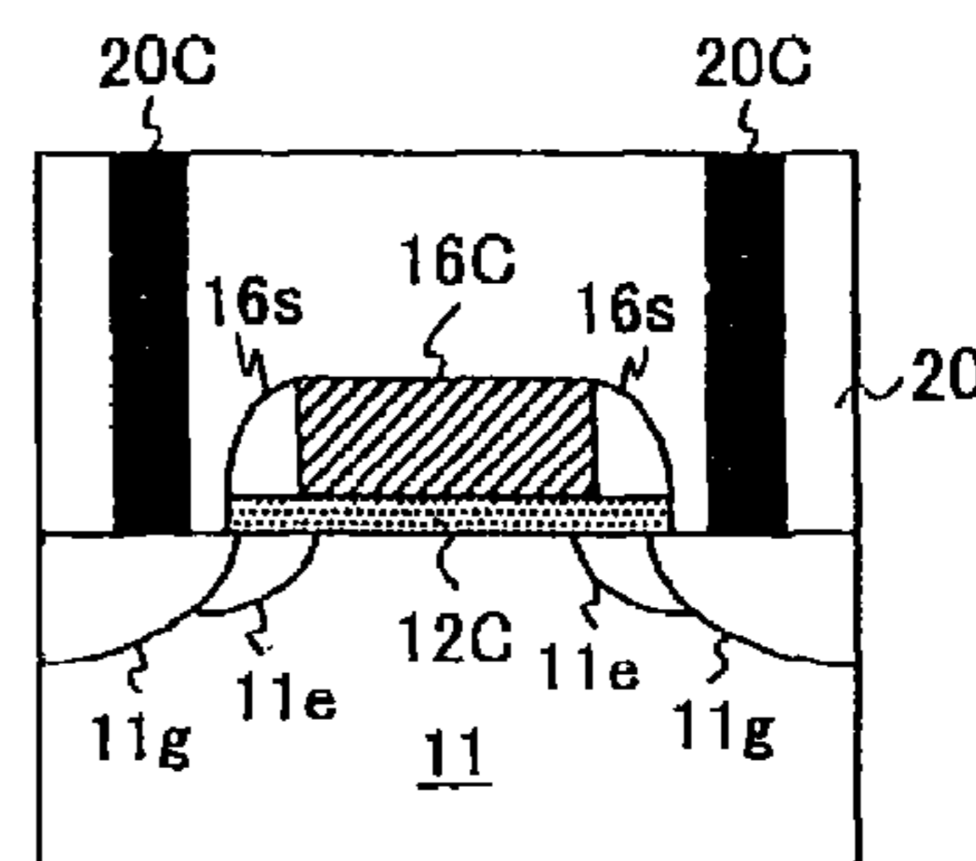
HIGH-VOLTAGE OPERATION TRANSISTOR C
