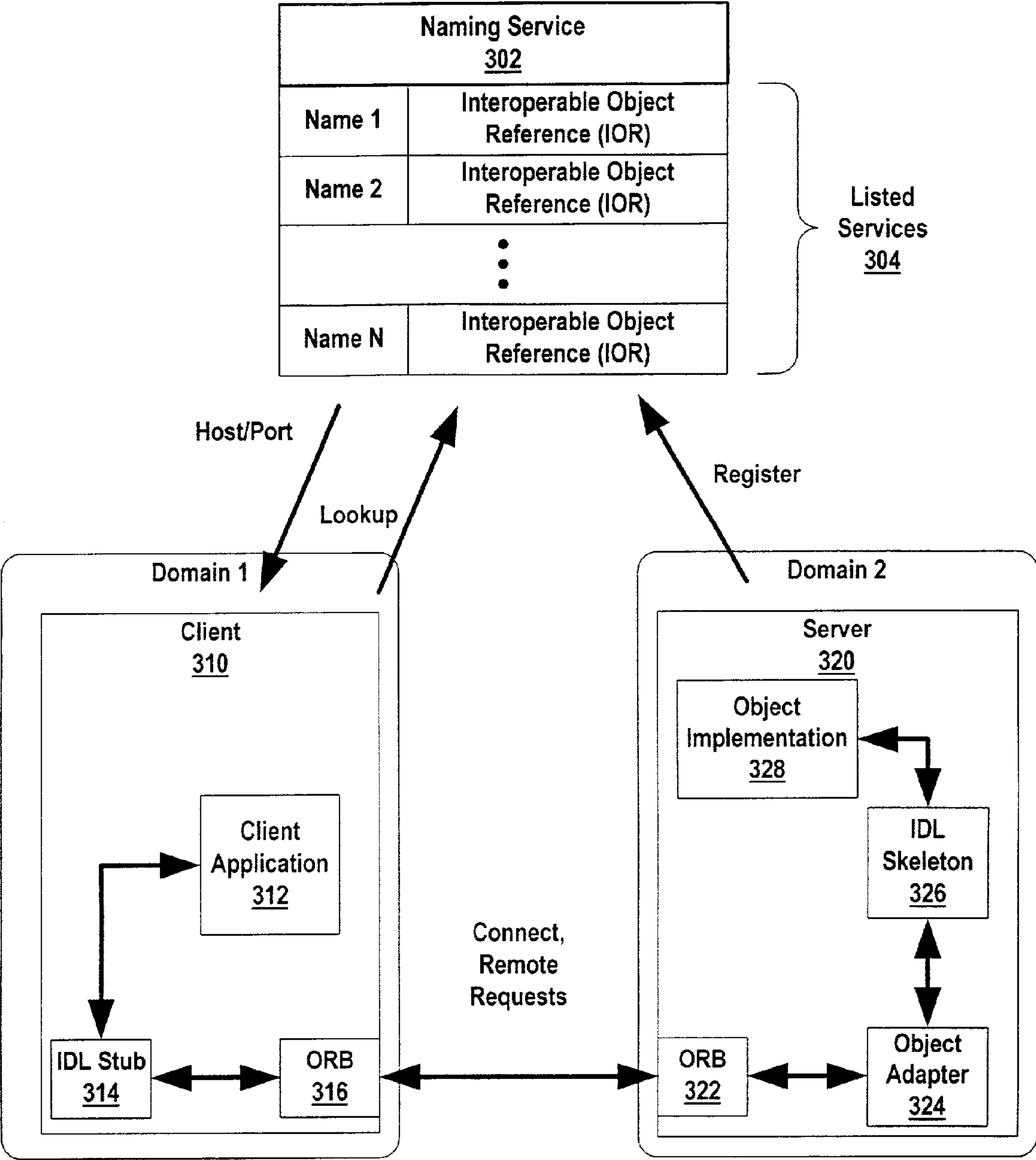
Corba Service Object Lookup Prior Art
