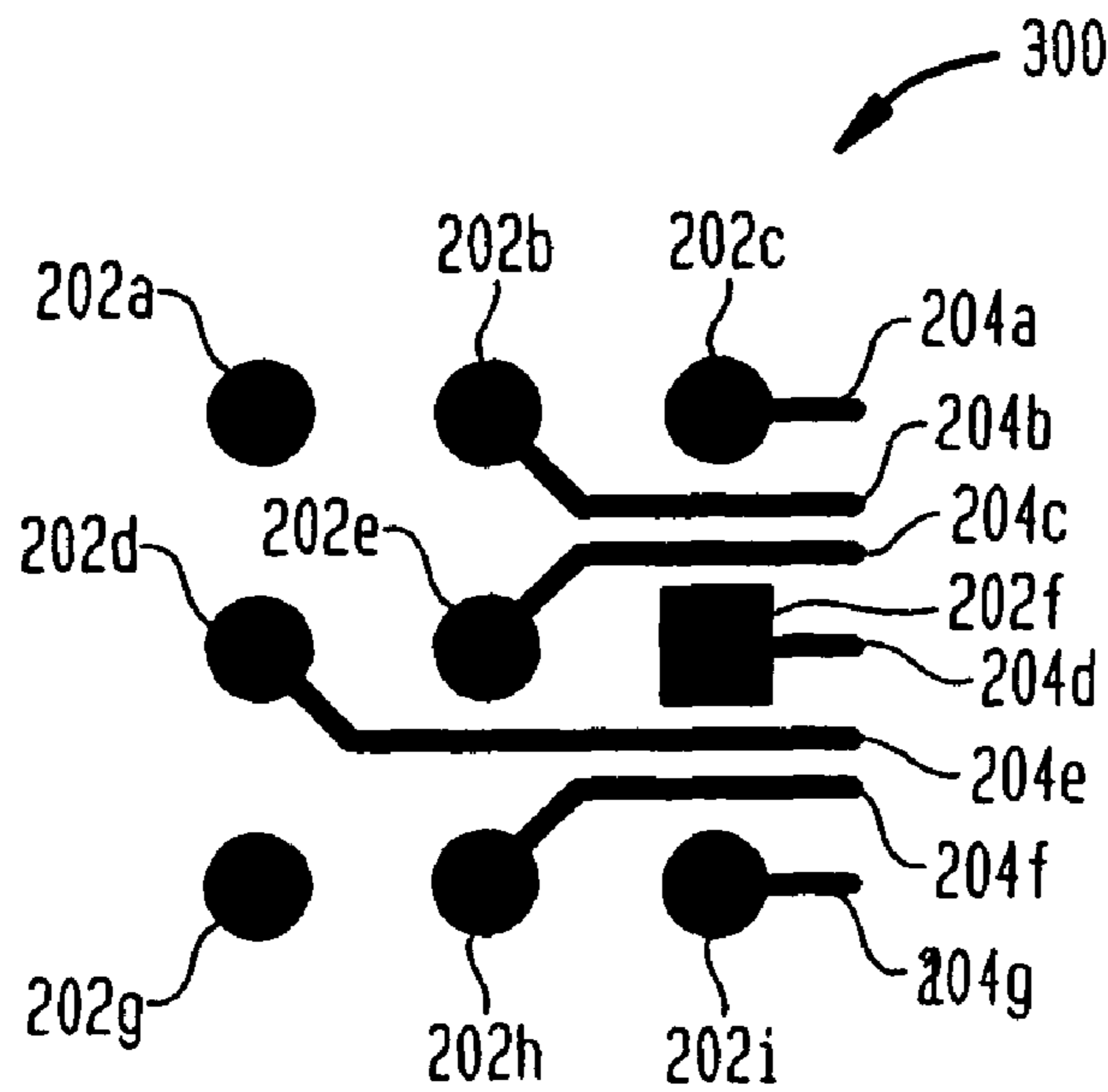
FIG. 3 PRIOR ART
