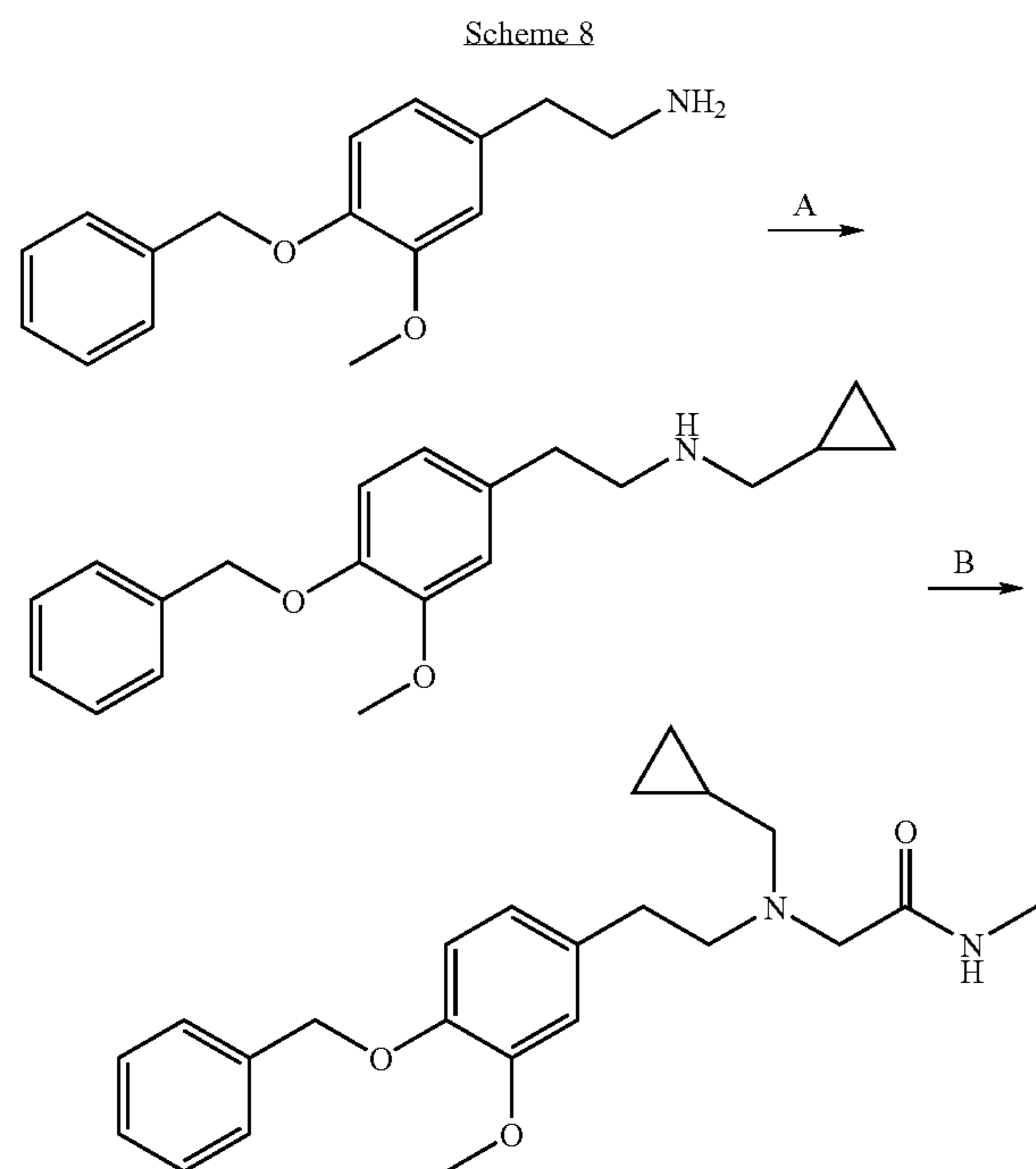
Step A [2-(4-Benzyloxy-3-methoxy-phenyl)-ethyl]- (cyclopropylmethyl)amine
