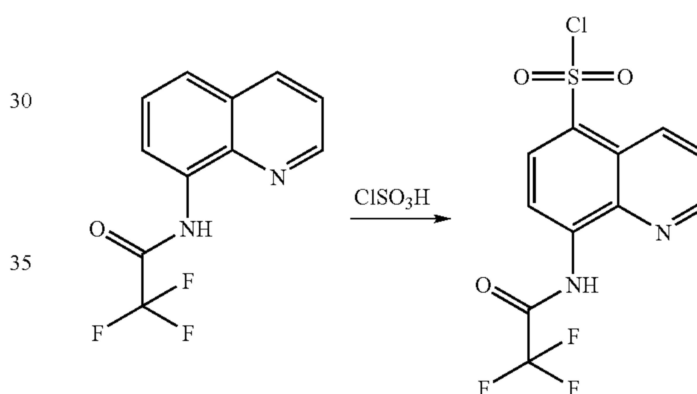
8-(2,2,2-Trifluoroacetamido)quinoline-5-sulfonyl chloride
