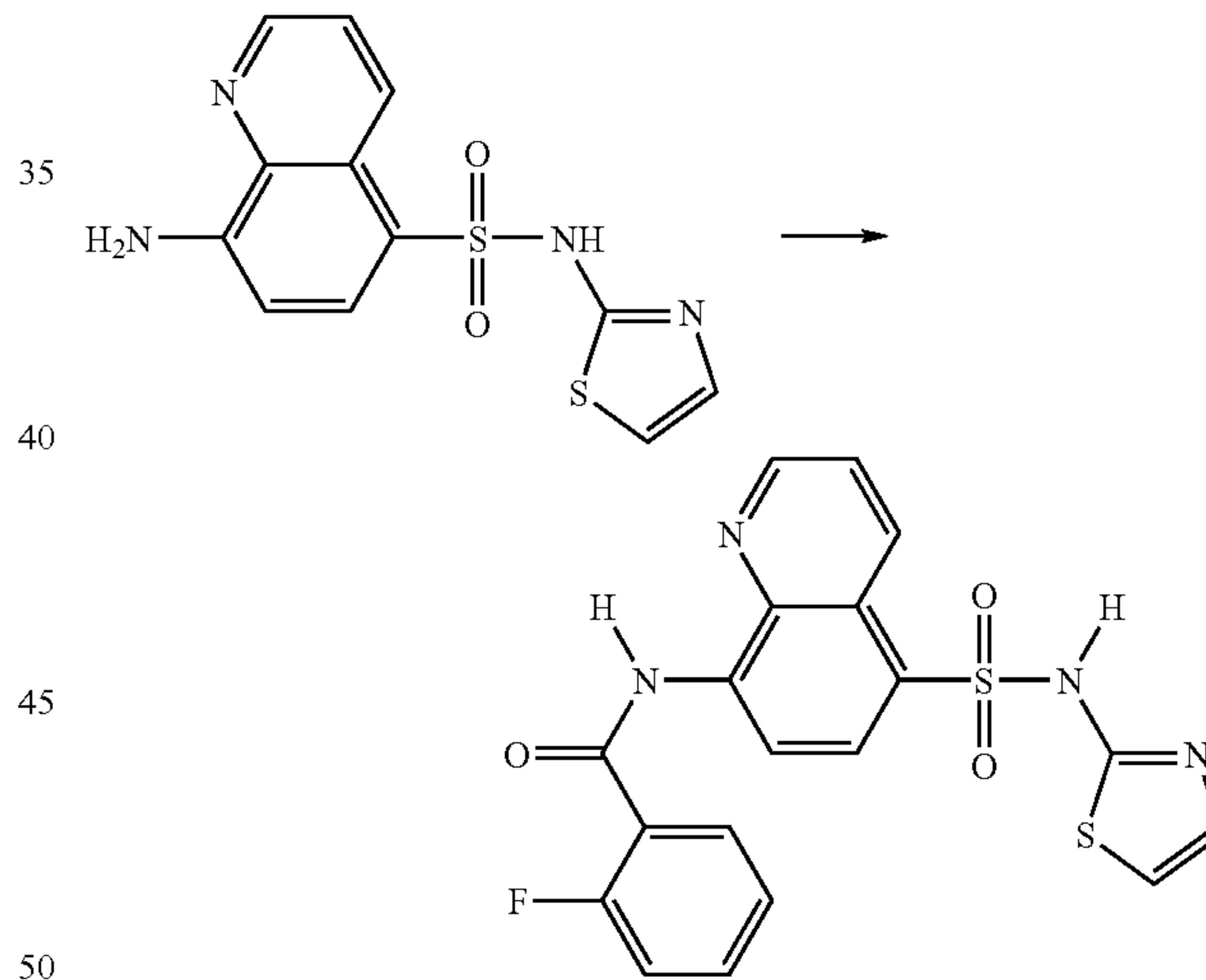
2-Fluoro-N-[5-(thiazol-2-ylsulfamoyl)-Quinolin-8-yl]-benzamide
