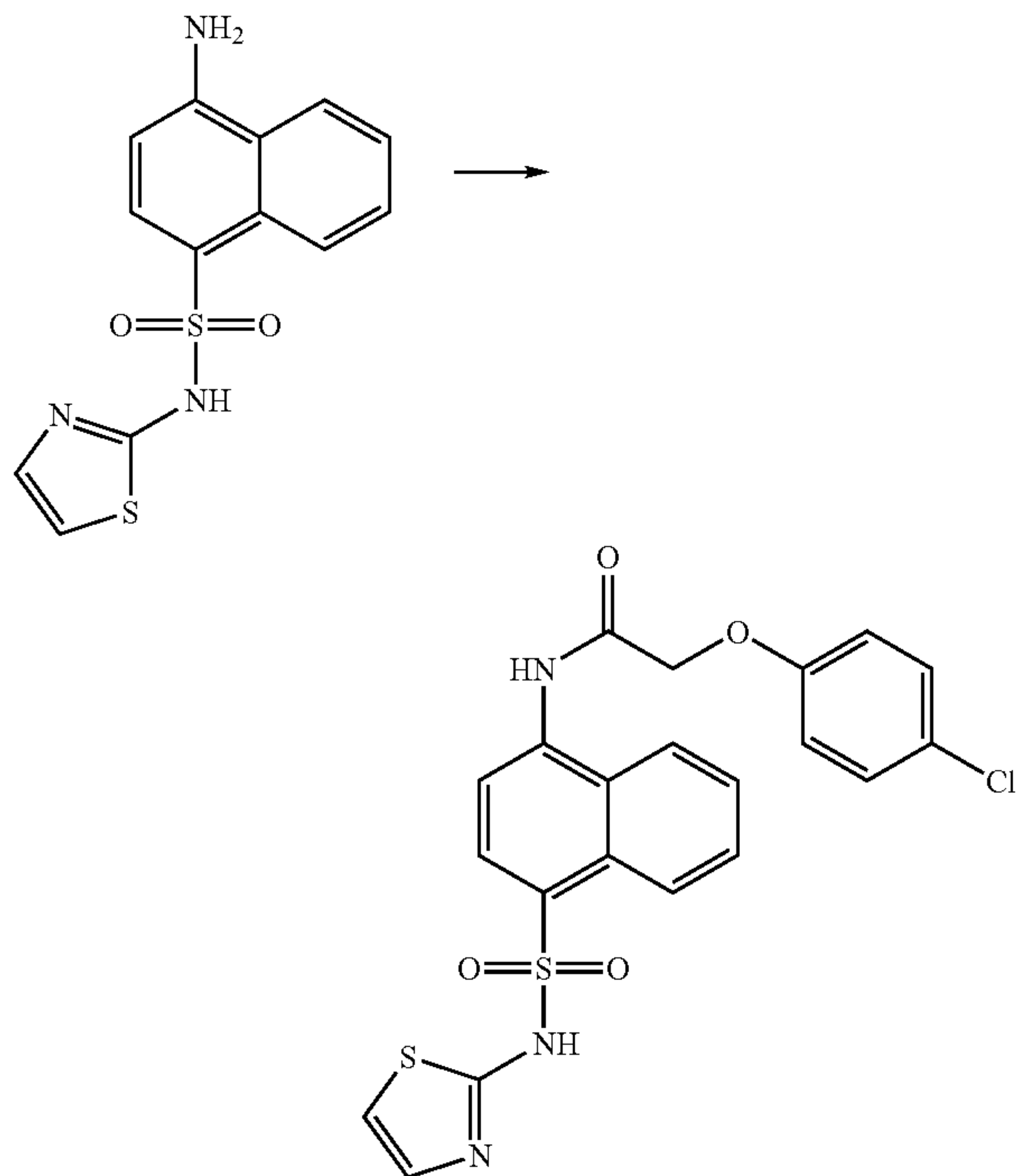
2-(4-Chloro-phenoxy)-N-[4-(thiazol-2-ylsulfamoyl)-naphthalen-1-yl]-acetamide
