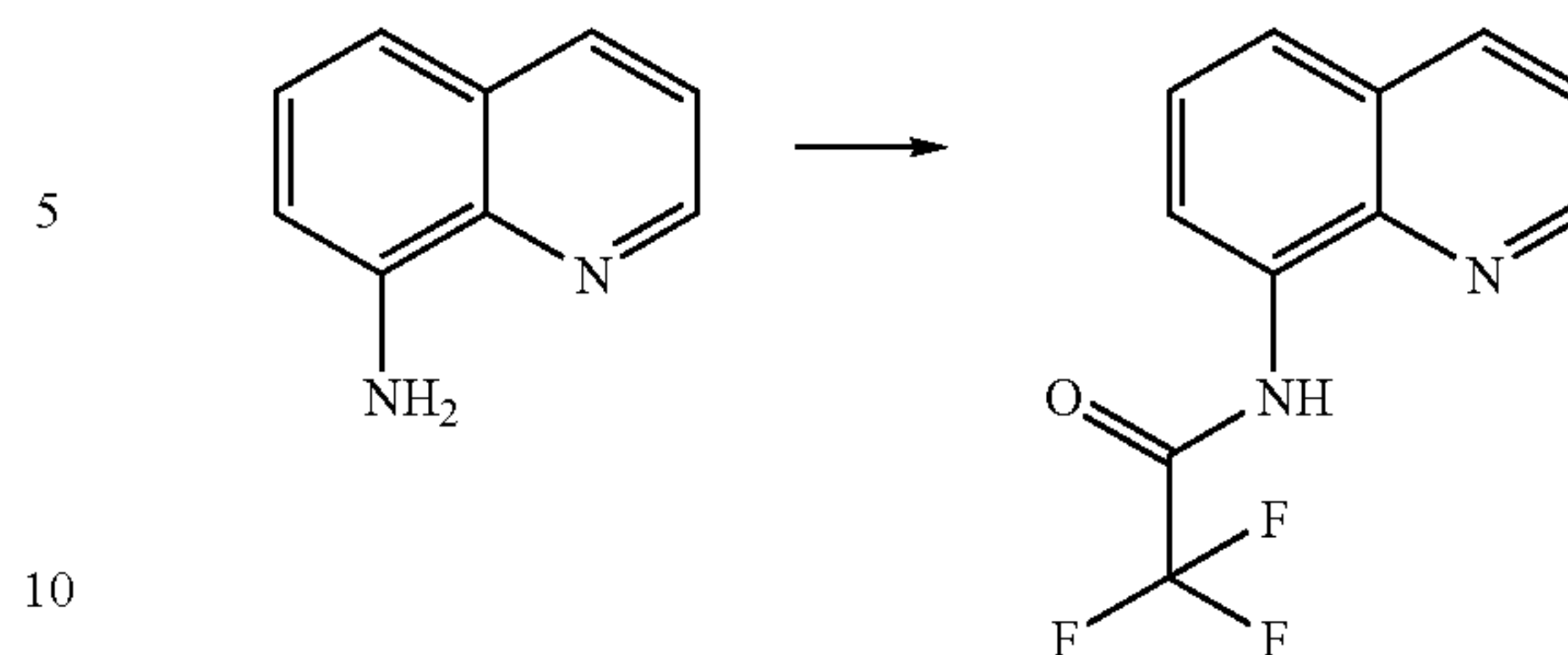
2,2,2-Trifluoro-N-(quinolin-8-yl)acetamide
