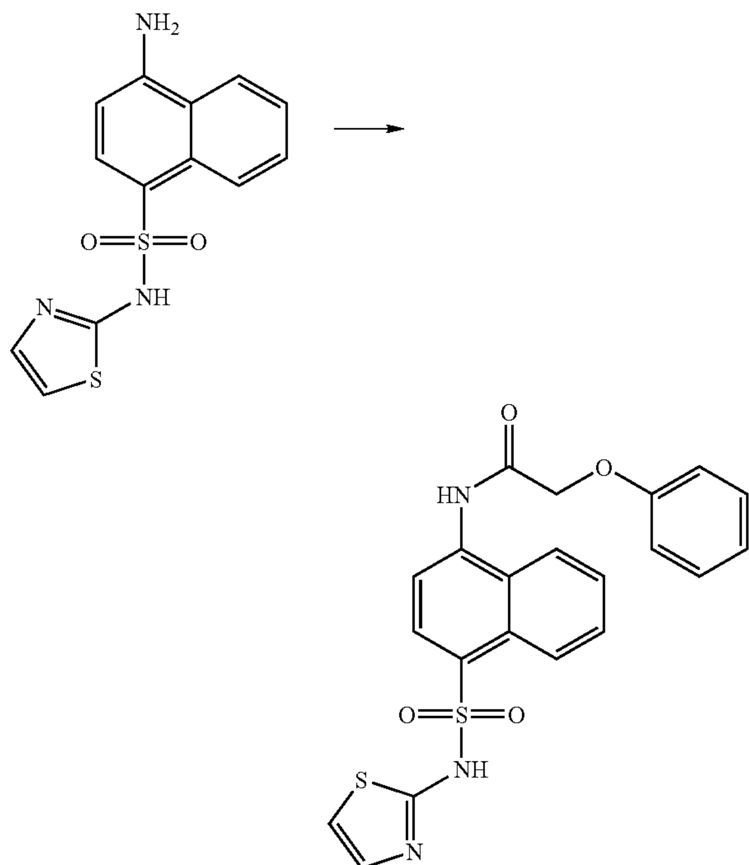
2-Phenoxy-N-[4-(thiazol-2-ylsulfamoyl)-naphthalen-1-yl]-acetamide
