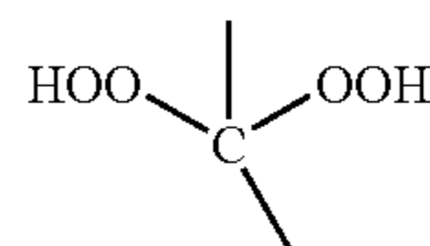
2,2-dihydroperoxypropane
