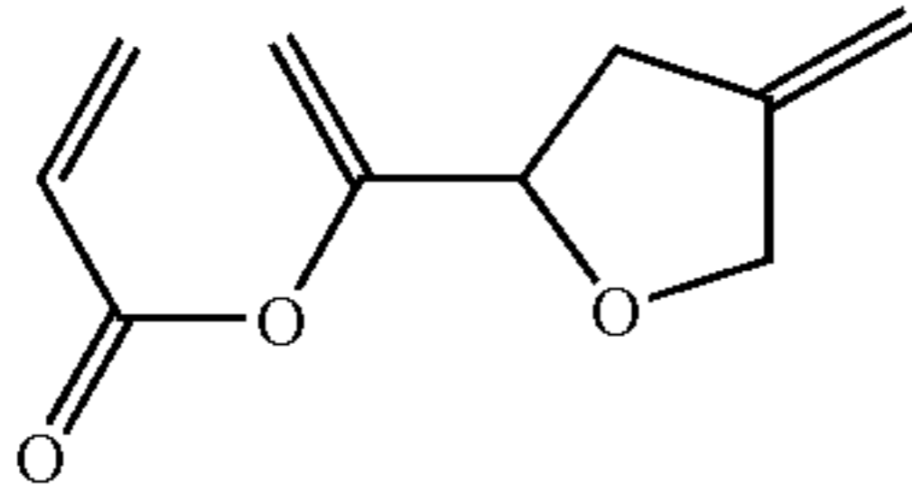
1-(tetrahydro-4-methylenefuran-2-yl)vinyl acrylate
