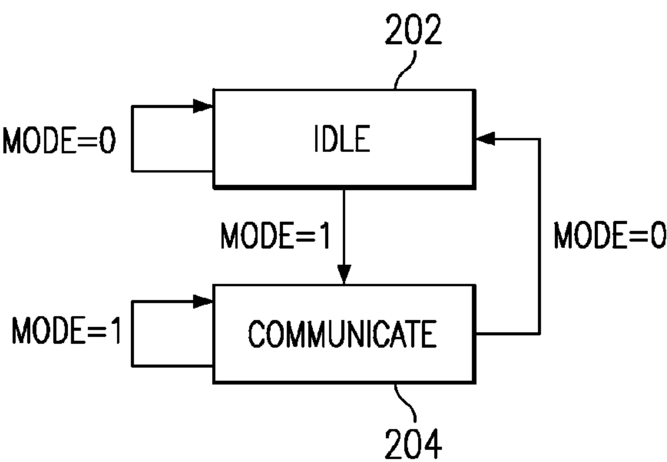
FIG. 2 (PRIOR ART)
