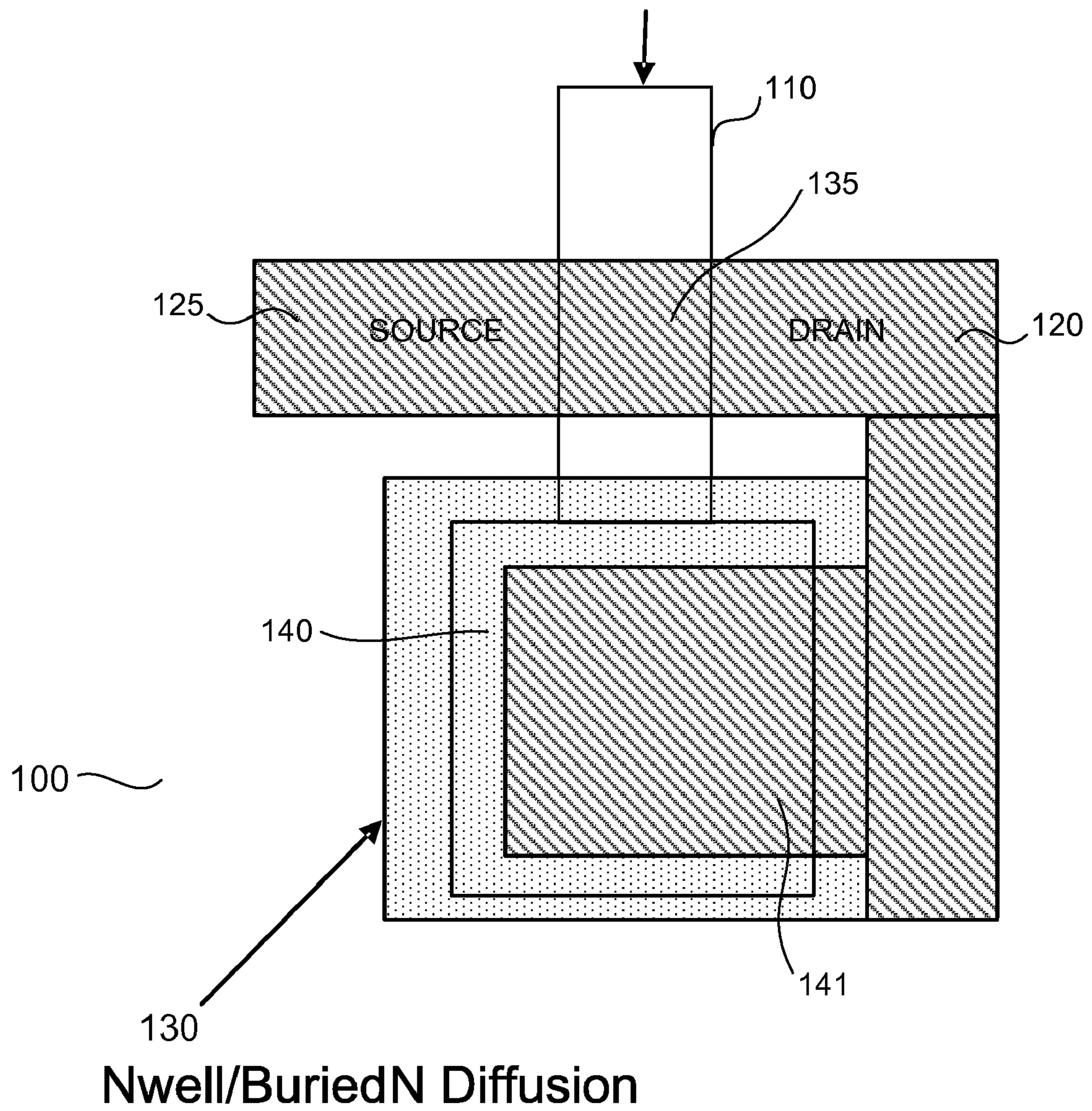
FIG. 1 Floating Gate
