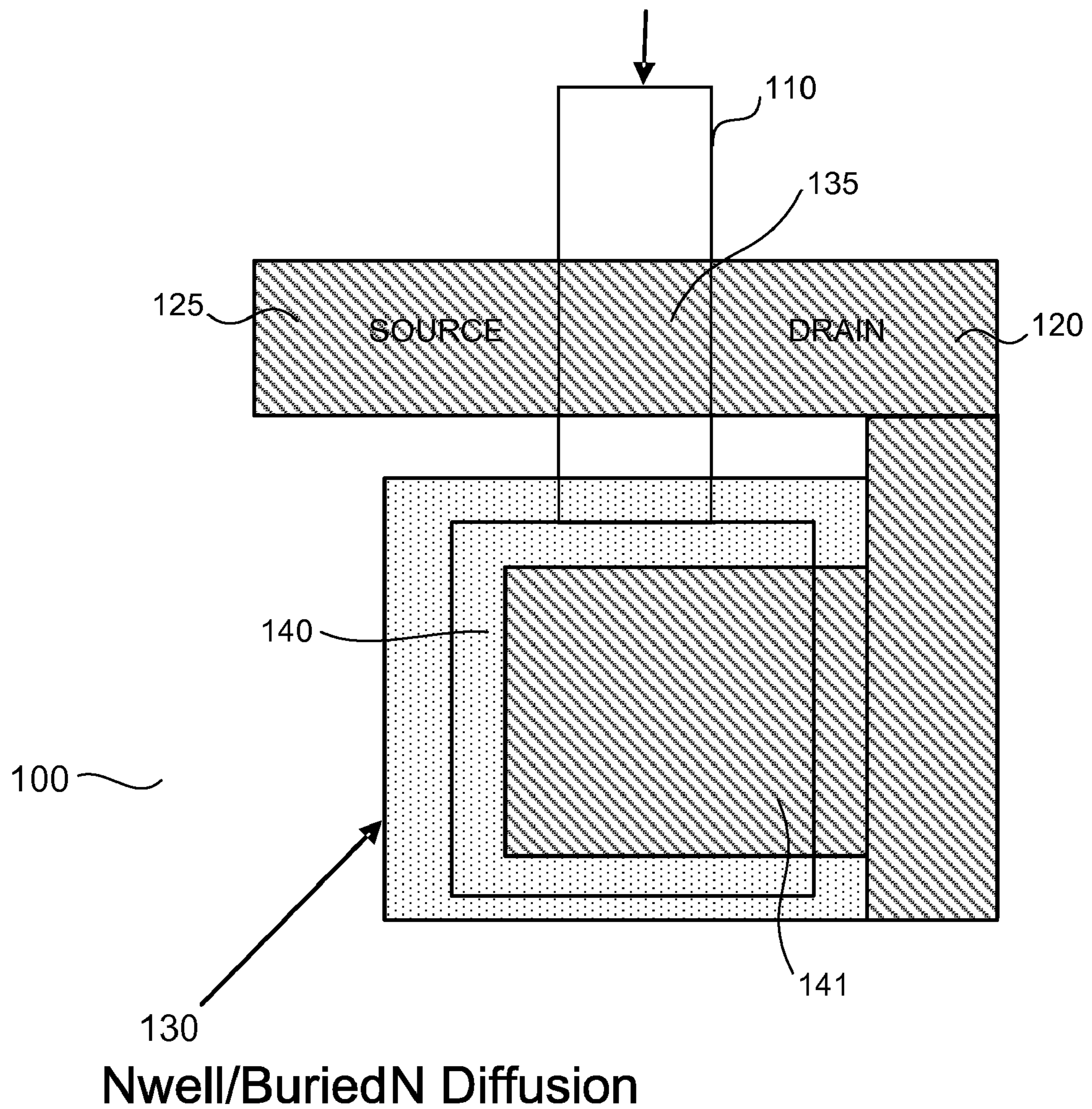
FIG. 1 Floating Gate
