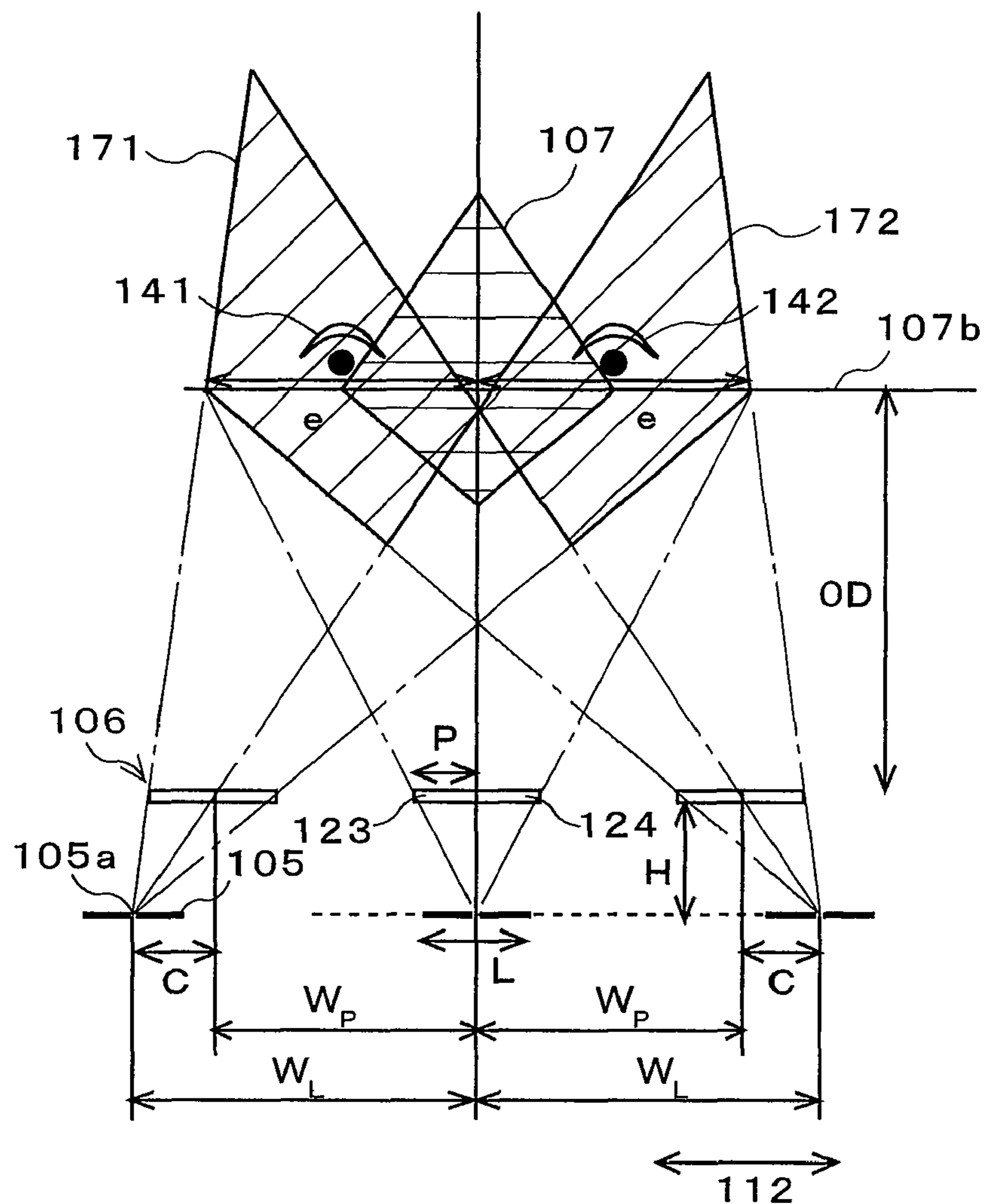
FIG. 7 (PRIOR ART)
