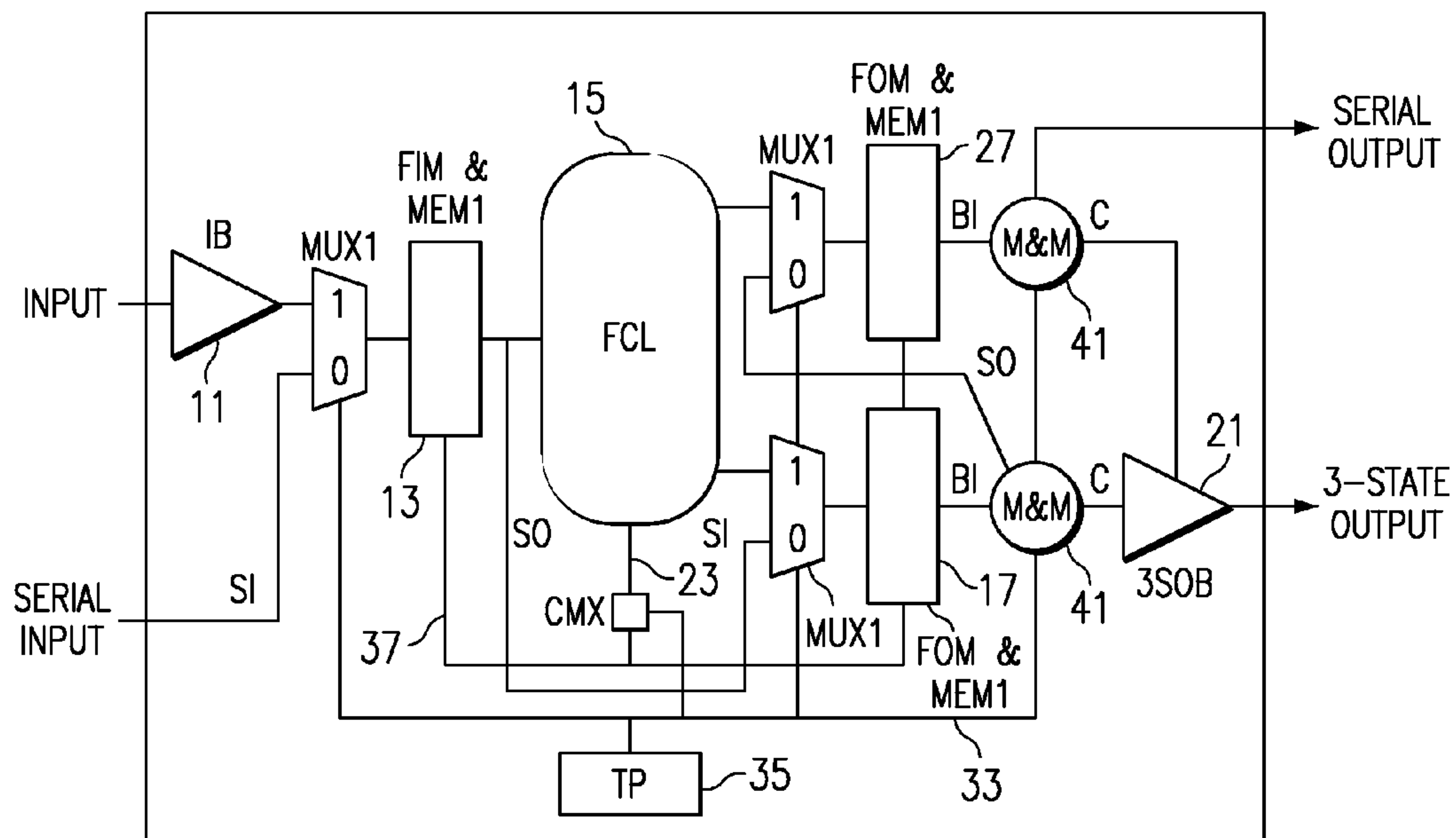
FIG. 6 (PRIOR ART)
