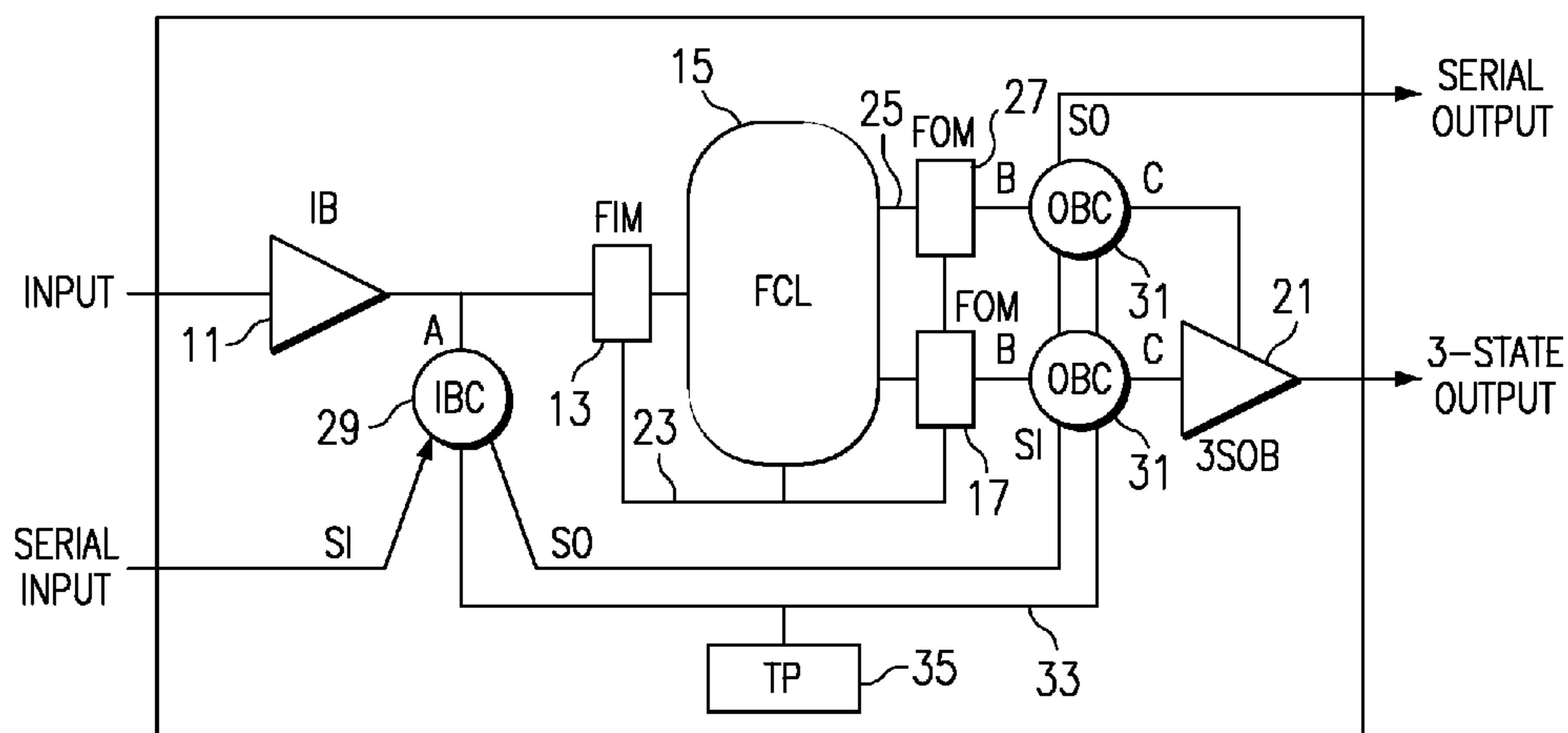
FIG. 4 (PRIOR ART)
