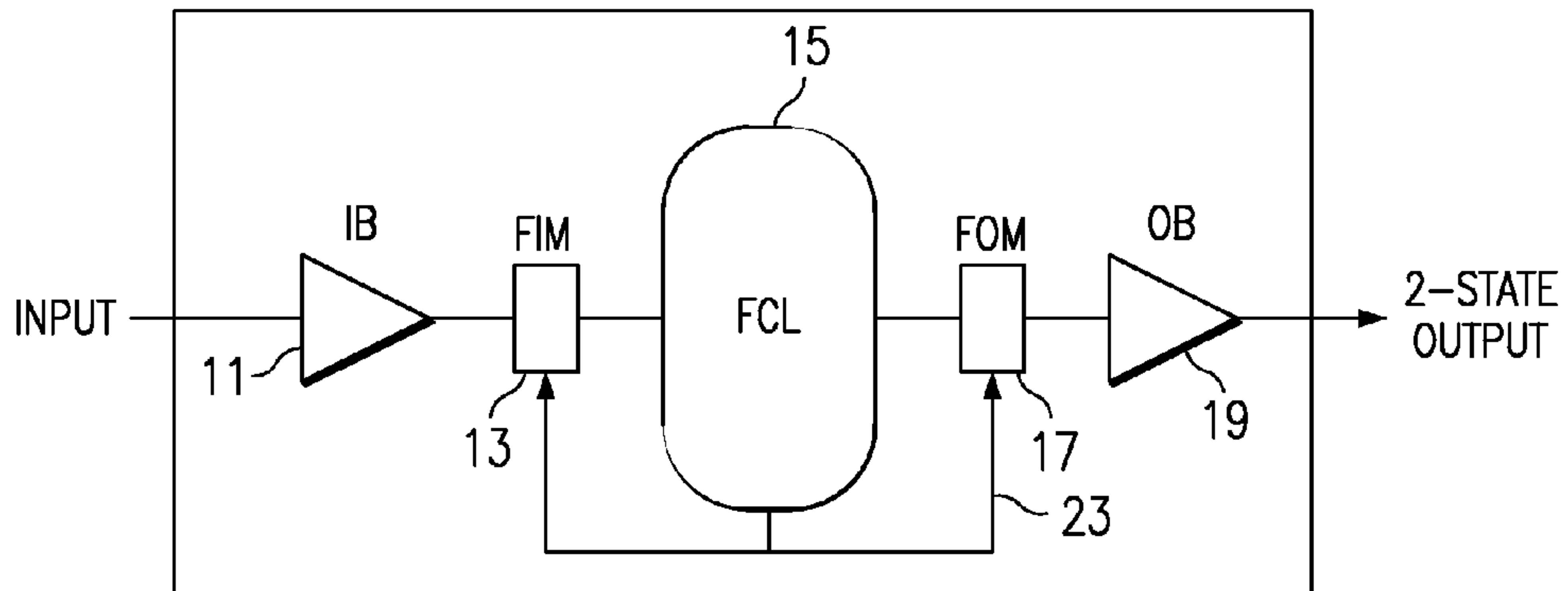
FIG. 1 (PRIOR ART)
