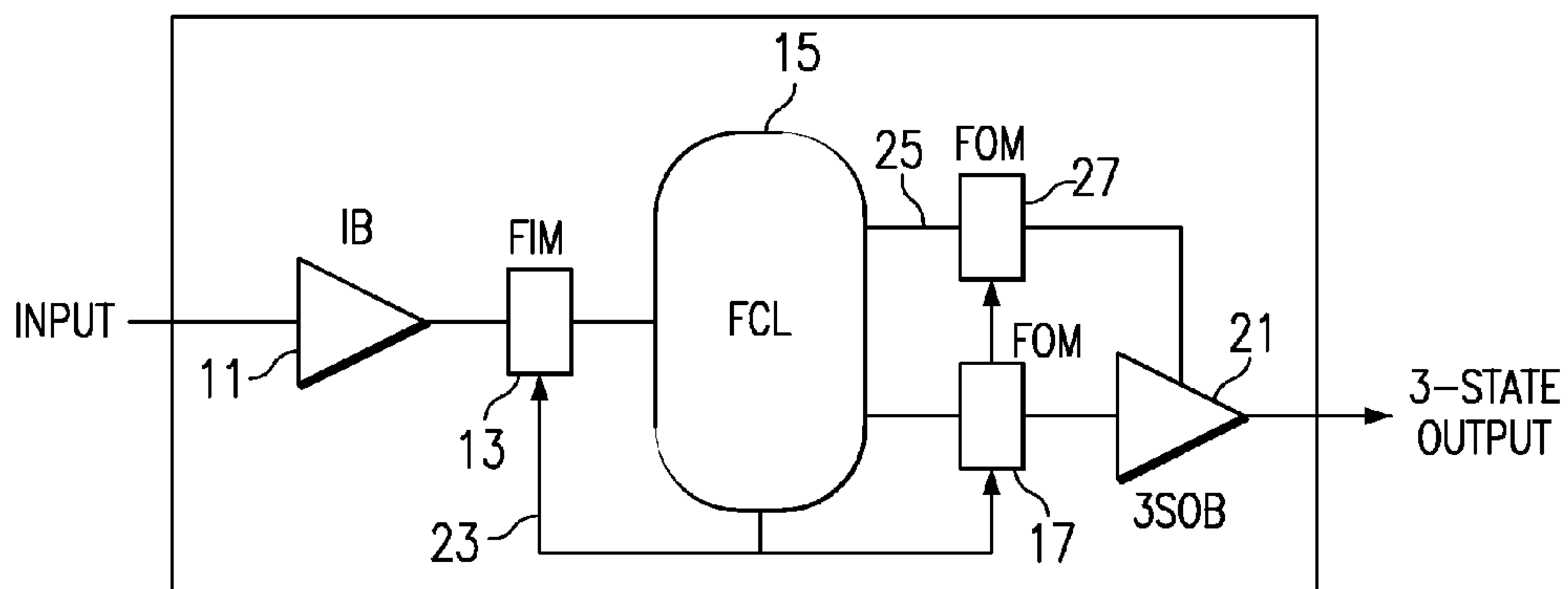
FIG. 2 (PRIOR ART)
