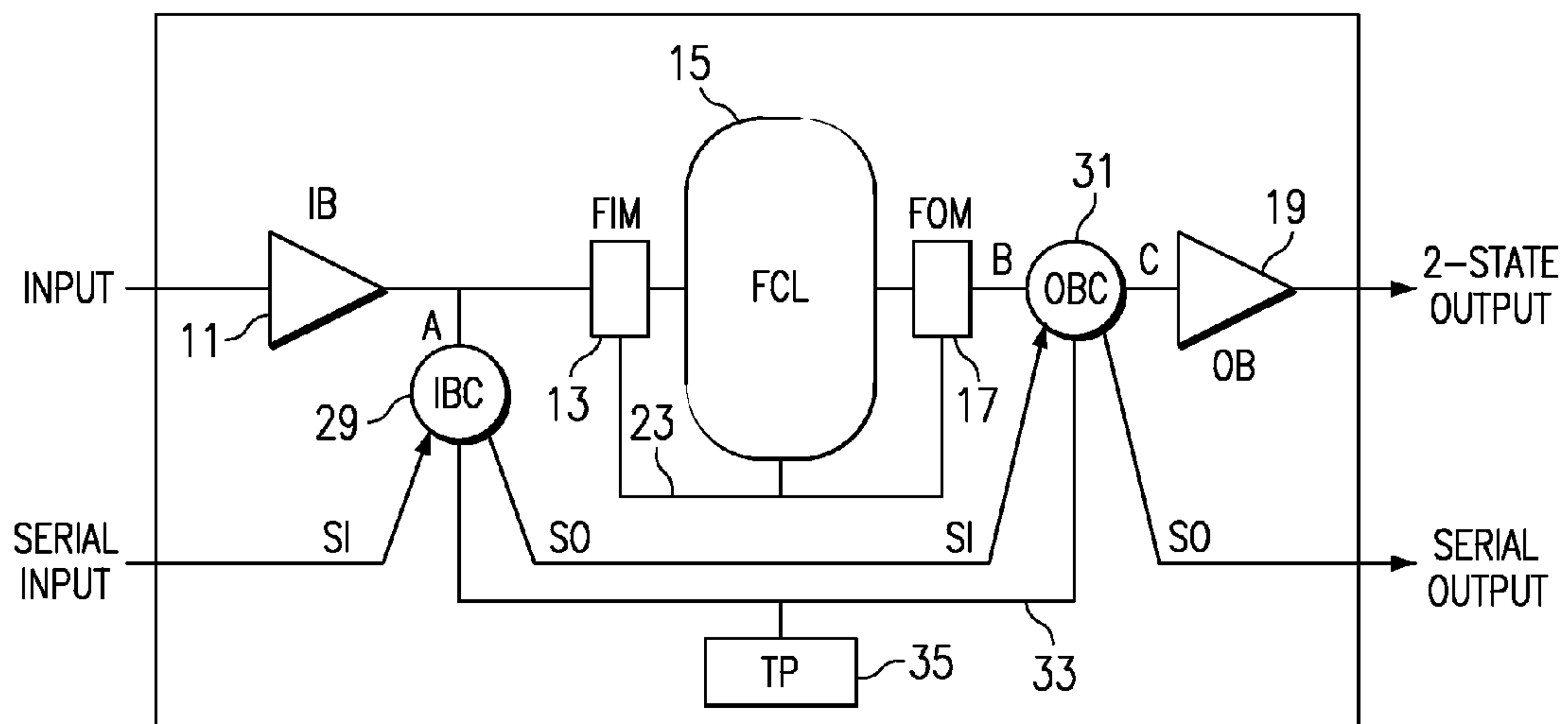
FIG. 3 (PRIOR ART)
