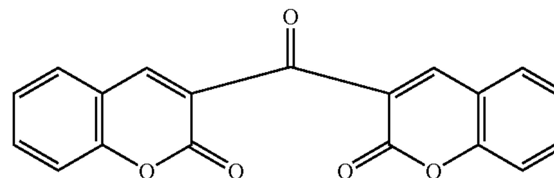
Chemical formula 1
