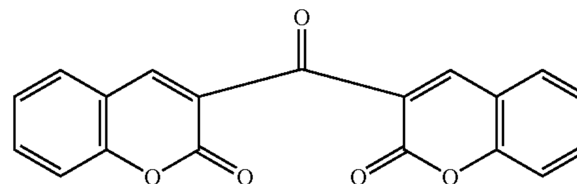
Chemical formula 1
