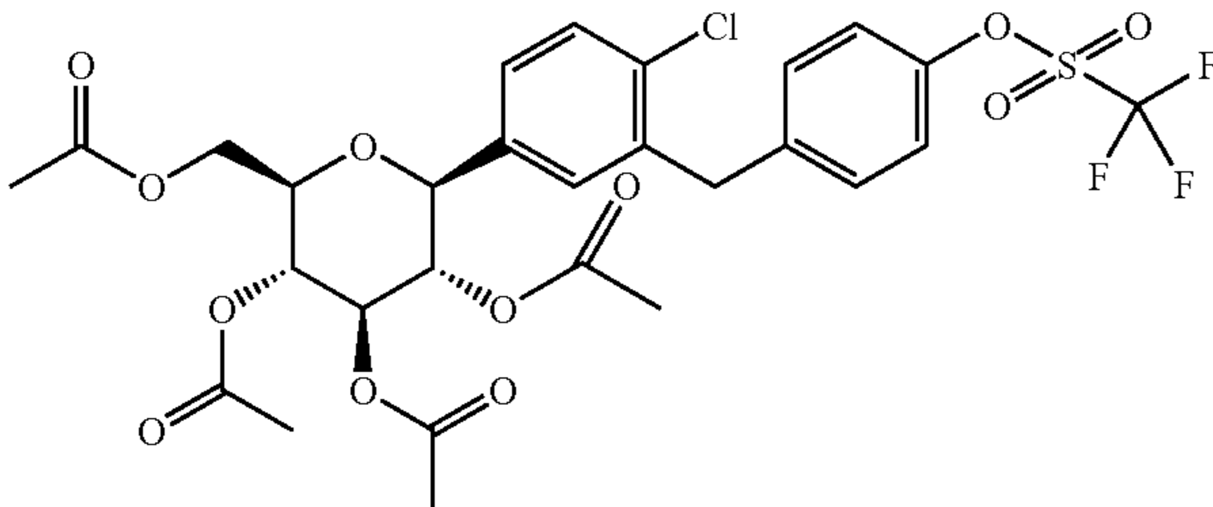
1-chloro-4-(2,3,4,6-tetra-O-acetyl-β-D-glucopyranos-1-yl)-2-[4-(trifluoromethylsulphonyloxy)-benzyl]-benzene
