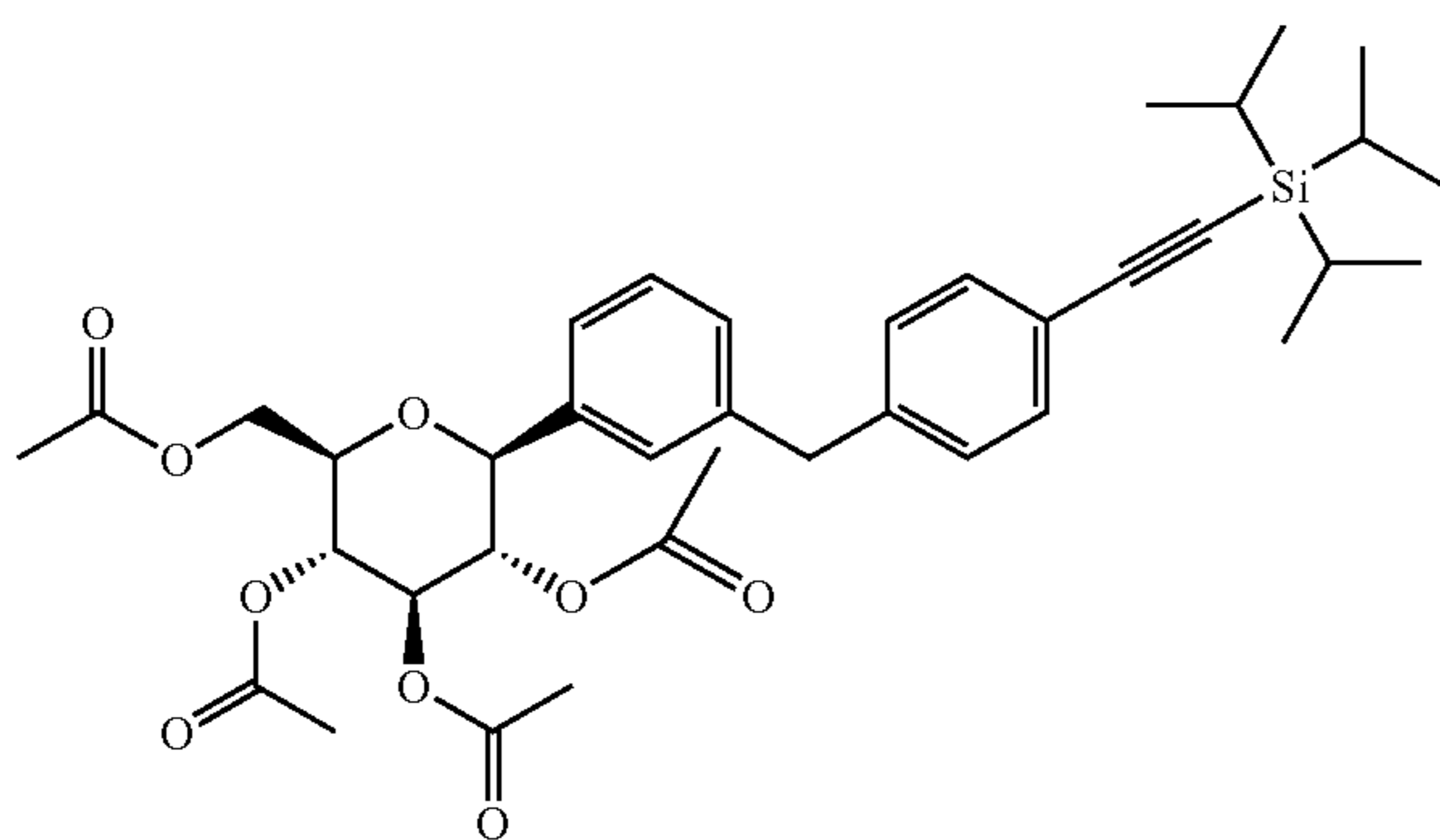
1-(2,3,4,6-Tetra-O-acetyl- \beta -D-glucopyranos-1-yl)-3-(4-triisopropylsilylethynyl-benzyl)-benzene
