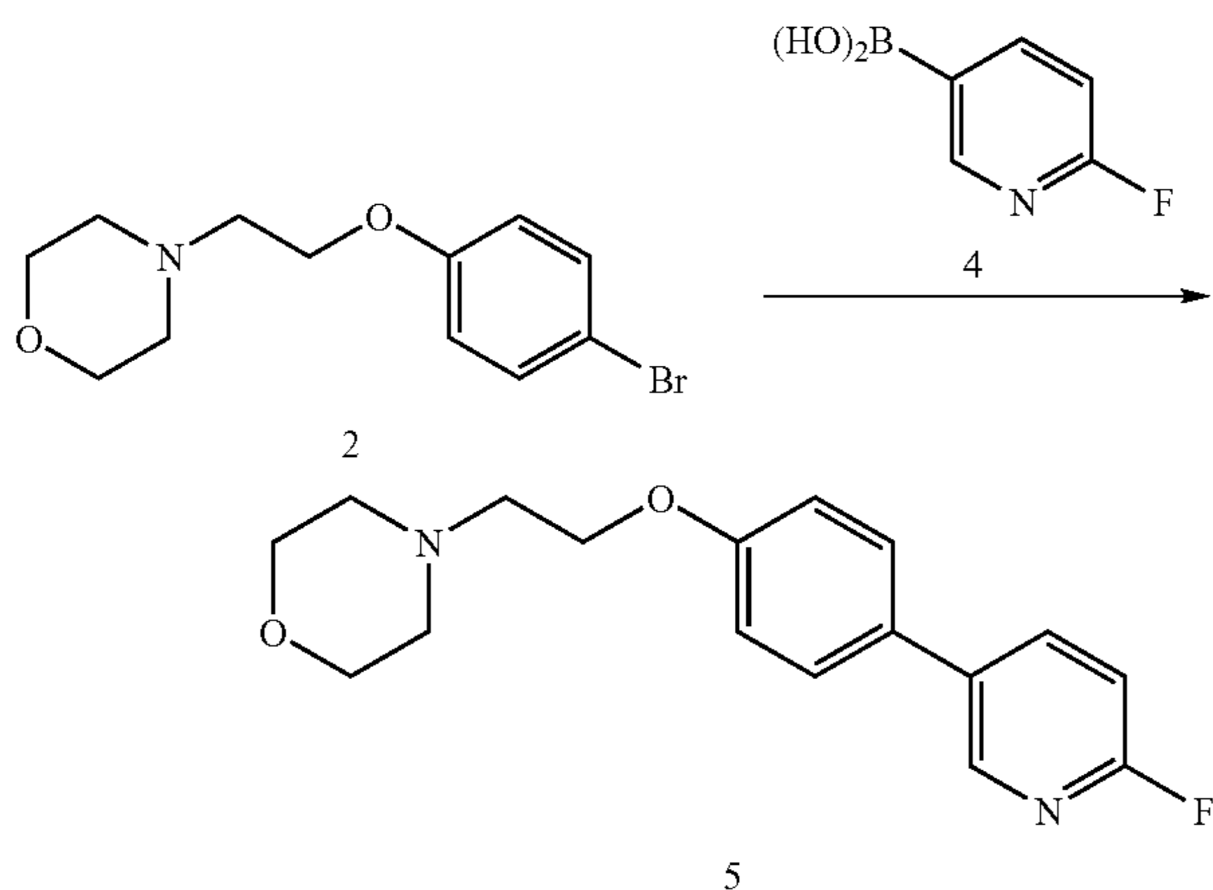
Preparation of 4-(2-(4-(6-fluoropyridin-3-yl)phenoxy)ethyl)morpholine (5)
