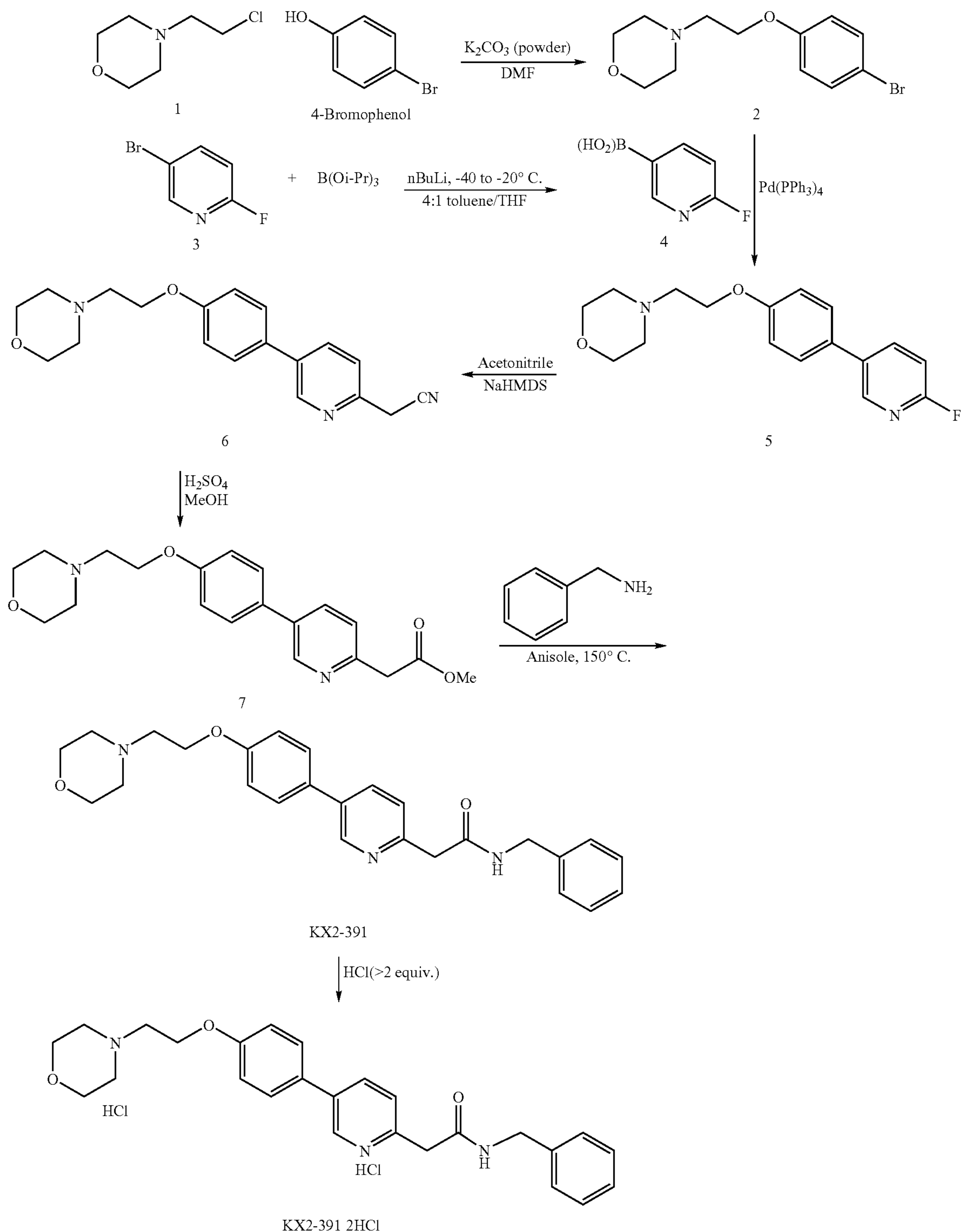
Scheme 2. Preparation of KX2-391•2HCl
