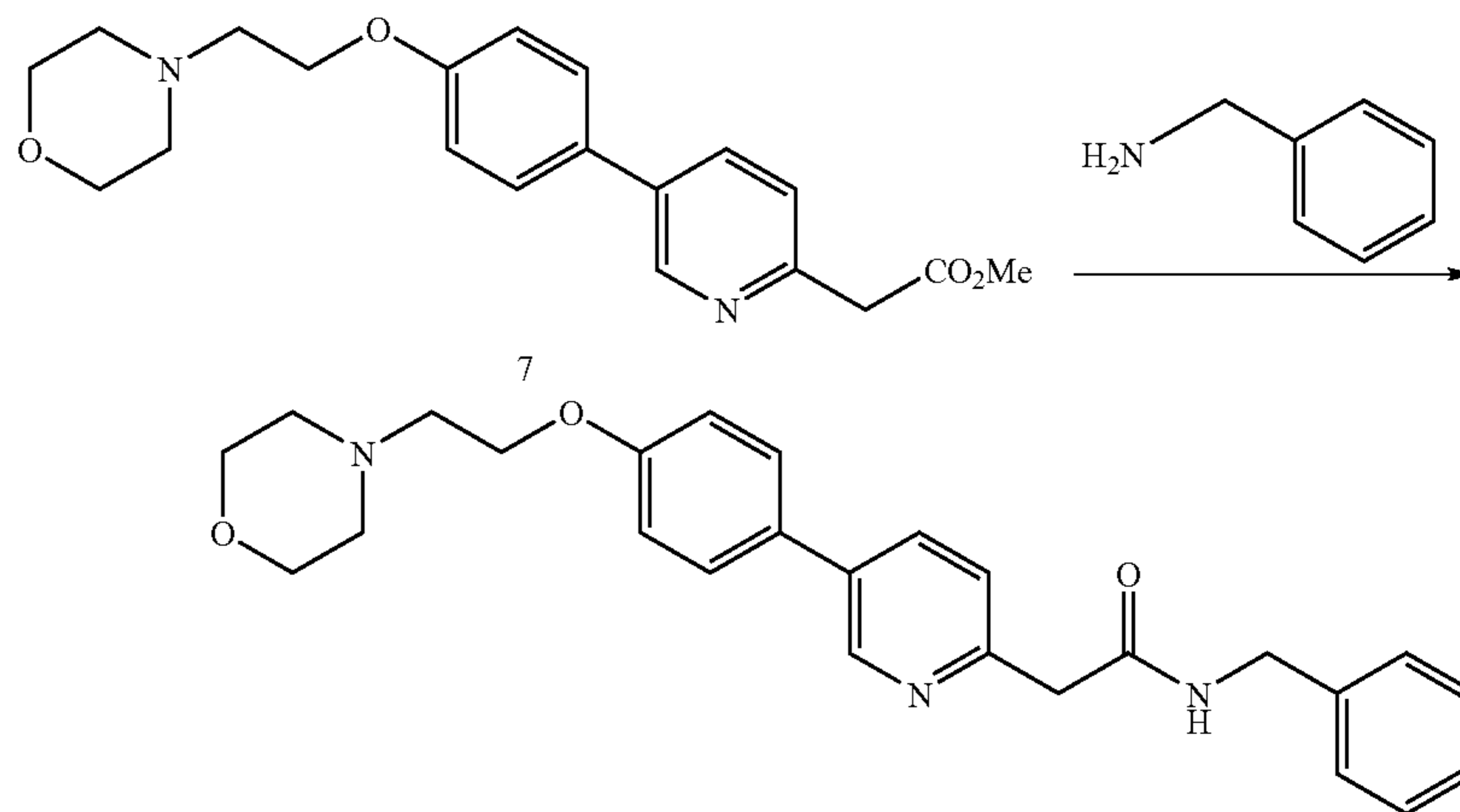
KX2-391 (free base)
