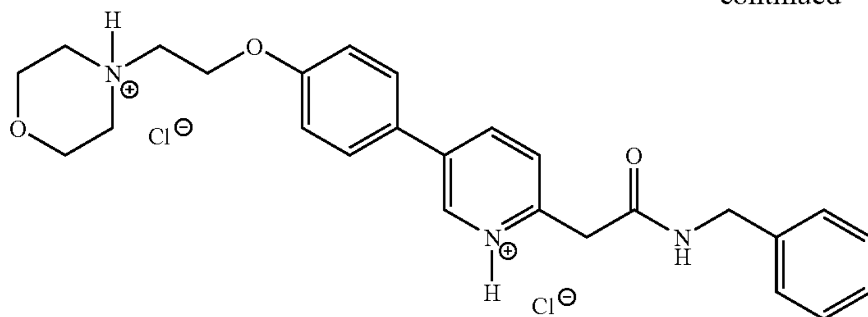
KX2-391 (diHCl salt)
