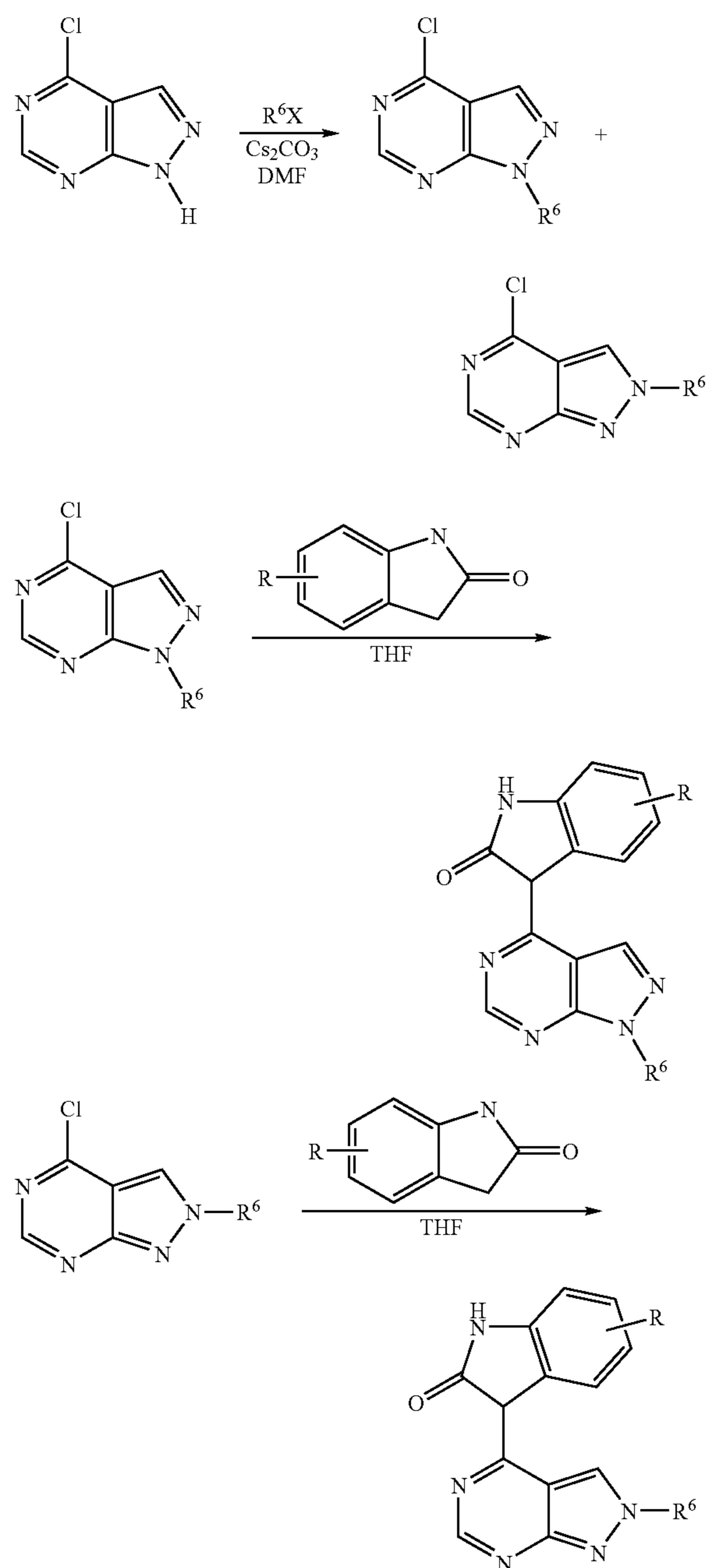
Scheme 2
