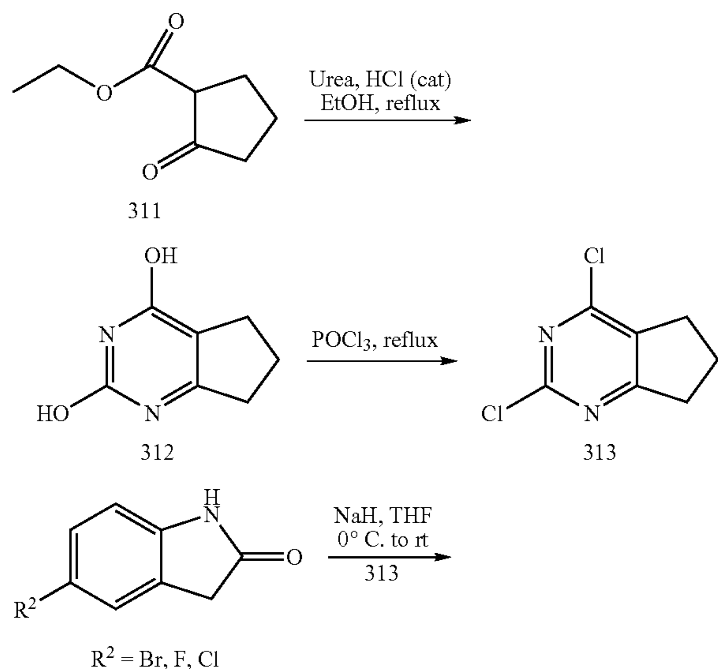
Scheme 7
