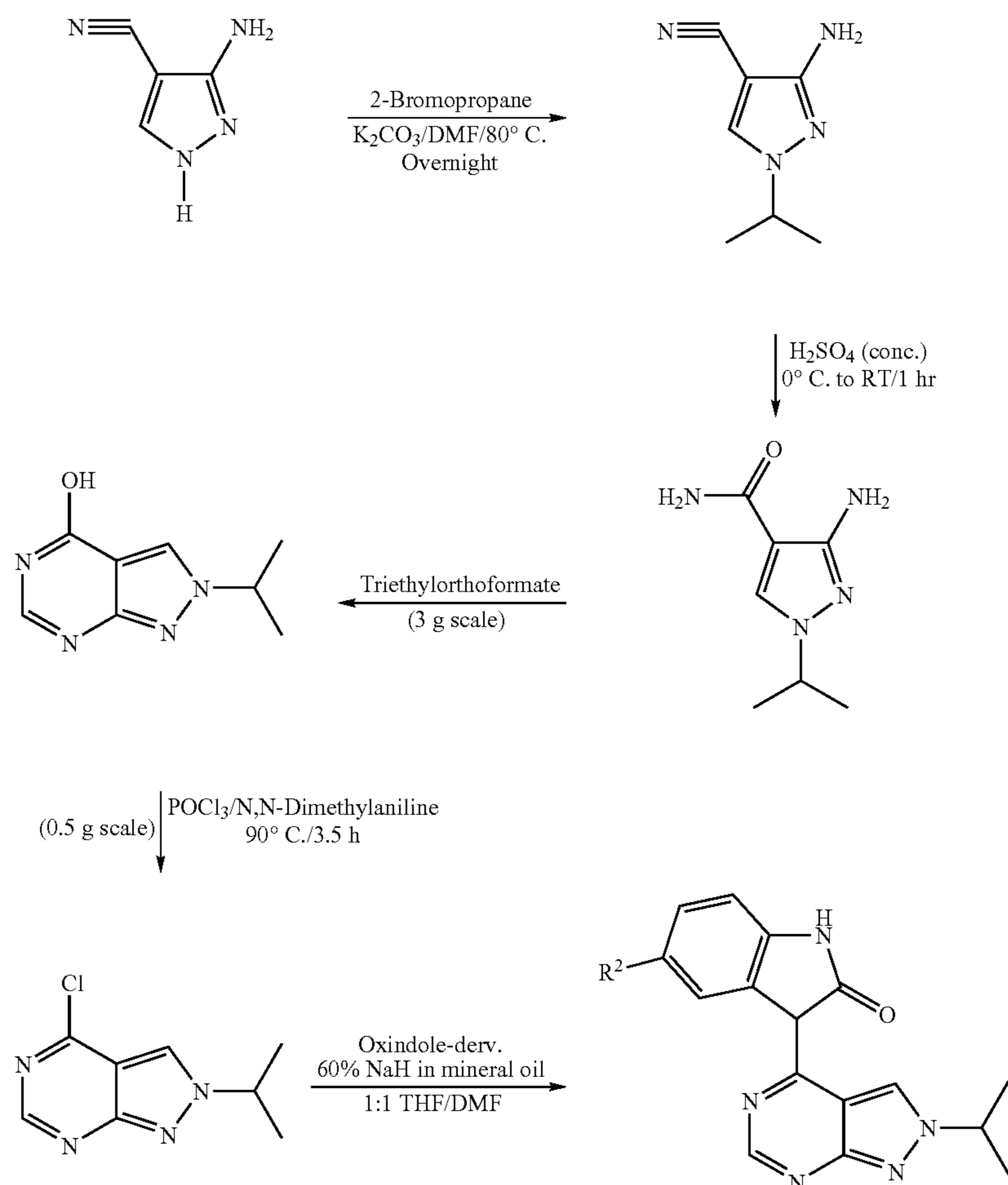
Scheme 9
