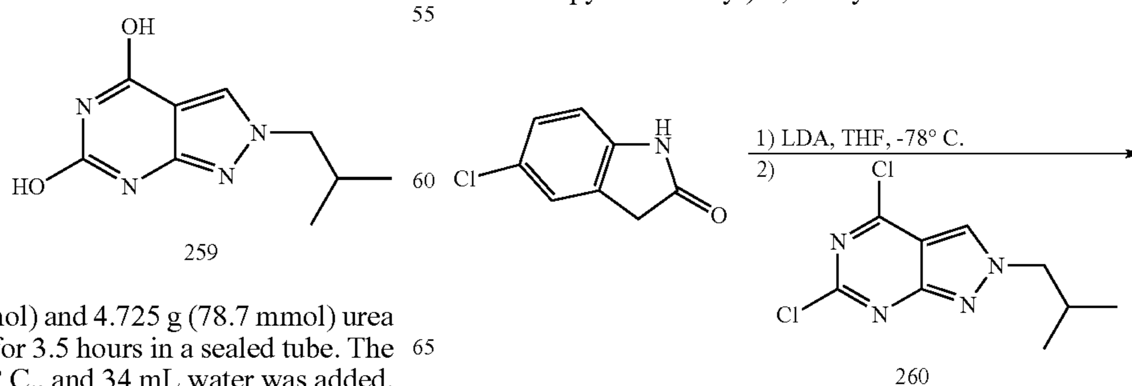
5-Chloro-3-(6-chloro-2-isobutyl-2H-pyrazolo[3,4-d]pyrimidin-4-yl)-1,3-dihydro-indol-2-one
