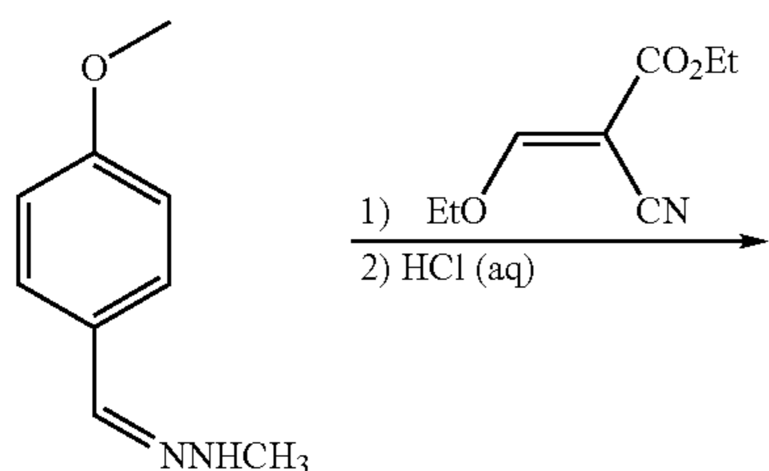
Scheme 6
