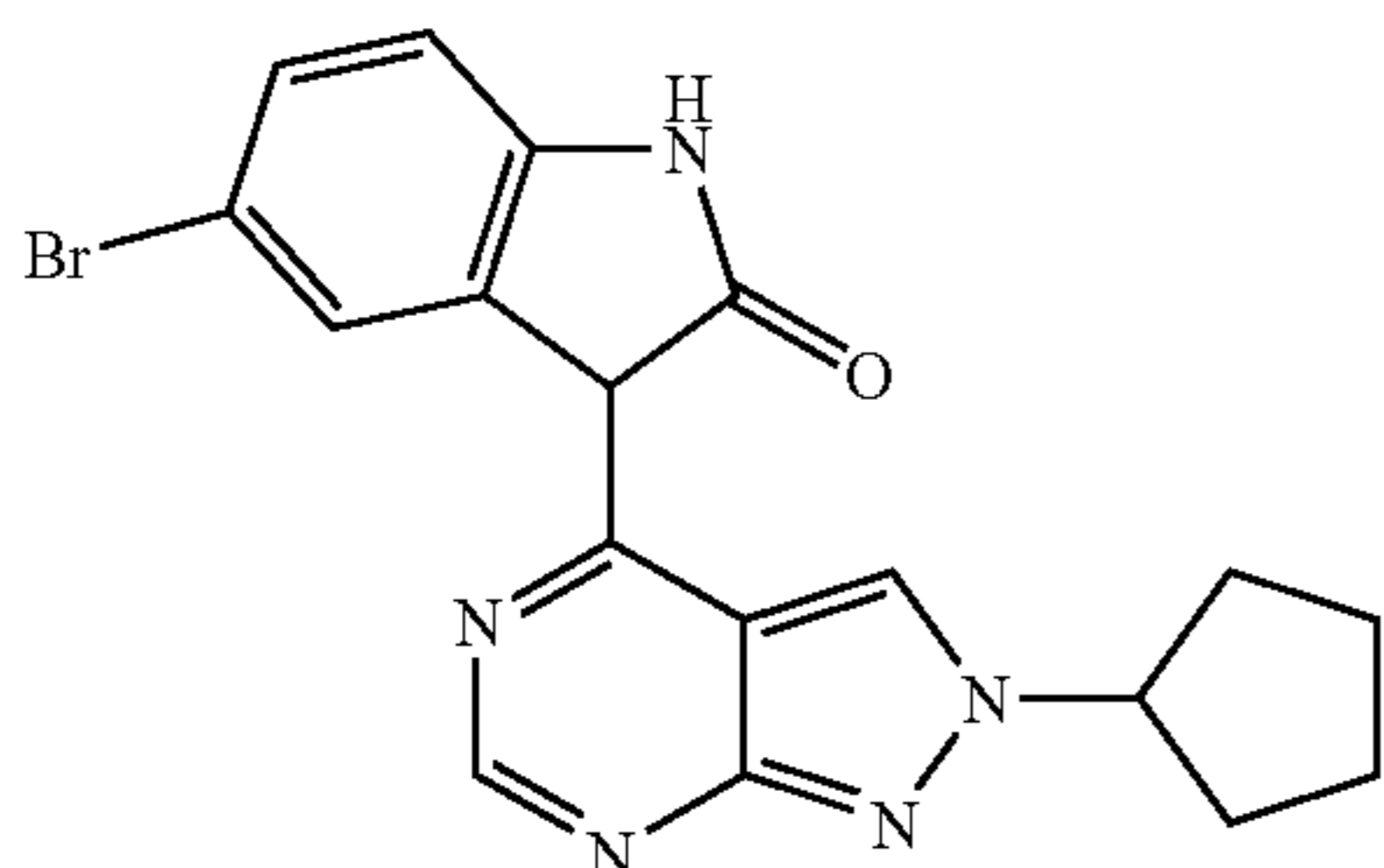
5-Bromo-3-(2-Cyclopentyl-2H-pyrazolo[3,4-d]pyrimidin-4-yl)-2-oxo-1,3-dihydro-indol-2-one
