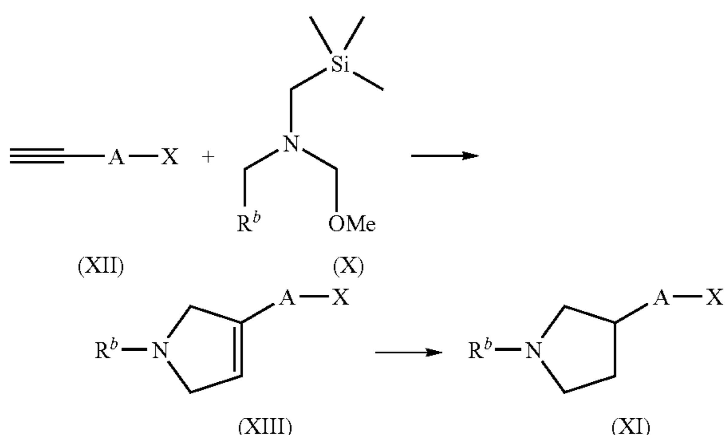
Scheme 4:
