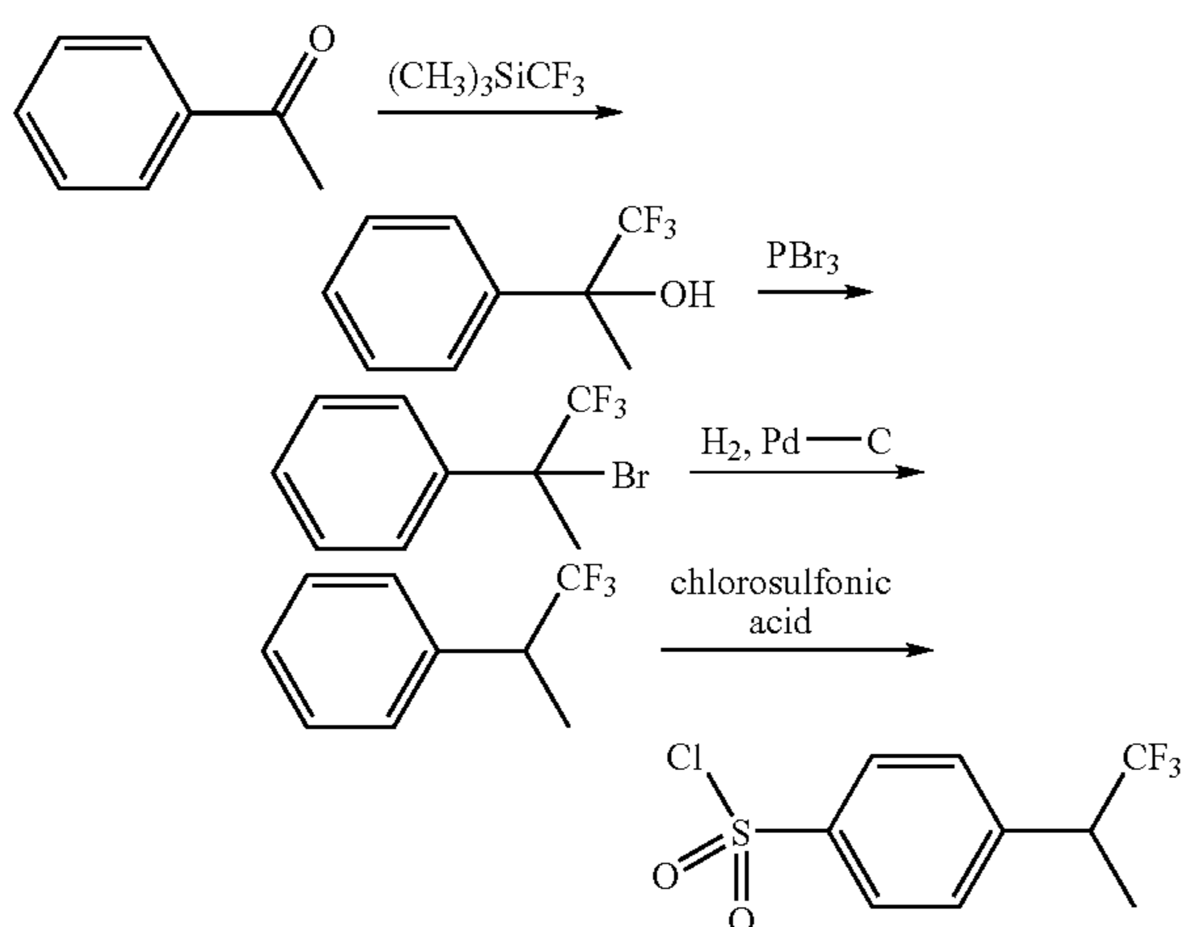
Scheme 8:
