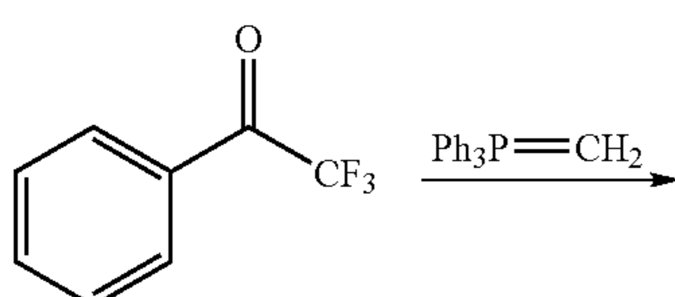
Scheme 7:
