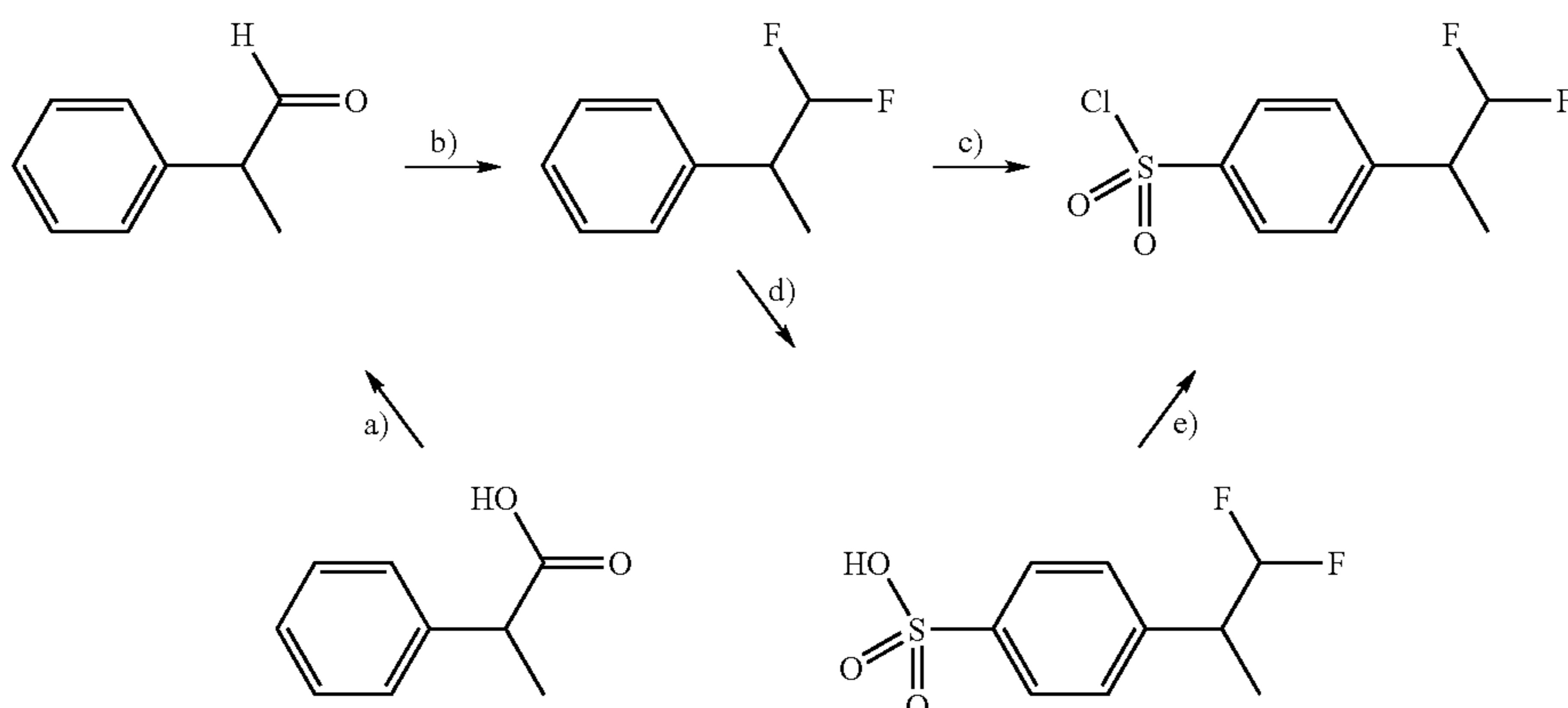
Scheme 6:
