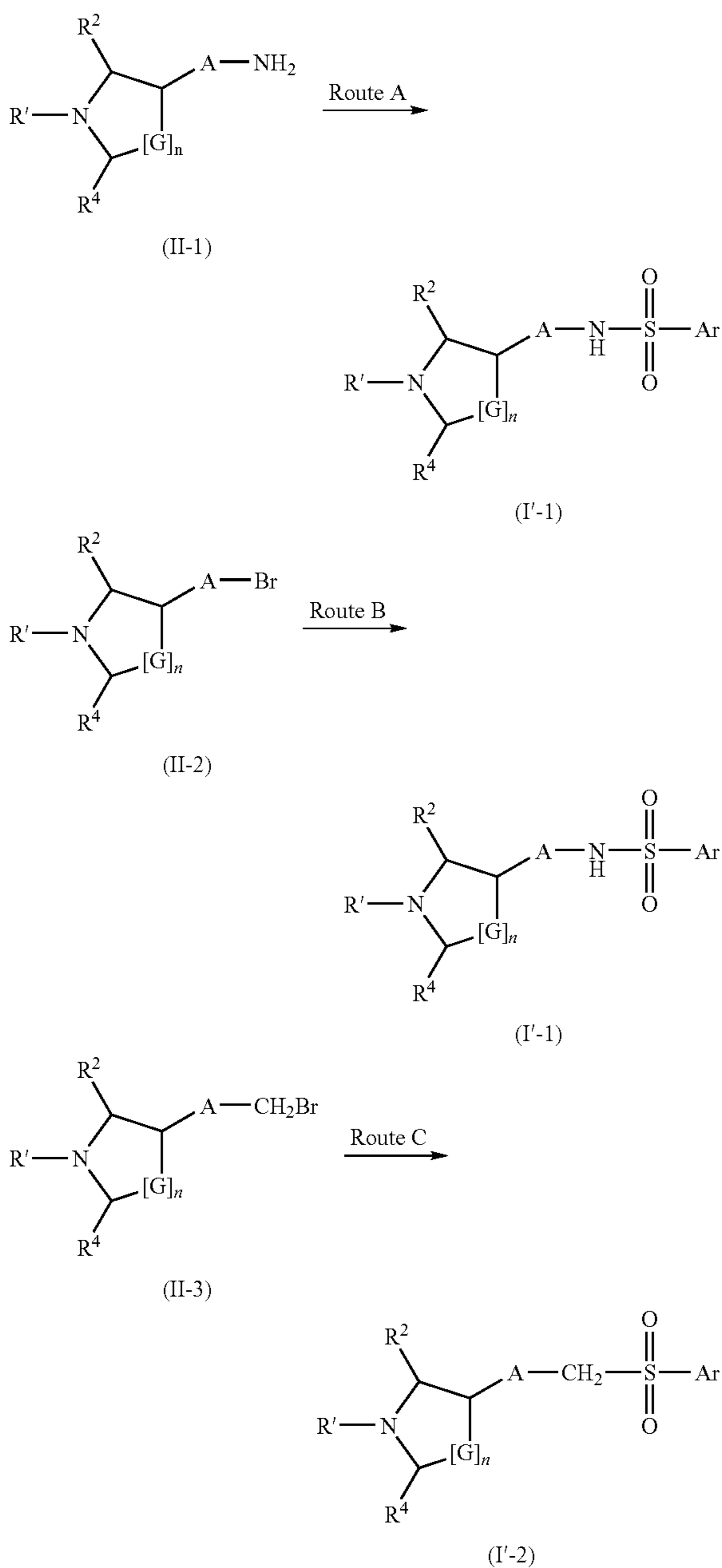
Scheme 1:
