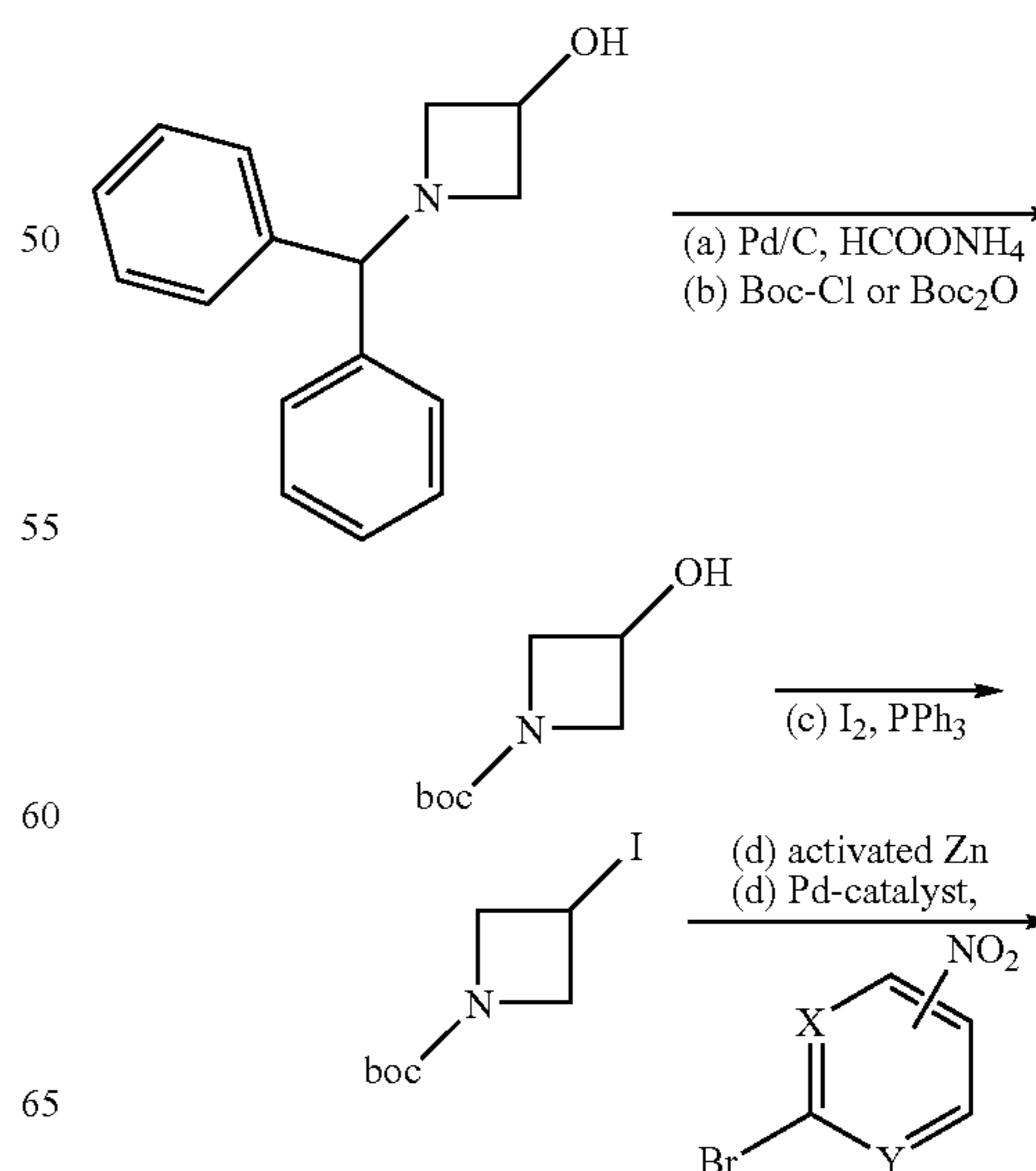
Scheme 5:
