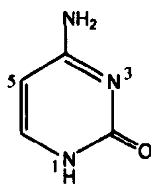
2-Oxy-4-amino pyrimidine or cytosine
