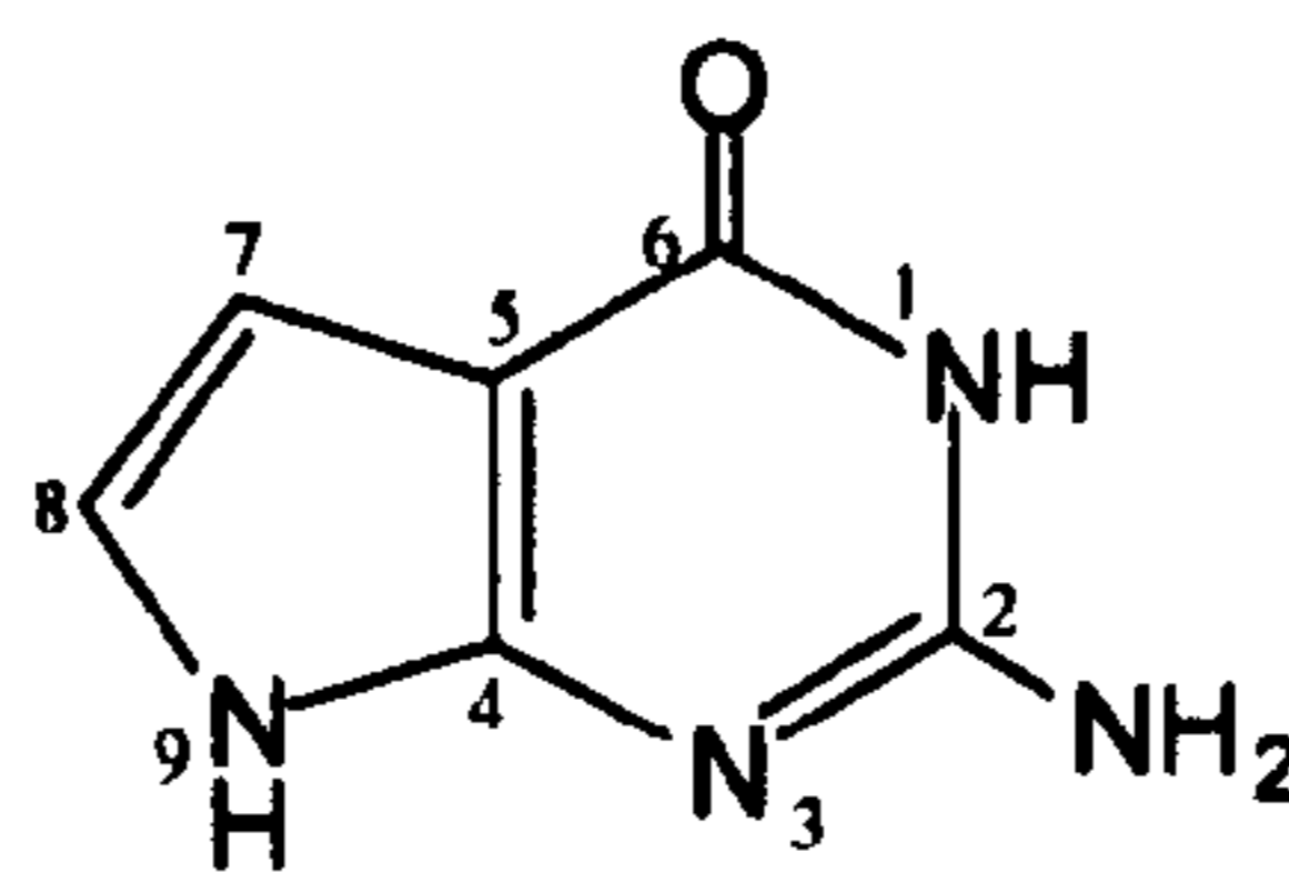
2-Amino-6-oxy-7-deaza-purine or 7-Deaza-guanine
