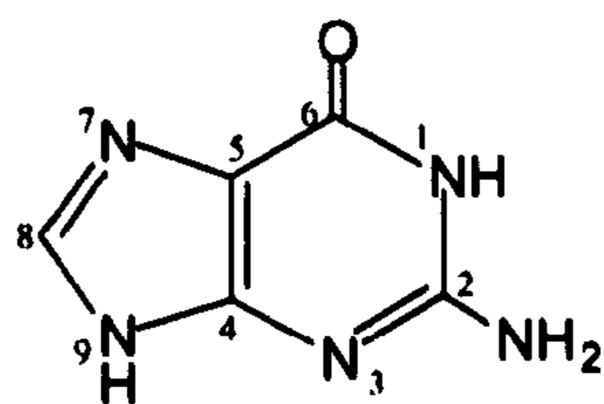
2-Amino-6-oxy-purine or Guanine
