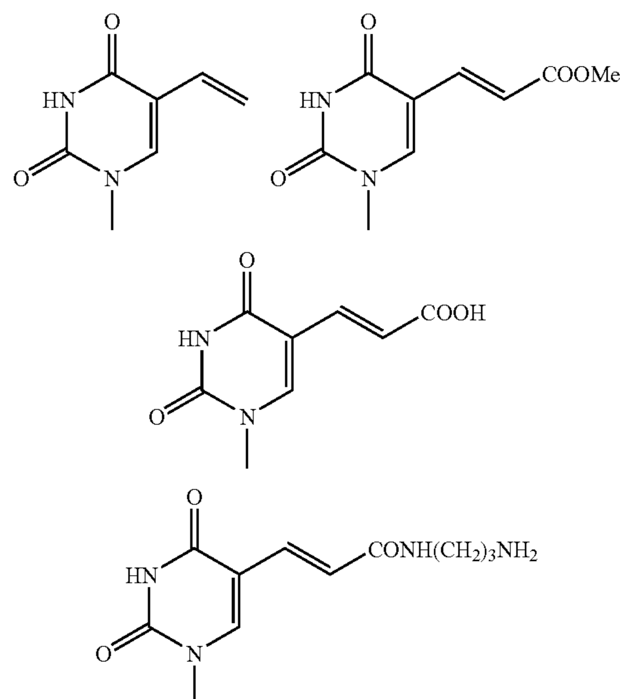
[Chemical Formula 11]
