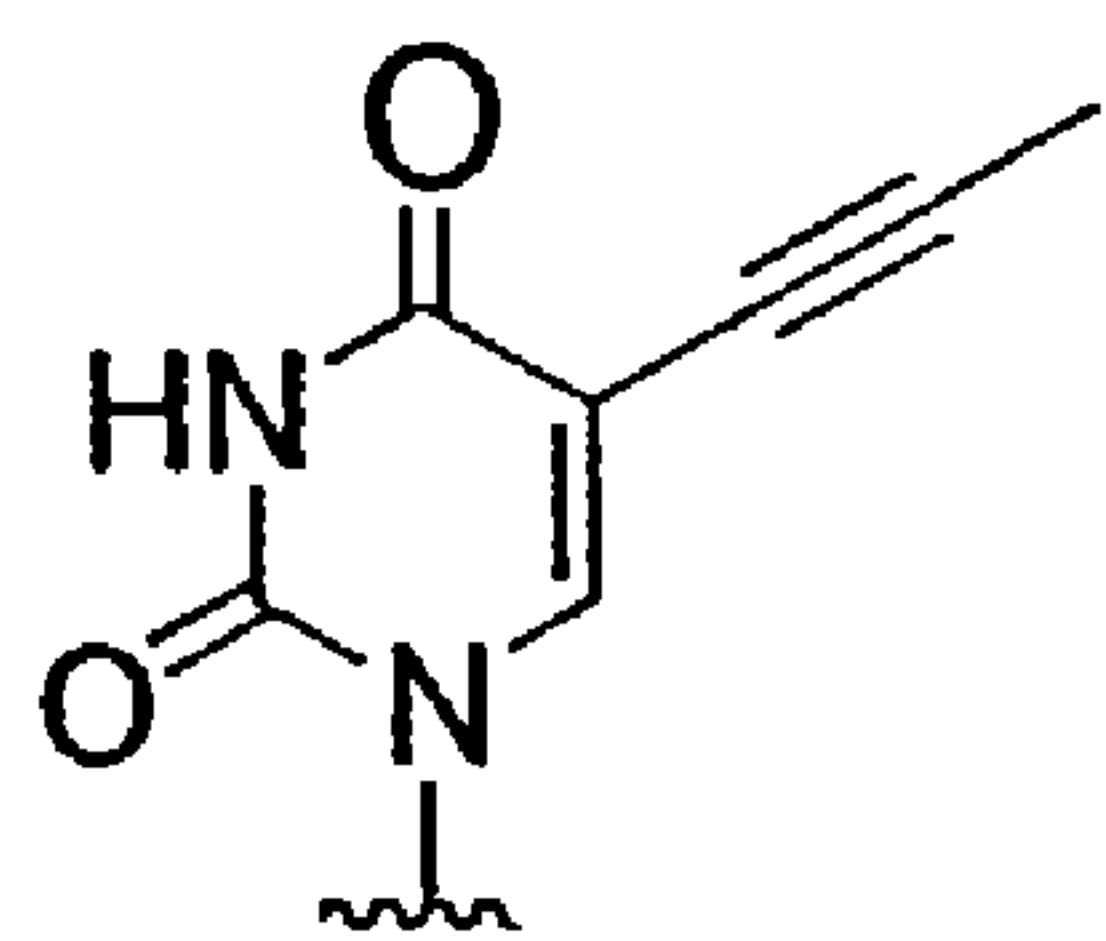
5-propynyl-U
