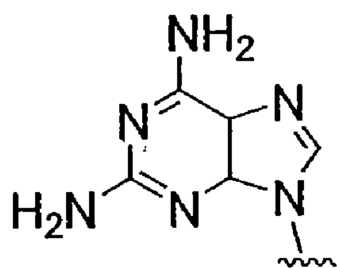
N9-(2,6,-diaminopurine)
