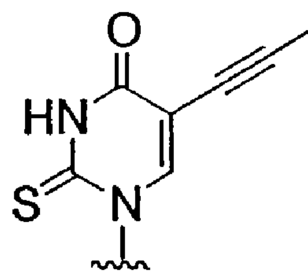
2-thio-5-propynyl-U
