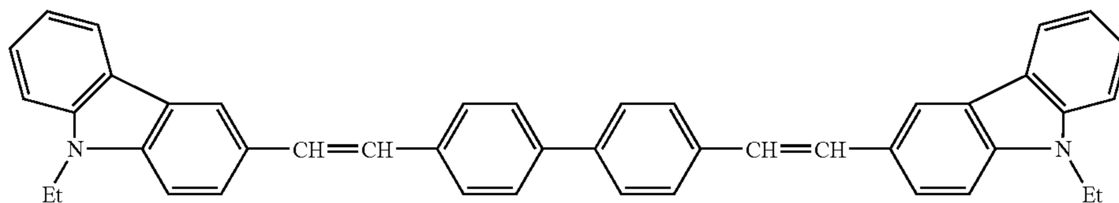
BCzVBi
