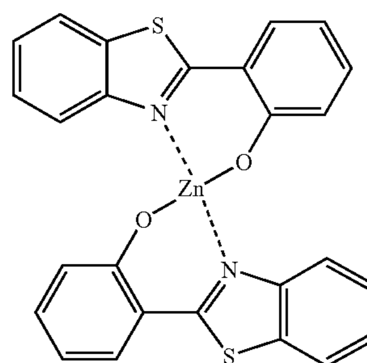
Zn(BTZ) 2
