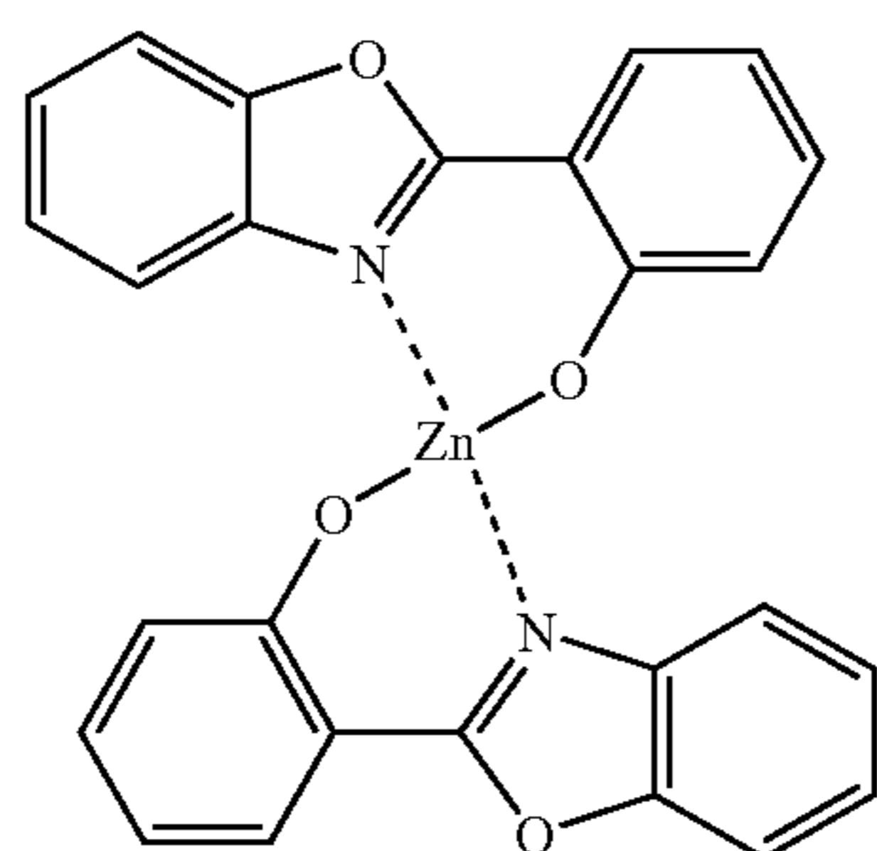
Zn(BOX) 1
