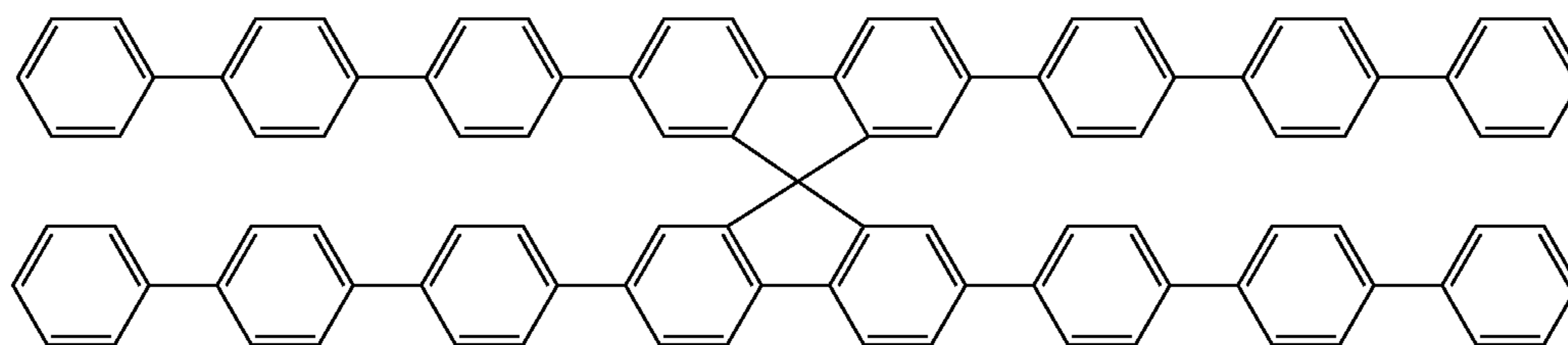
spiro-8Φ
